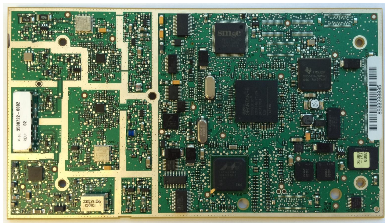
9211 Satellite Core Module Board – Topside
