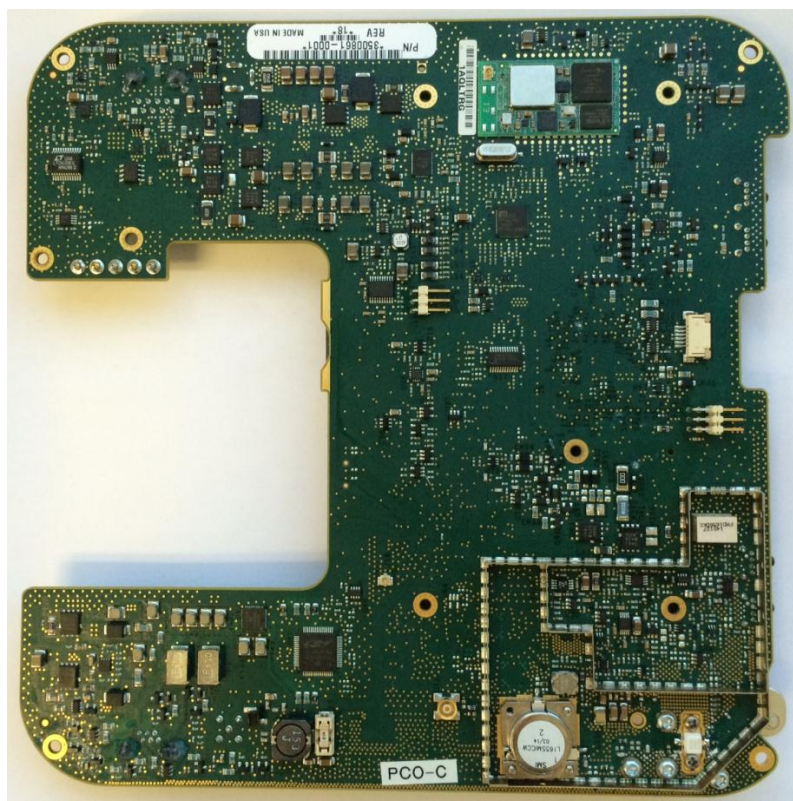
9211 Interface Board – Topside, no Shield
