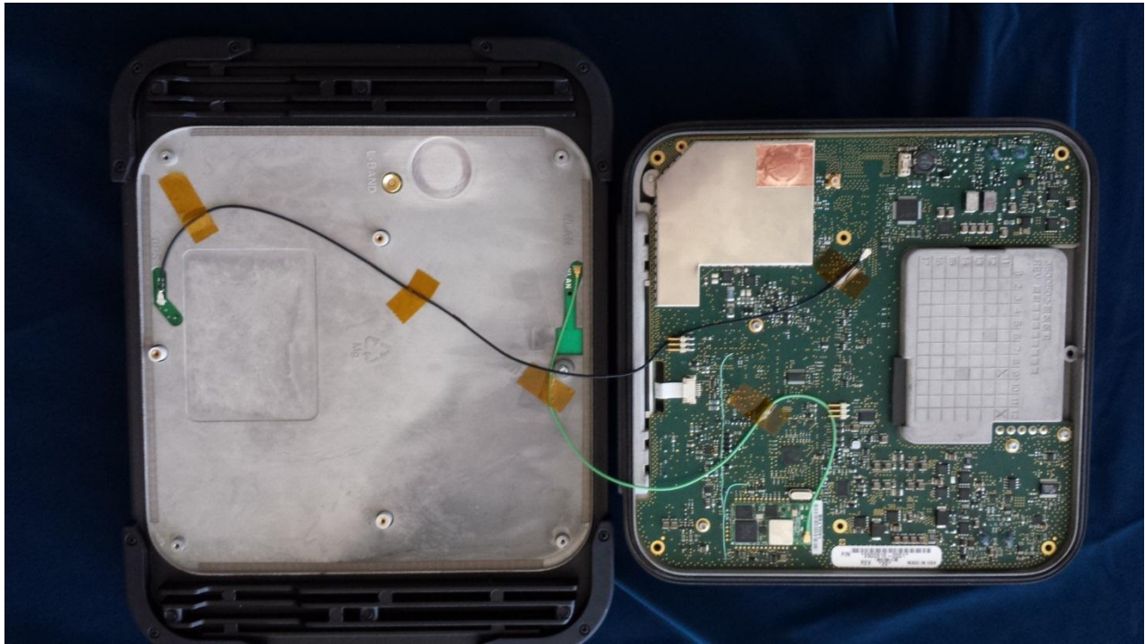
9211 Interface Board installed in chassis, Satellite Core Module underneath, With view of back of Antenna Radome
