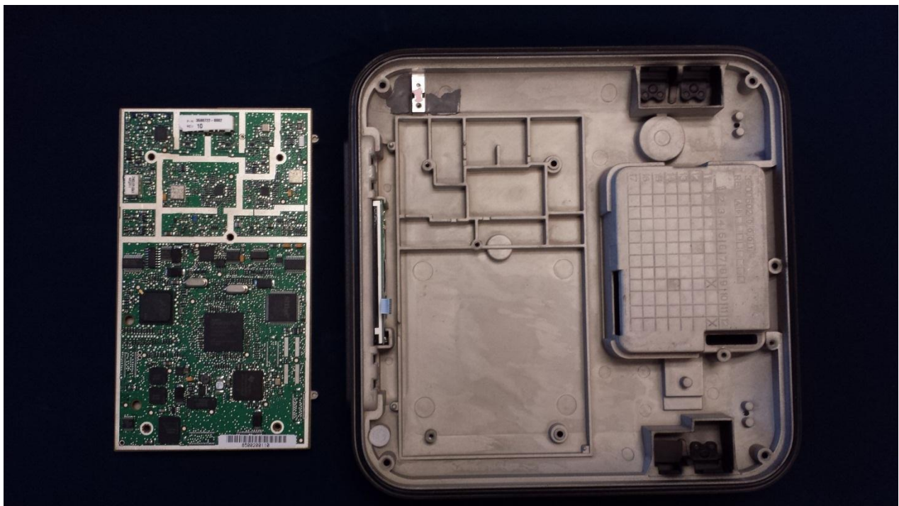
9211 Satellite Core Module board and view of chassis
