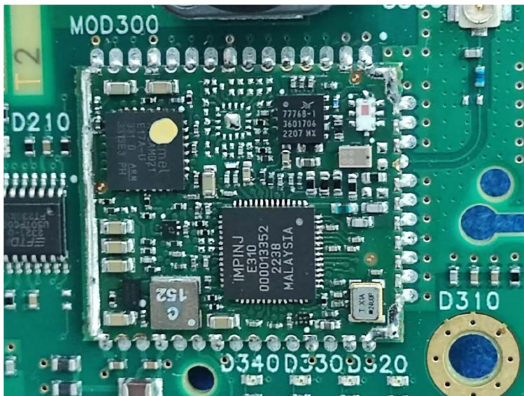
FIGURE 7 RF MODULE (MT-UHF-RFID01) SHIELDED REMOVED
