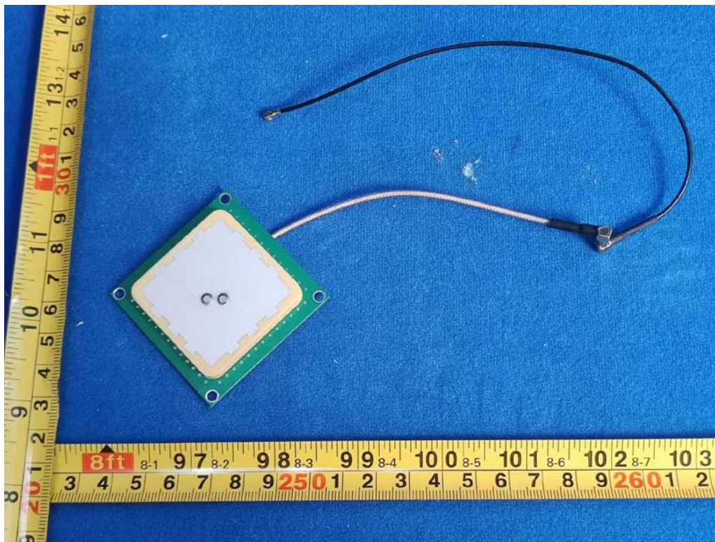
FIGURE 11 RF MODULE (MT-UHF-RFID01) ANTENNA#2 BACK
