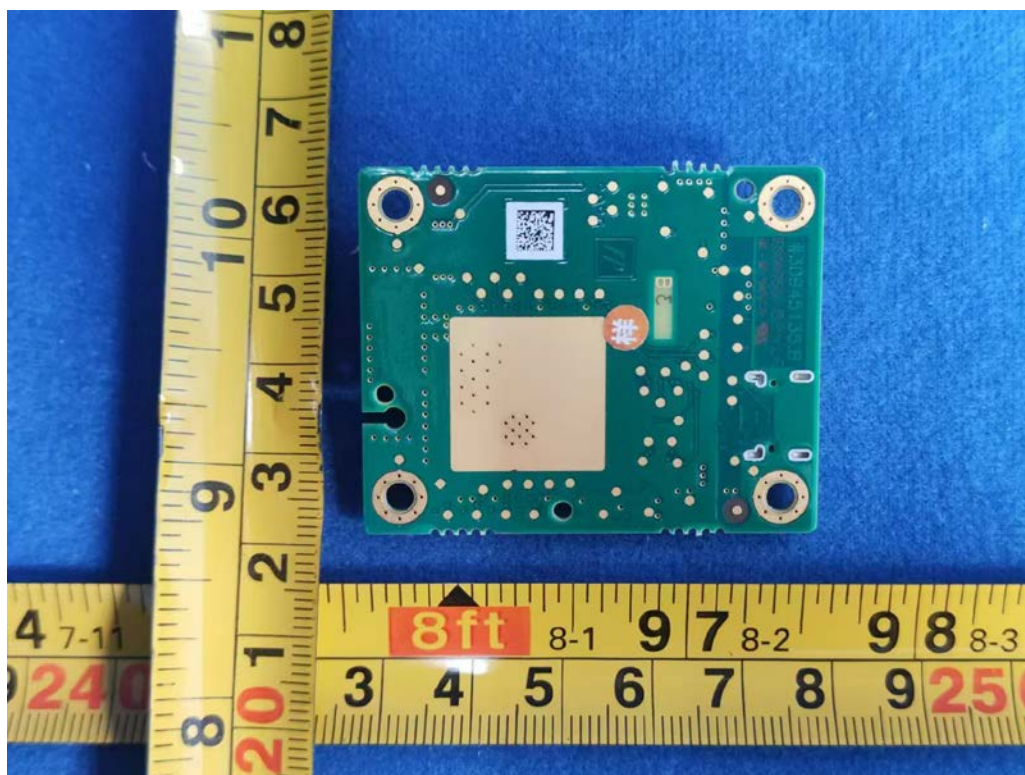
FIGURE 6 RF MODULE (MT-UHF-RFID01) MAIN BOARD BACK
