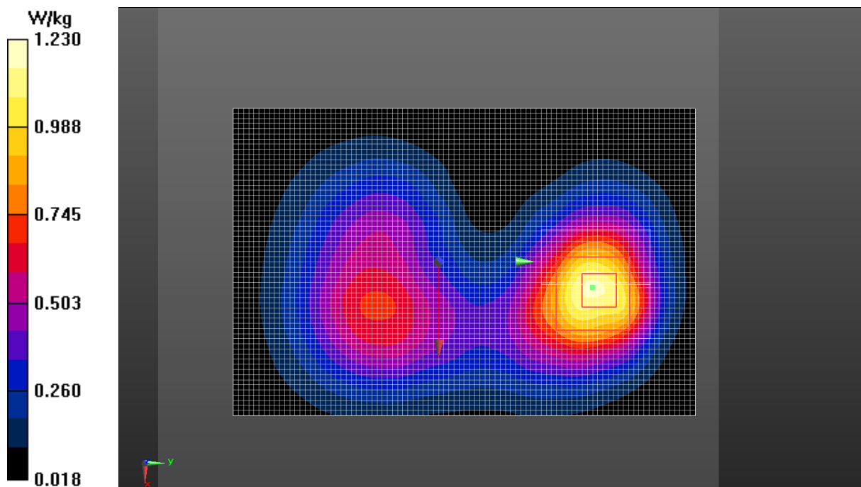
Fig.1 LTE Band 2
