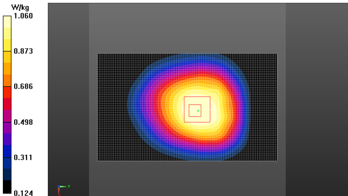
Fig.7 LTE Band 26
