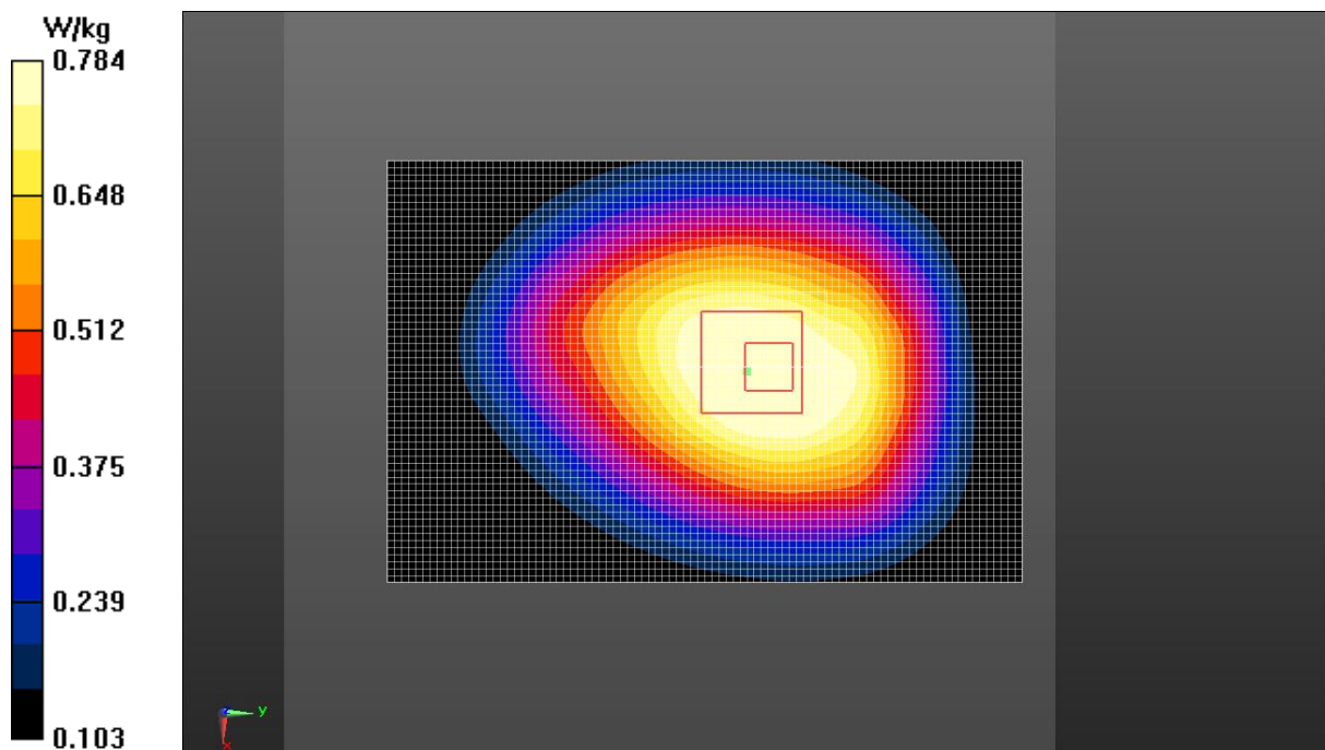
Fig.4 LTE Band 12
