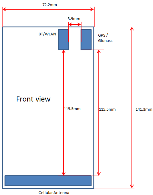
Photo 14: Antenna location
