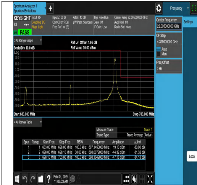
Band71_15MHz_QPSK_133397_1RB#74
