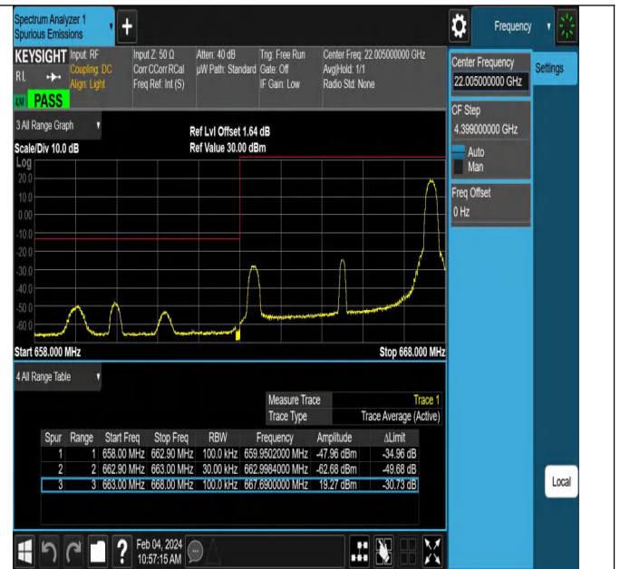
Band71_5MHz_QPSK_133147_1RB#24
