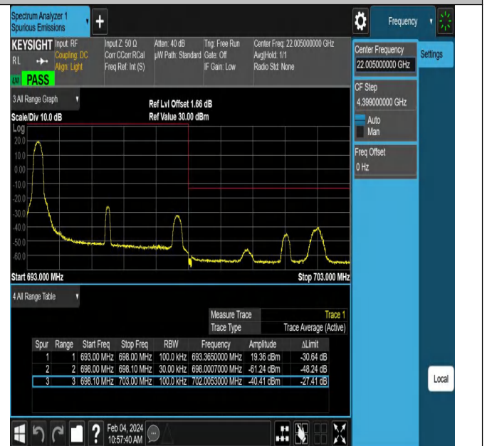
Band71_5MHz_QPSK_133447_1RB#0
