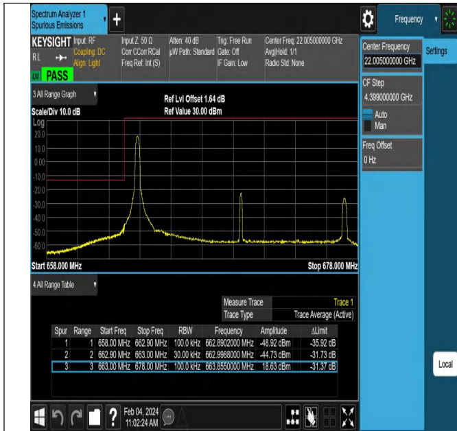
Band71_15MHz_QPSK_133197_1RB#0
