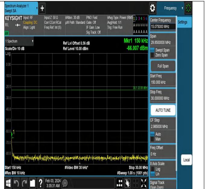
Band71_5MHz_QPSK_133147_1RB#0_0.15~30_0.15~30
