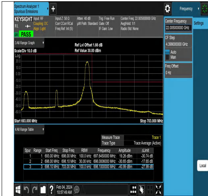
Band71_5MHz_QPSK_133447_1RB#24
