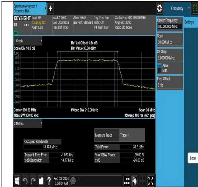
Band71-15MHz-QPSK-133297-75RB#0-PASS
