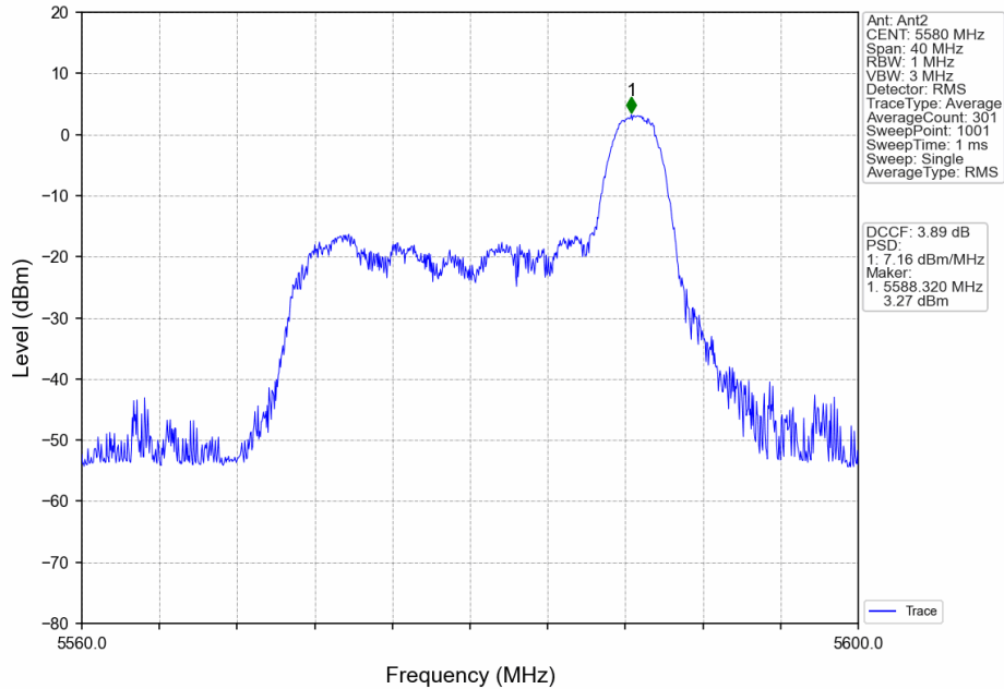
802.11ax(HEW20)_MCH_5580MHz_RU26_Right_MIMO_NTNV
