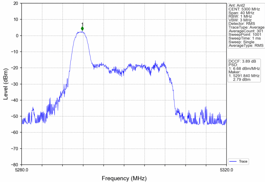
802.11ax(HEW20)_MCH_5300MHz_RU26_Left_MIMO_NTNV
