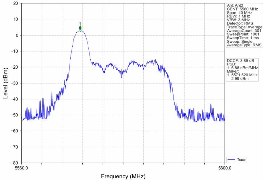
802.11ax(HEW20)_MCH_5580MHz_RU26_Left_MIMO_NTNV
