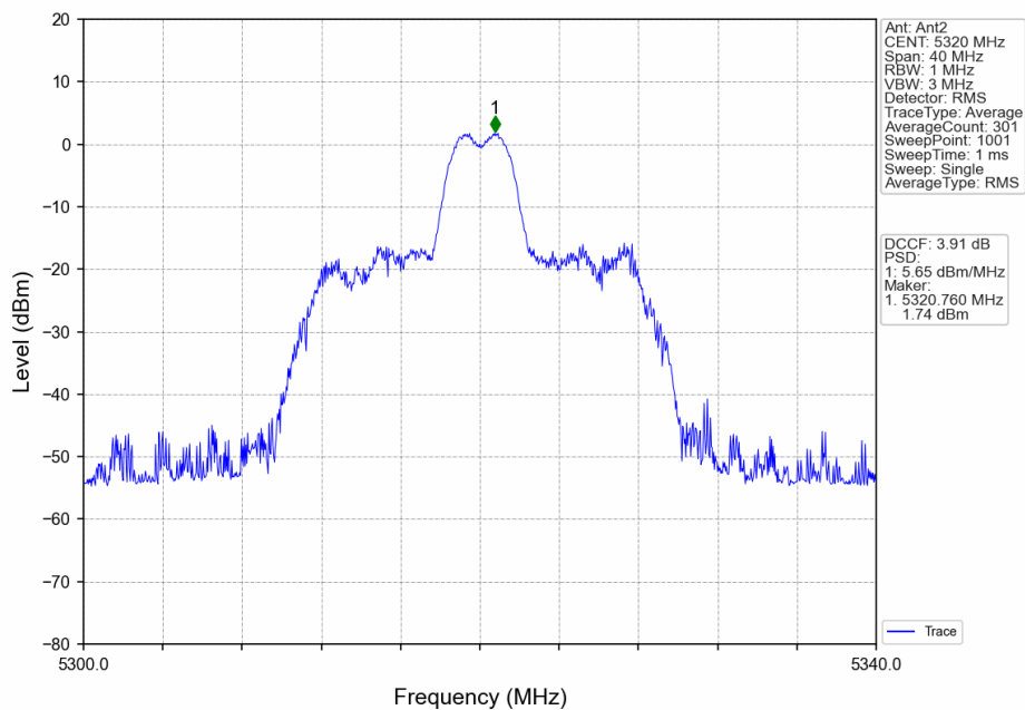
802.11ax(HEW20)_HCH_5320MHz_RU26_Mid_Ant2_NTNV
