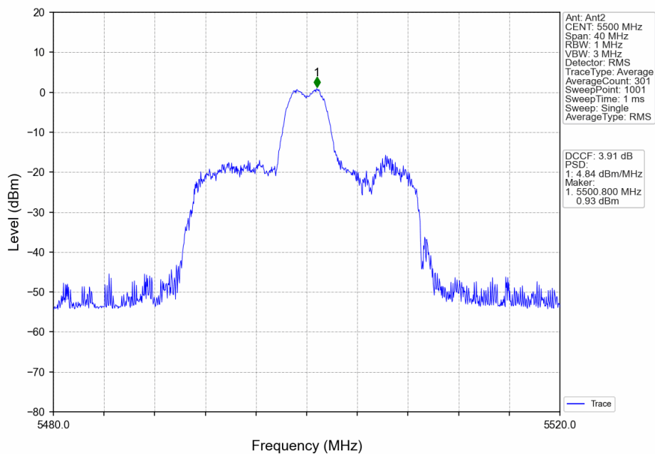
802.11ax(HEW20)_LCH_5500MHz_RU26_Mid_Ant2_NTNV
