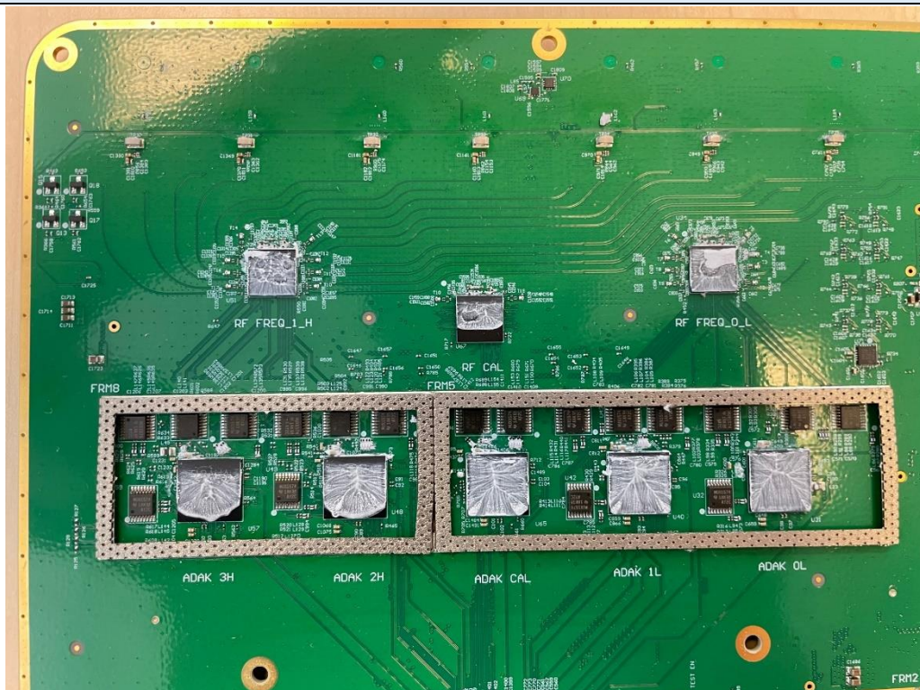
Internal View 8 (Bottom PCB Detail View_1)
