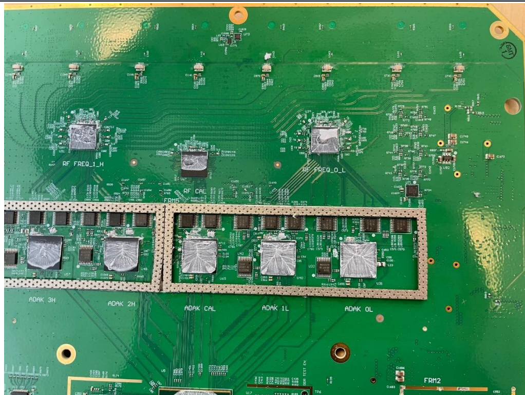
Internal View 10 (Bottom PCB Detail Veiw_3)
