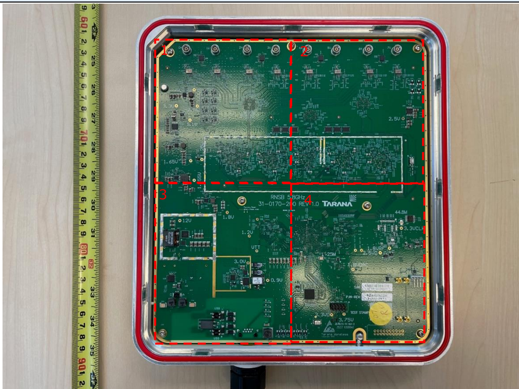
Internal View 2 (Front PCB View)
