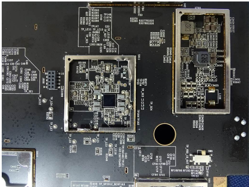
(79) EUT Photo
