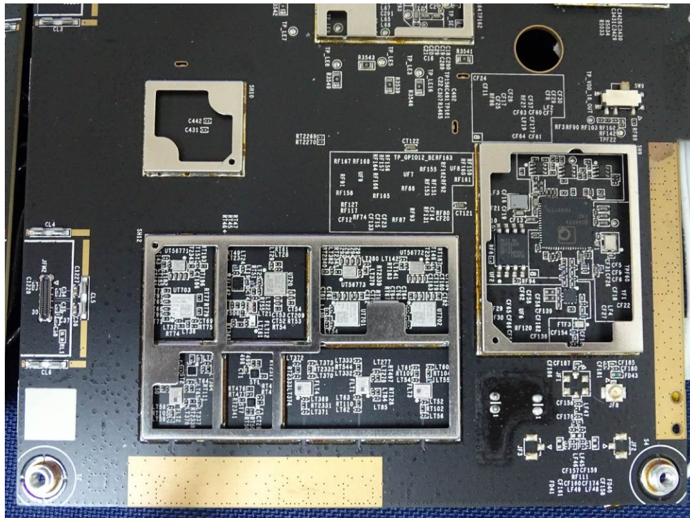
(80) EUT Photo
