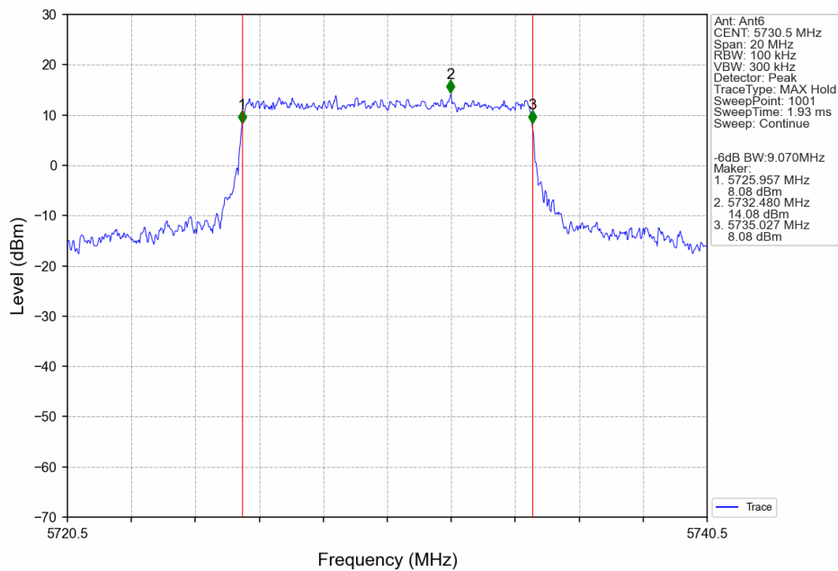
10M_LCH_5730.5MHz_Ant6_NTNV
