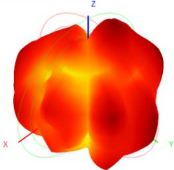
2450.0MHz H+V, Eff: 41.5%
