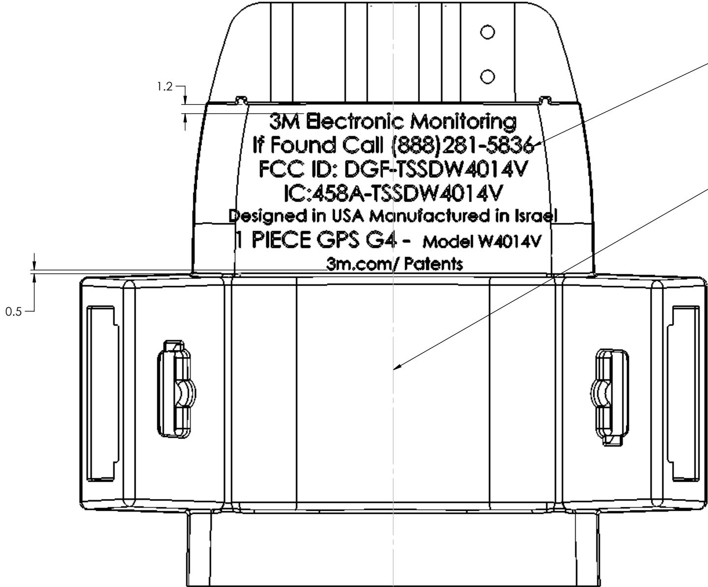
REAR/ BACK VIEW
