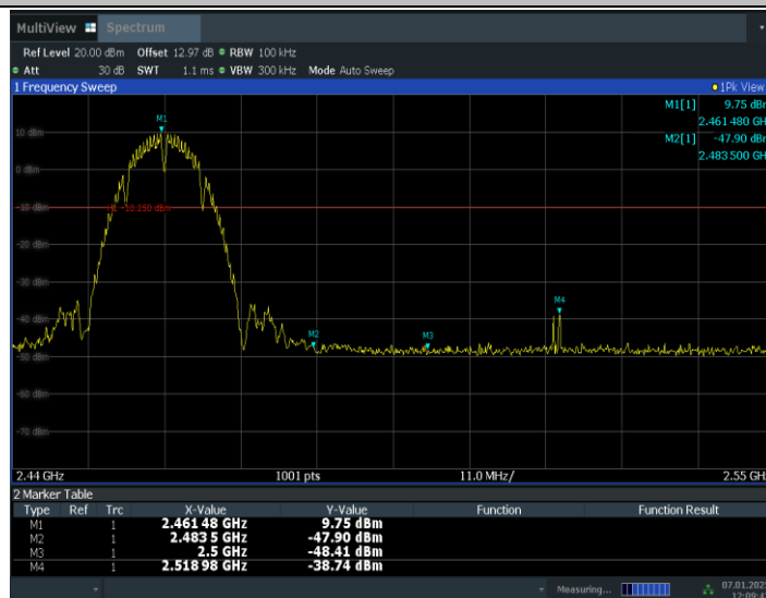
11B_Ant1_High_2462
