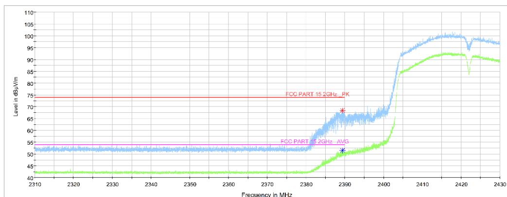
Fig.A.6.2.7 Transmitter Spurious Emission - Radiated (Power): 802.11n-HT40, ch3, 2.31 GHz - 2.43GHz
