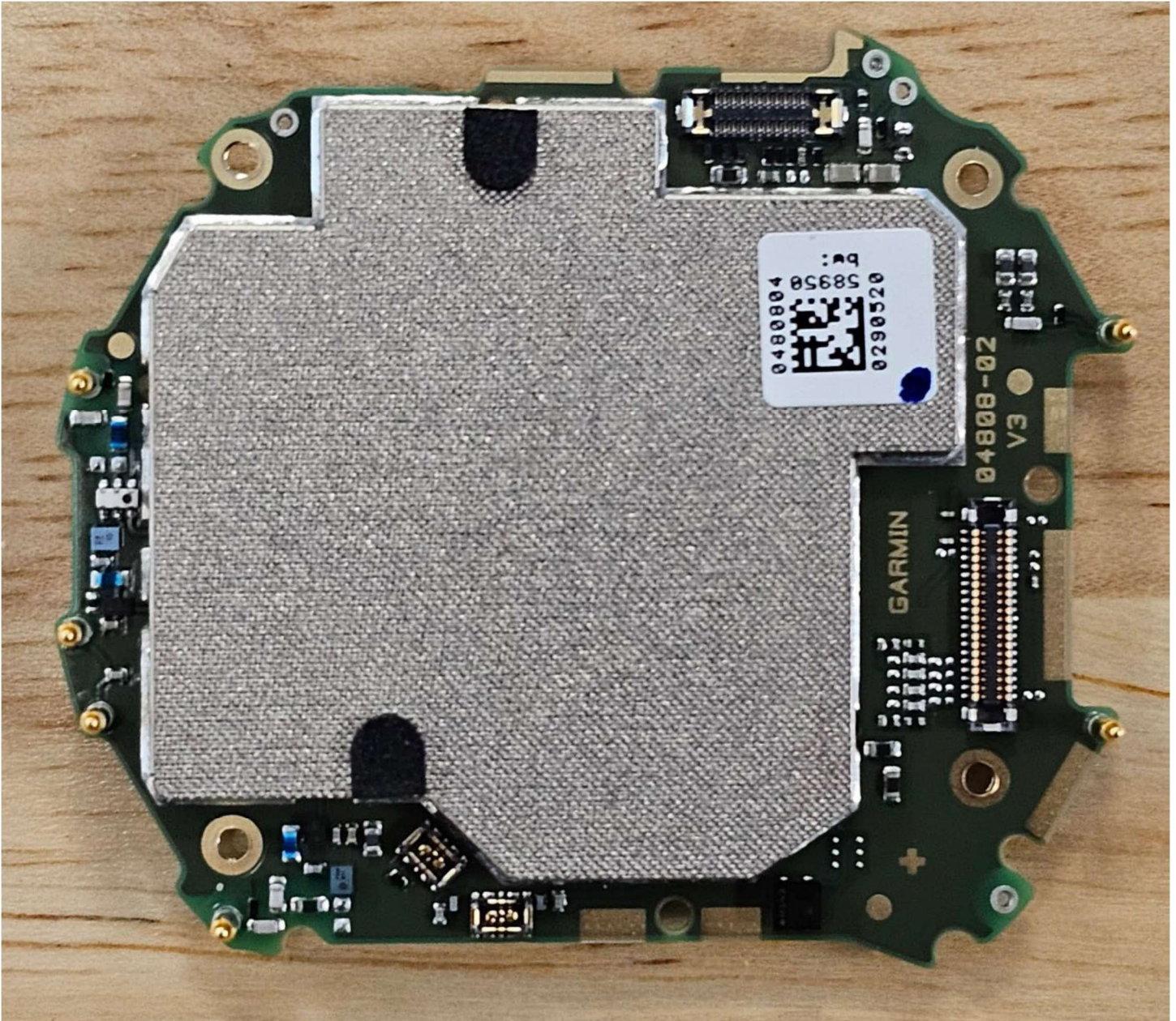
Figure E14.3 – Internal – DUT Split, Main PCB
