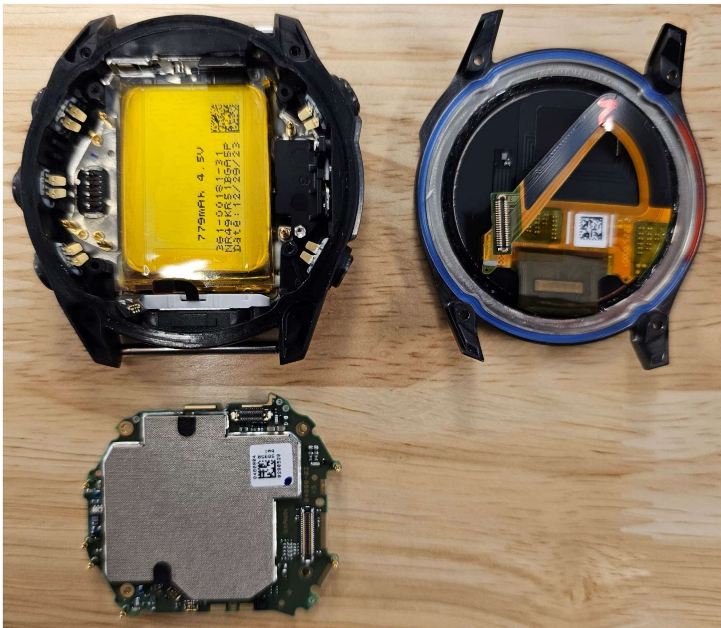
Figure E14.2 – Internal – DUT Split, Main PCB Removed
