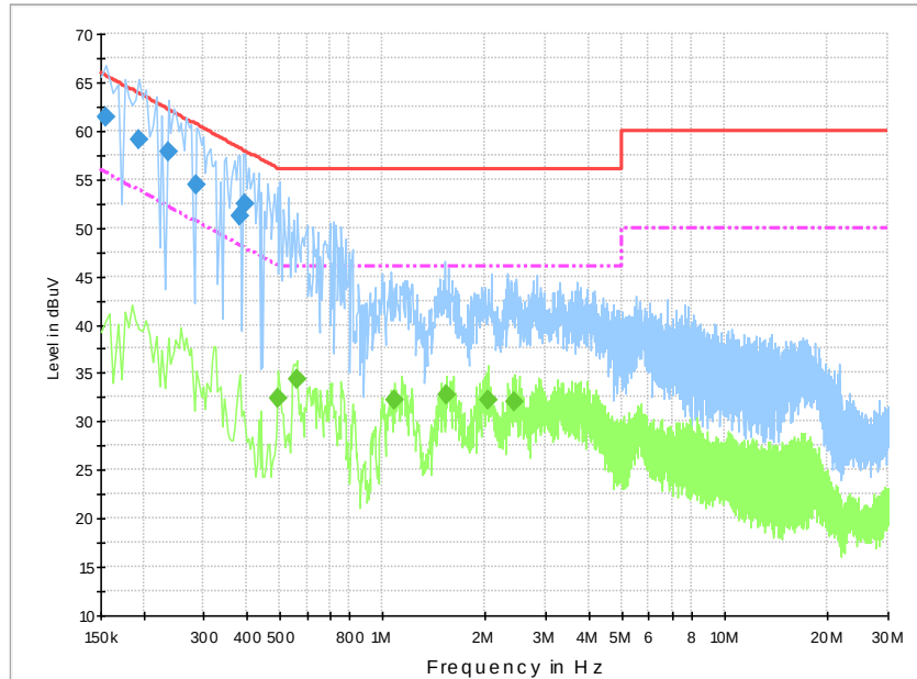
Fig.B.11.1 AC Powerline Conducted Emission- bluetooth
