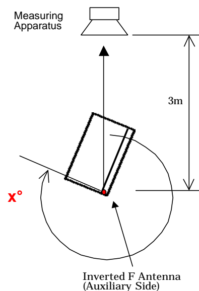
Auxiliary Antenna
