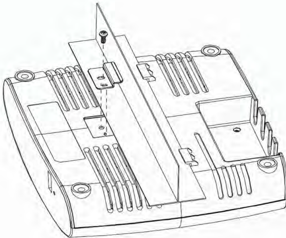
Figure 3-2 Wall Mounting
