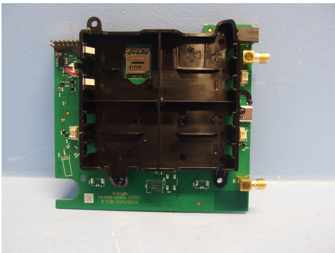
Enclosure removed
