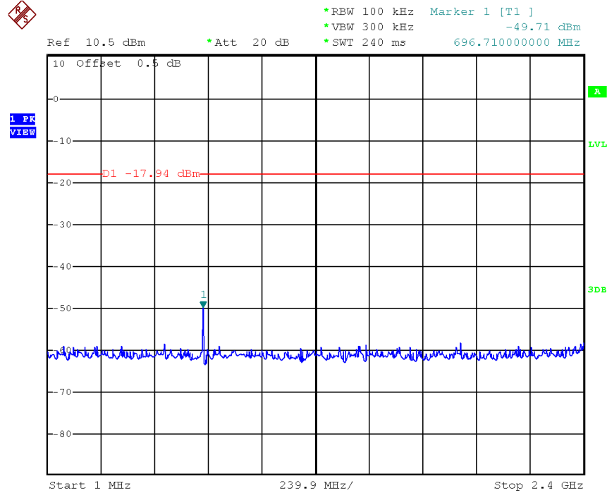
802.11b, Middle Channel, Plot A
