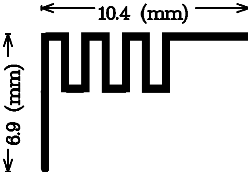
Antenna Photo & Length (mm)
