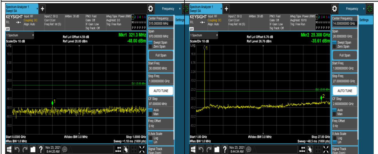
Band38-20MHz-QPSK-38150-1RB#0-Range1:30~1000MHz
