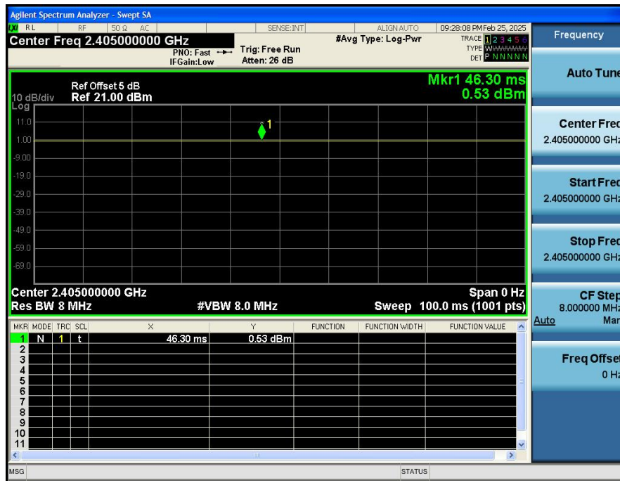
Duty_Cycle_NVNT_ANT1_2Mbps_2405
