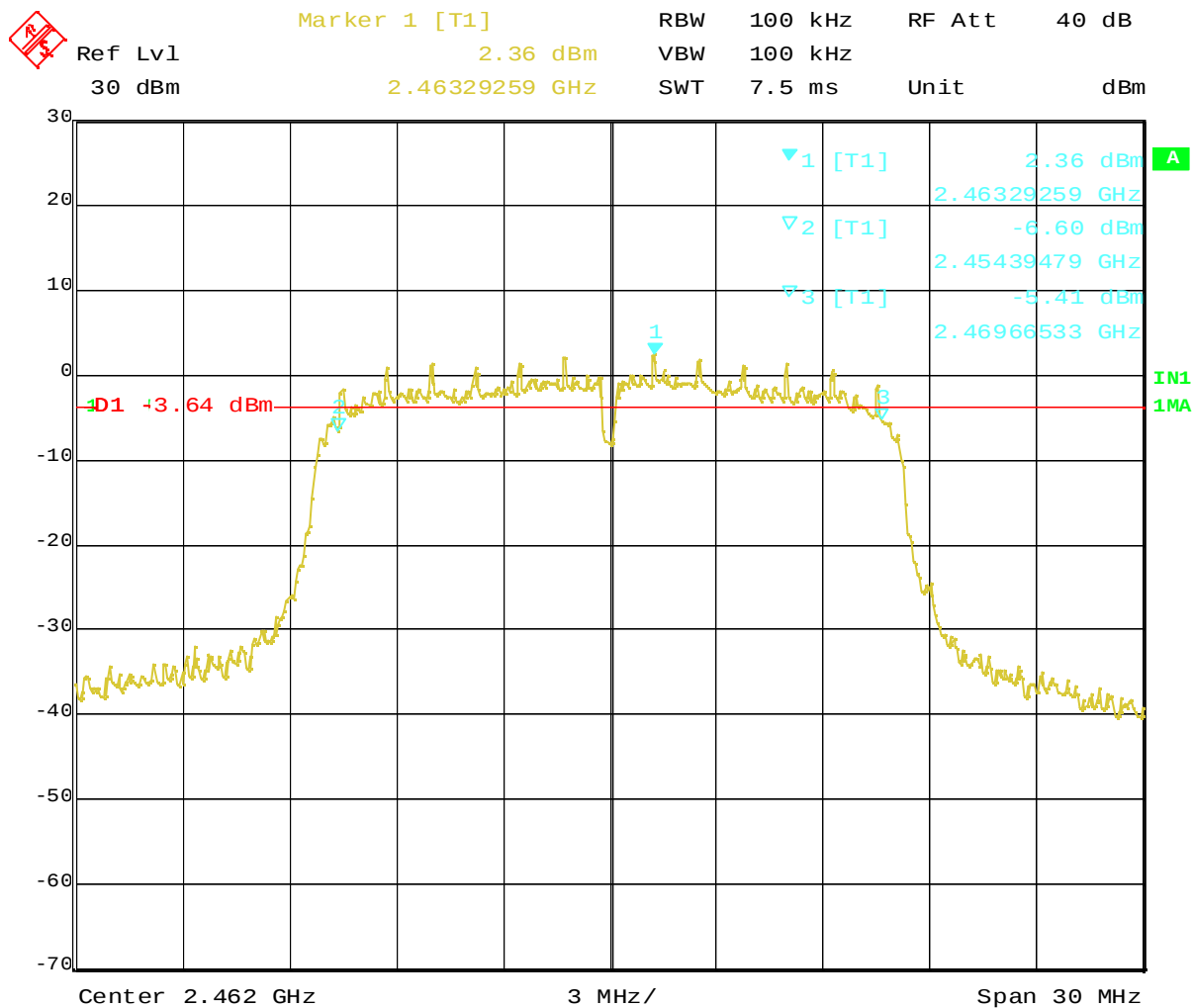
Plot 1-2. 6dB BW at 2462MHz (OFDM, 6Mbps)
