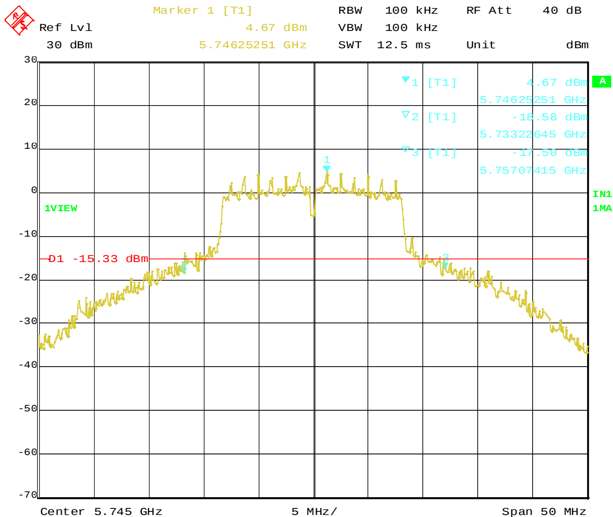
Plot 2-5. 20dB BW at 5745MHz (OFDM, 6Mbps)
