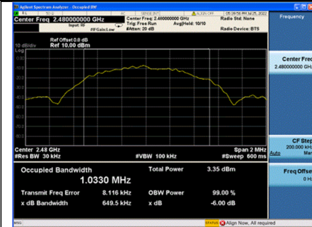
Test Mode:GFSK (LE 1Mbps) 2480MHz
