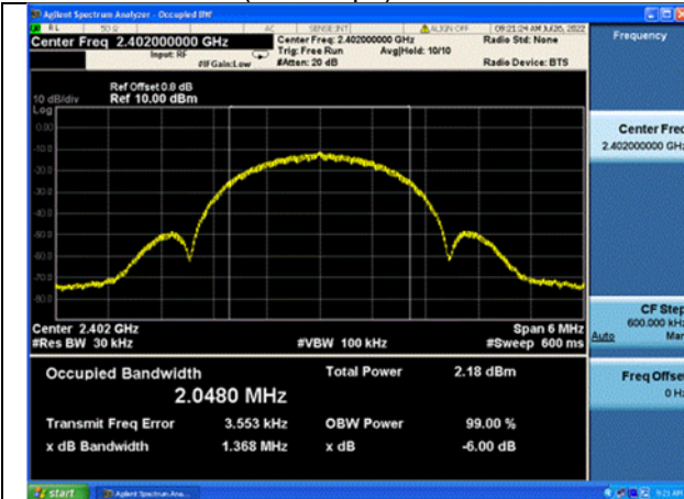
Test Mode:GFSK (LE 2Mbps) 2402MHz
