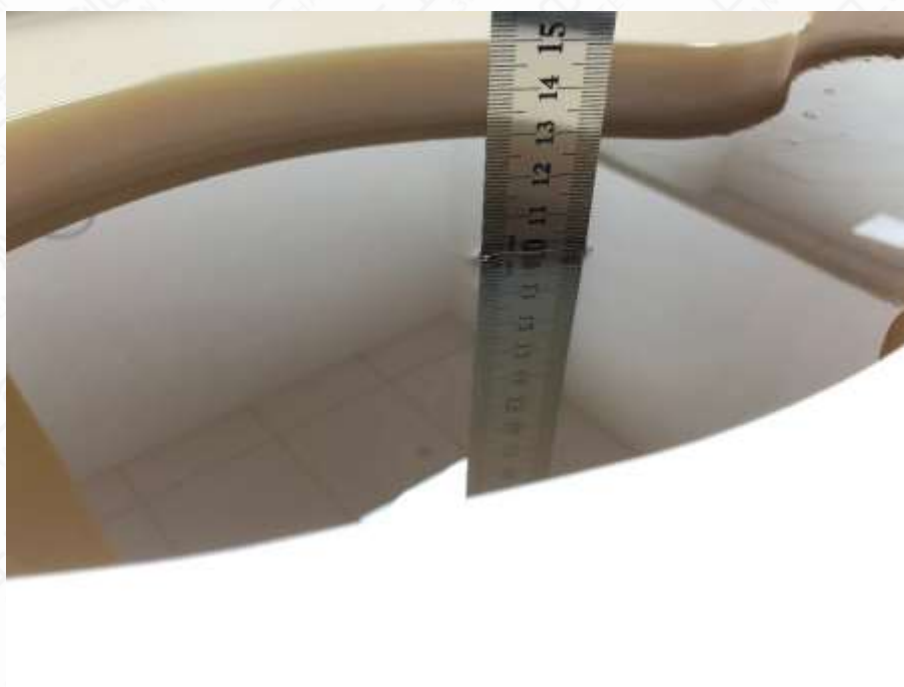
Picture 9.2-2 Liquid depth in the Flat Phantom for SAR measurements > 3 \text{ GHz}
