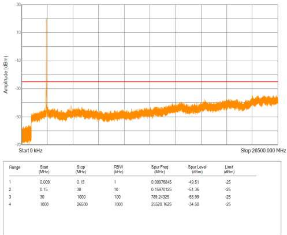
Band41(2555-2655) QAM16 BW=10MHz Channel=40290 RB Size=50 Position=#0
