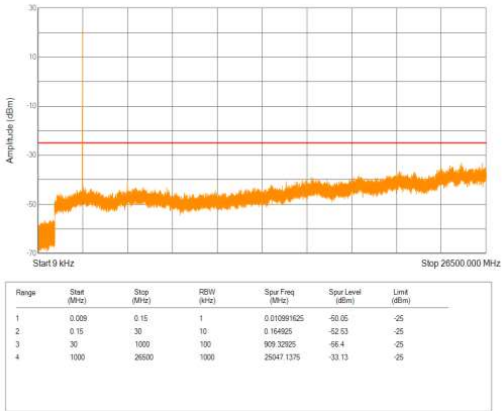
Band41(2555-2655) QAM16 BW=5MHz Channel=41215 RB Size=25 Position=#0
