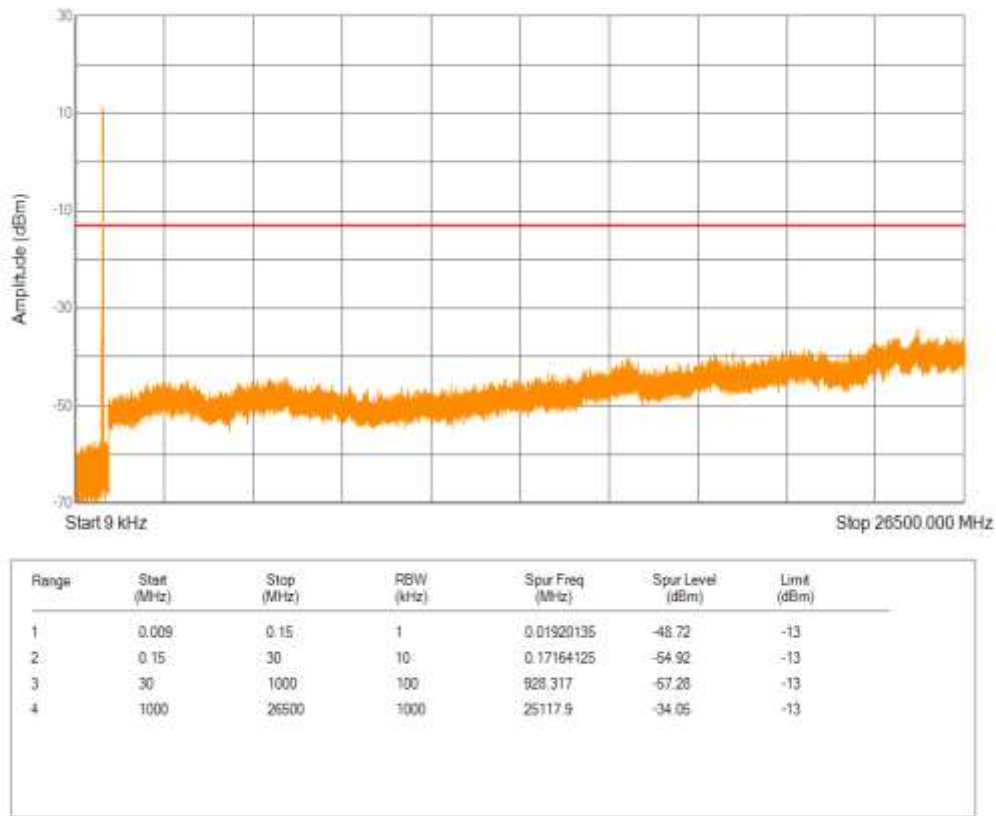
Band26(824-849) QAM16 BW=15MHz Channel=26965 RB Size=75 Position=#0
