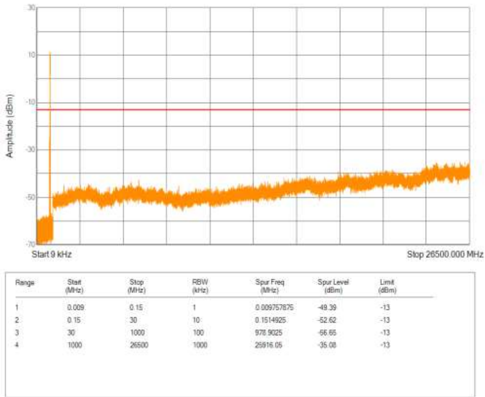
Band26(824-849) QAM16 BW=15MHz Channel=26865 RB Size=75 Position=#0
