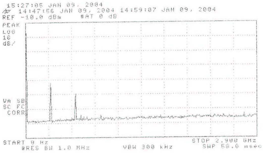
Figure 6.2(b). Emission spectrum of the DUT (310 MHz, 50% duty factor). The amplitudes are only indicative (not calibrated).
