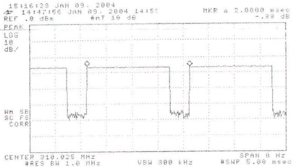
Figure 6.1(c). Transmissions modulation characteristics: (top) pulse width, (bottom) pulse period. (310 MHz, 80% duty factor).
