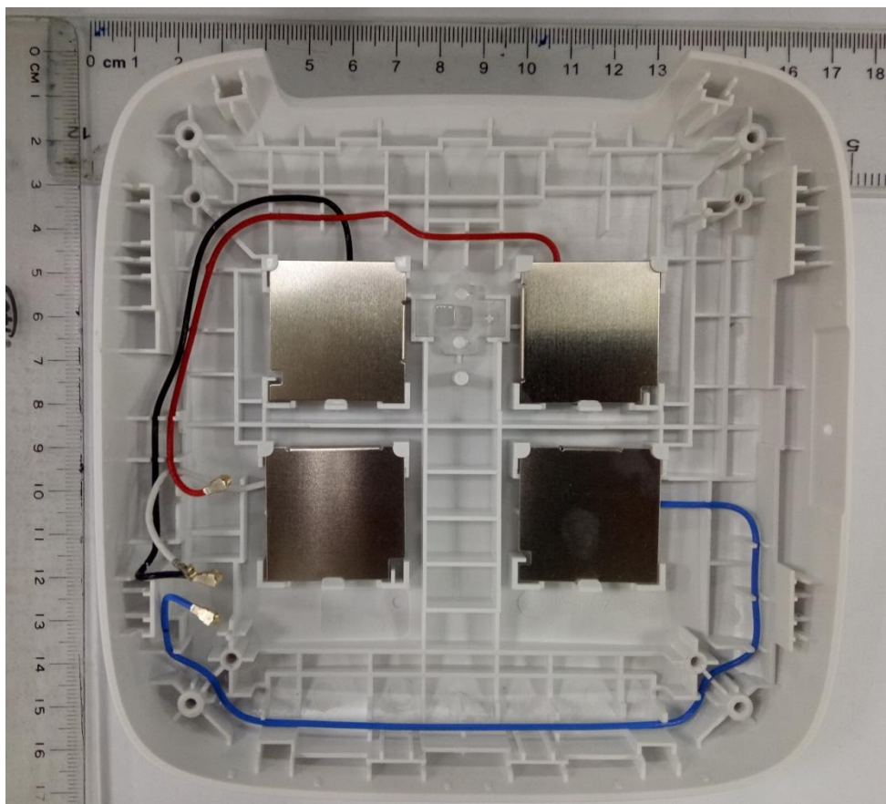
Antenna View
