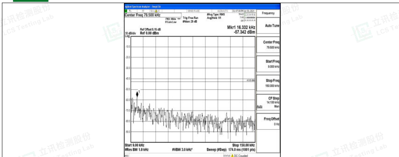
Band4_15MHz_QPSK_20175_1RB#0_0.009~0.15_0.009~0.15
