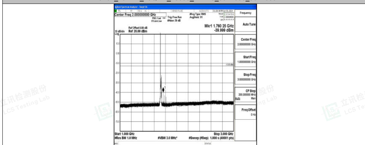
Band4_10MHz_16QAM_20000_1RB#0_1000~3000_1000~3000
