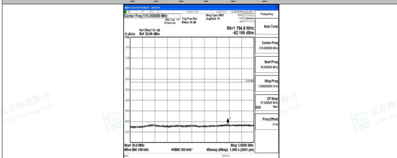
Band4_3MHz_QPSK_19965_1RB#0_30~1000_30~1000
