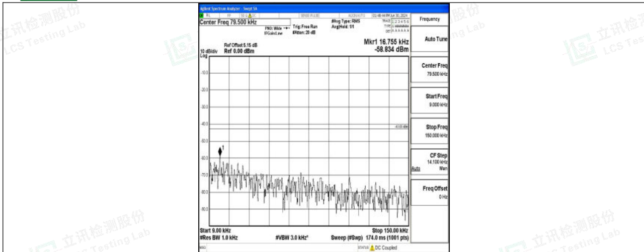
Band4_15MHz_16QAM_20325_1RB#0_0.009~0.15_0.009~0.15
