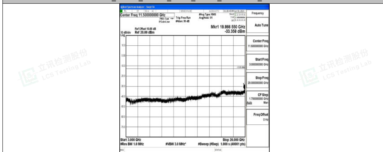
Band4_10MHz_16QAM_20000_1RB#0_3000~20000_3000~20000
