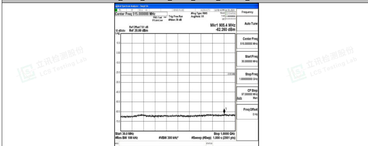
Band4_3MHz_16QAM_20385_1RB#0_30~1000_30~1000
