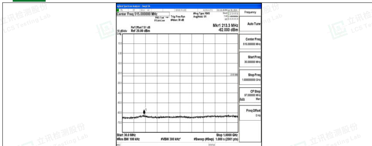
Band4_5MHz_QPSK_20375_1RB#0_30~1000_30~1000
