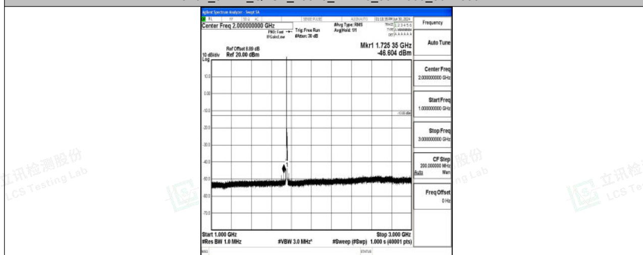
Band4_5MHz_QPSK_20375_1RB#0_1000~3000_1000~3000
