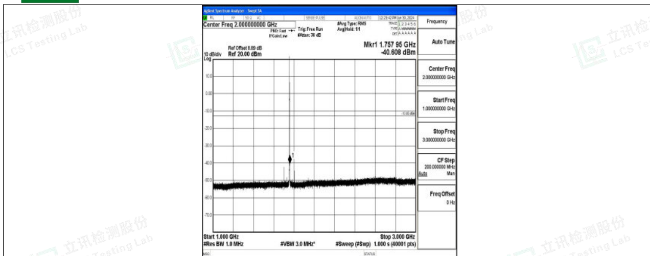
Band4_1.4MHz_16QAM_20393_1RB#0_1000~3000_1000~3000
