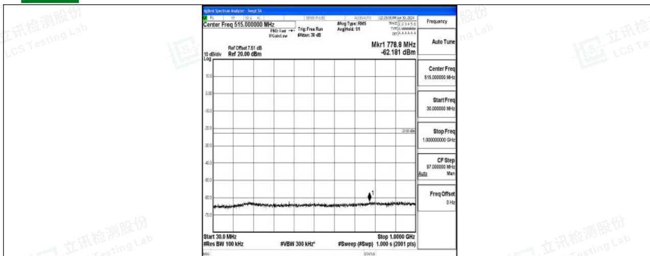
Band4_1.4MHz_QPSK_20393_1RB#0_30~1000_30~1000
