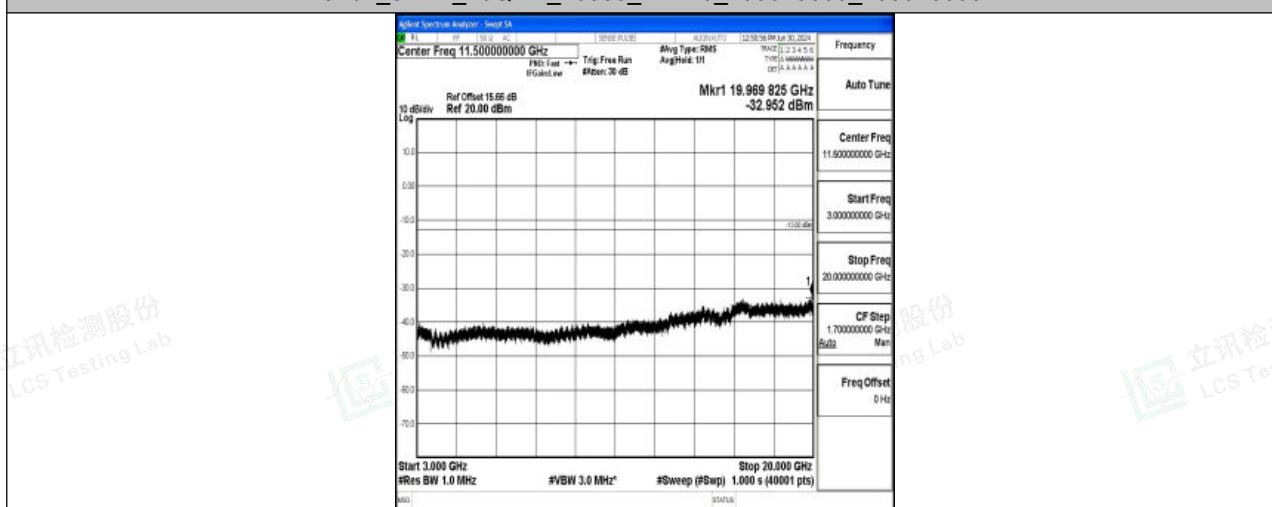
Band4_3MHz_16QAM_20385_1RB#0_3000~20000_3000~20000
