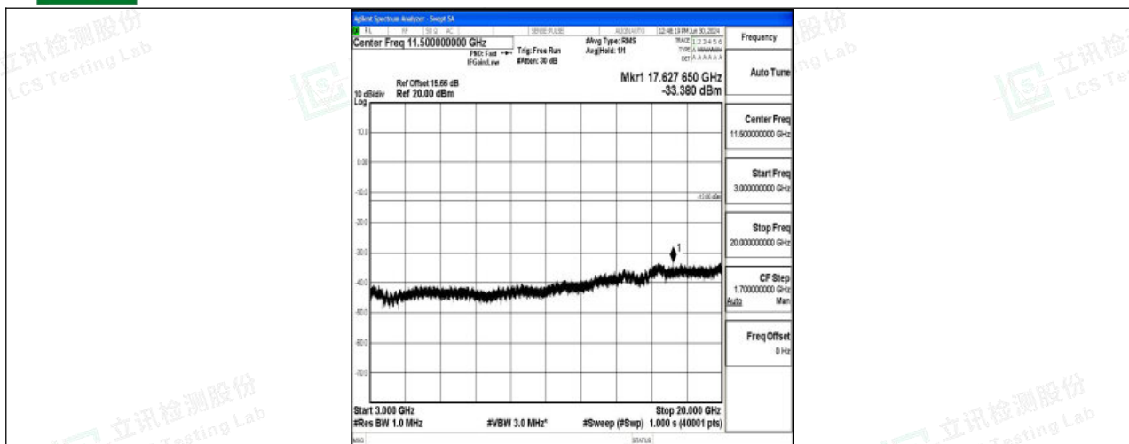
Band4_3MHz_QPSK_19965_1RB#0_3000~20000_3000~20000
