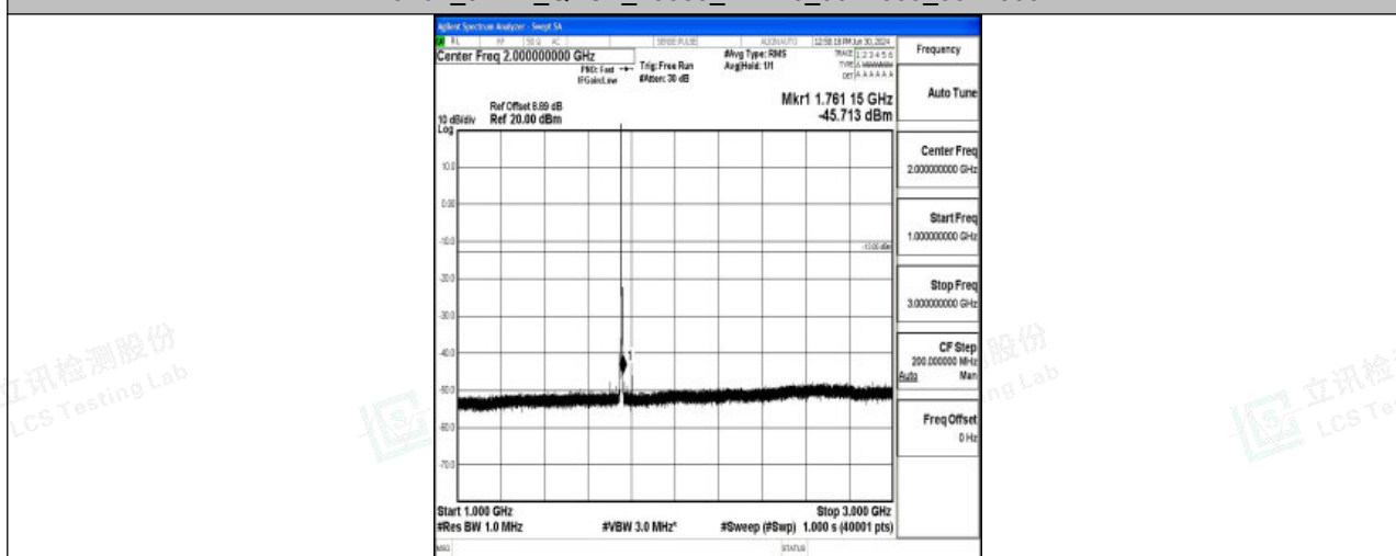
Band4_3MHz_QPSK_20385_1RB#0_1000~3000_1000~3000
