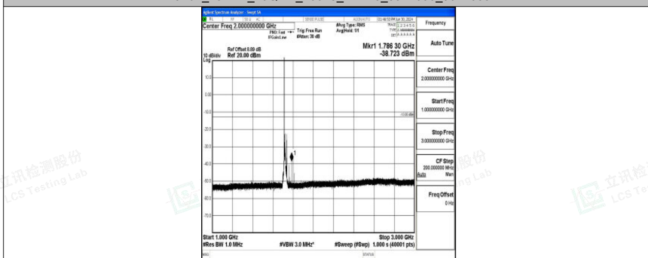
Band4_15MHz_16QAM_20025_1RB#0_1000~3000_1000~3000
