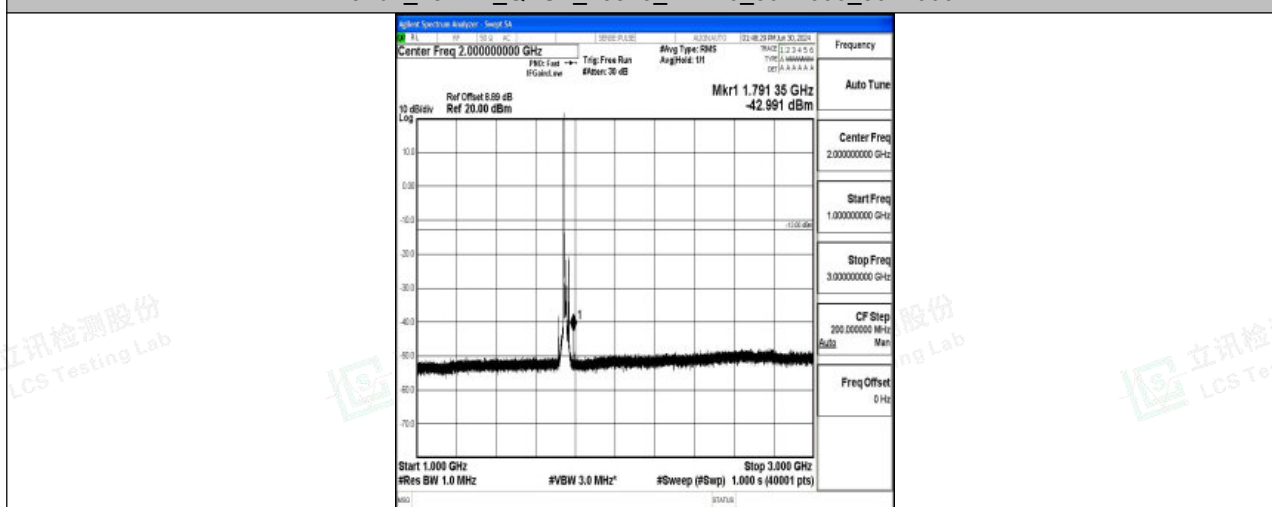
Band4_15MHz_QPSK_20325_1RB#0_1000~3000_1000~3000
