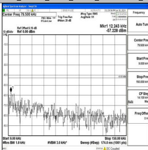
Band4_10MHz_QPSK_20350_1RB#0_0.009~0.15_0.009~0.15
