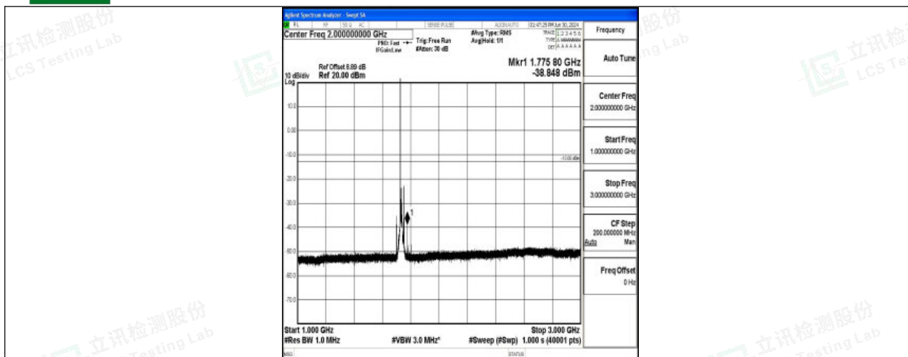
Band4_15MHz_QPSK_20175_1RB#0_1000~3000_1000~3000
