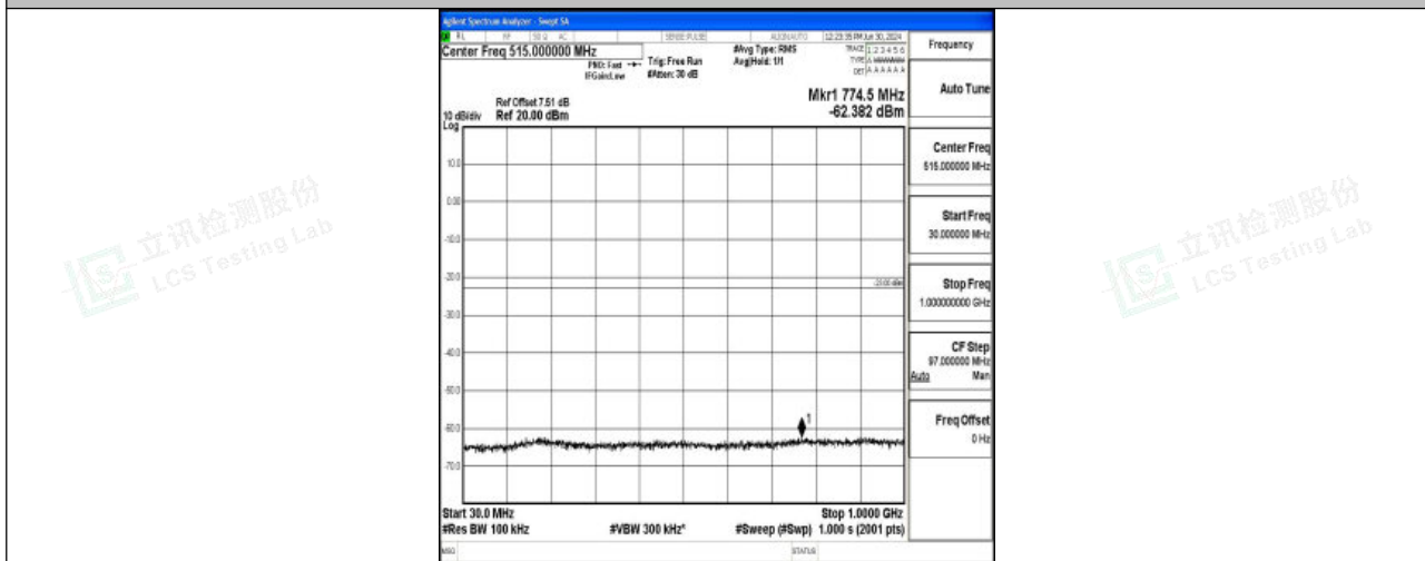
Band4_1.4MHz_16QAM_20393_1RB#0_30~1000_30~1000
