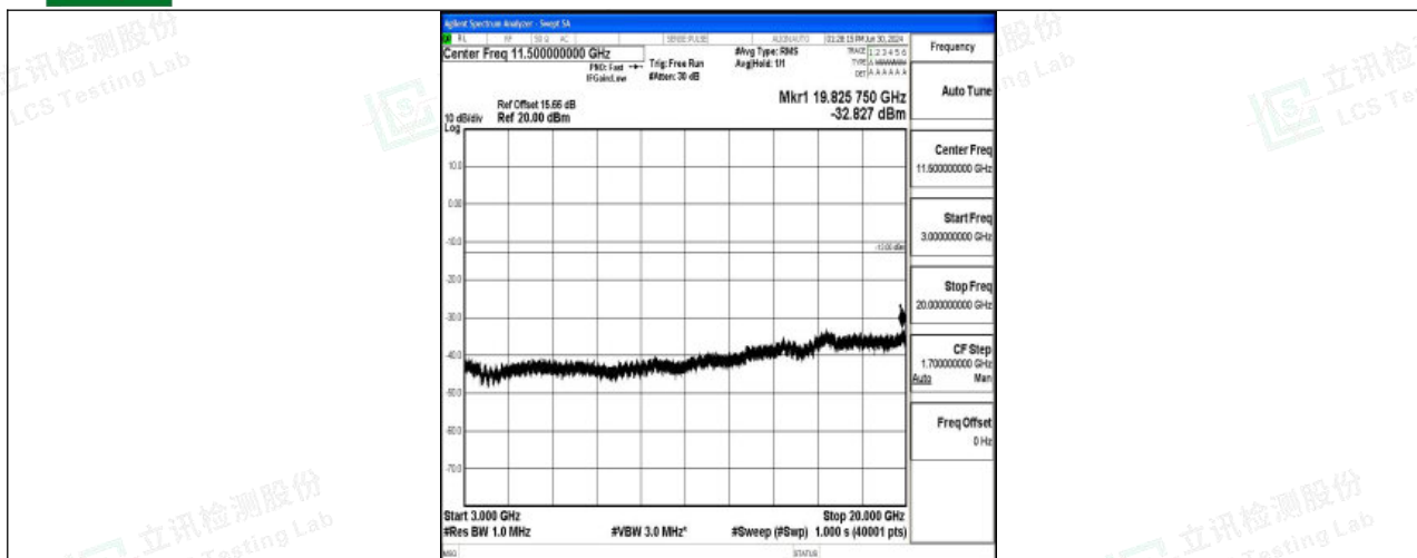
Band4_10MHz_QPSK_20000_1RB#0_3000~20000_3000~20000
