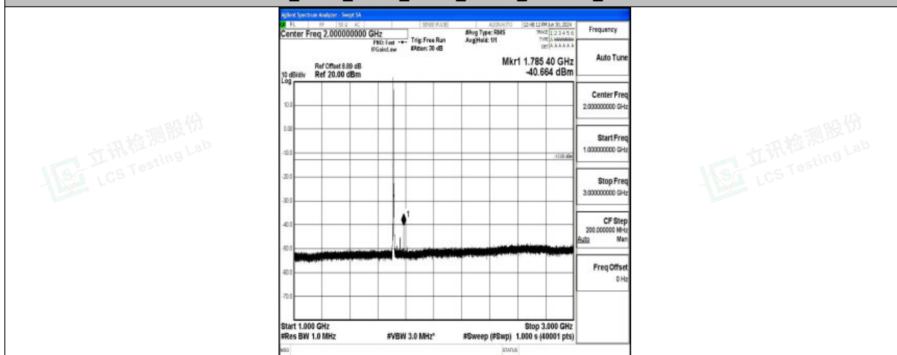
Band4_3MHz_QPSK_19965_1RB#0_1000~3000_1000~3000
