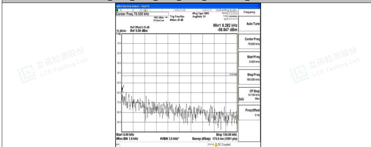
Band4_5MHz_16QAM_20175_1RB#0_0.009~0.15_0.009~0.15
