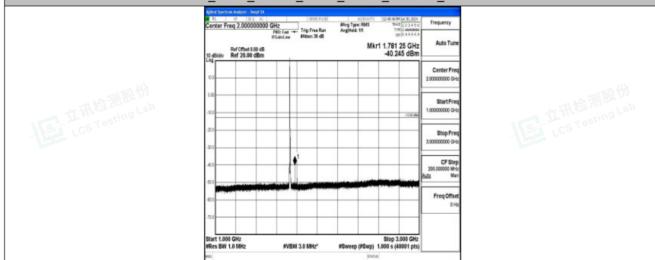
Band4_3MHz_16QAM_20175_1RB#0_1000~3000_1000~3000
