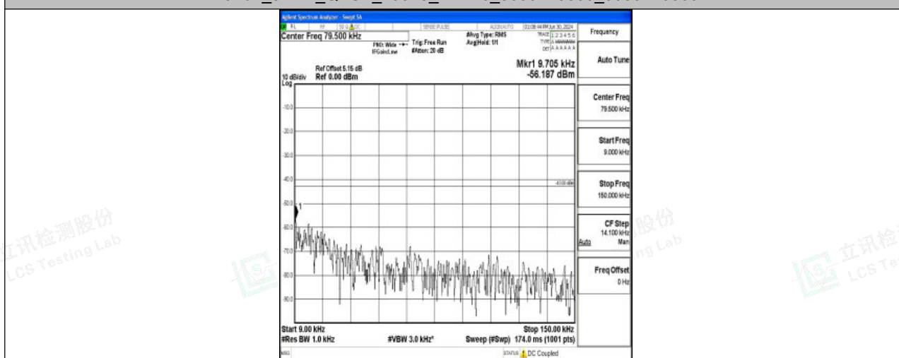
Band4_5MHz_16QAM_19975_1RB#0_0.009~0.15_0.009~0.15
