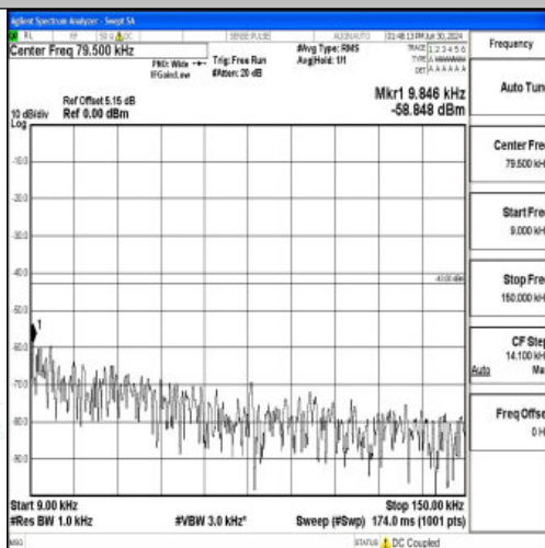
Band4_15MHz_QPSK_20325_1RB#0_0.009~0.15_0.009~0.15
