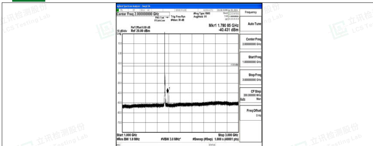
Band4_5MHz_QPSK_20175_1RB#0_1000~3000_1000~3000
