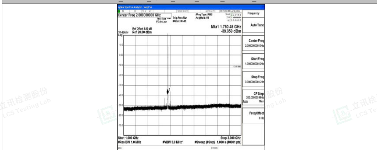
Band4_1.4MHz_QPSK_20393_1RB#0_1000~3000_1000~3000
