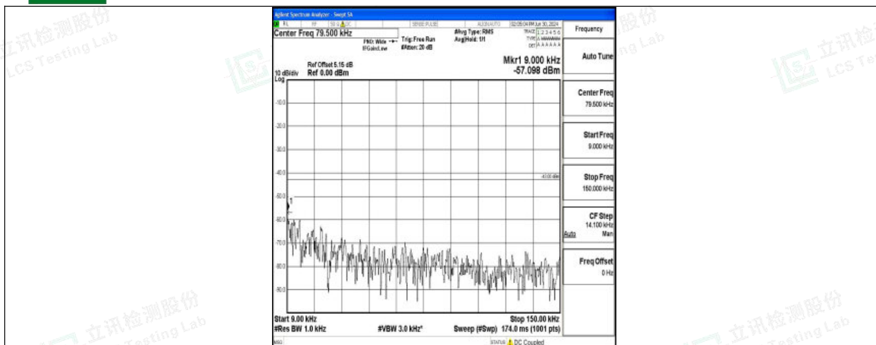
Band4_20MHz_QPSK_20175_1RB#0_0.009~0.15_0.009~0.15
