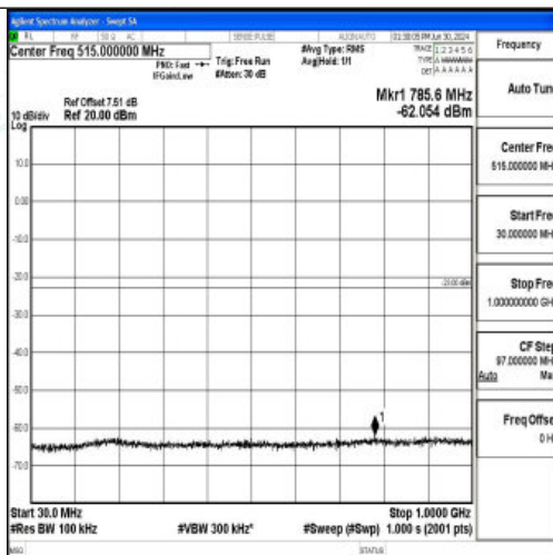
Band4_10MHz_QPSK_20350_1RB#0_30~1000_30~1000
