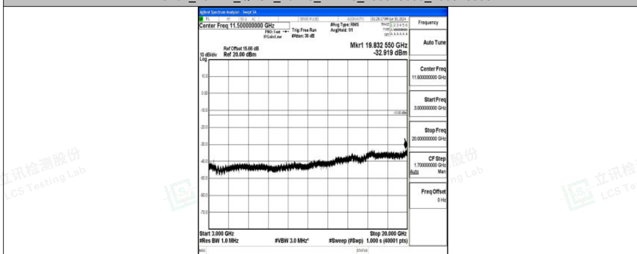
Band4_10MHz_QPSK_20175_1RB#0_3000~20000_3000~20000
