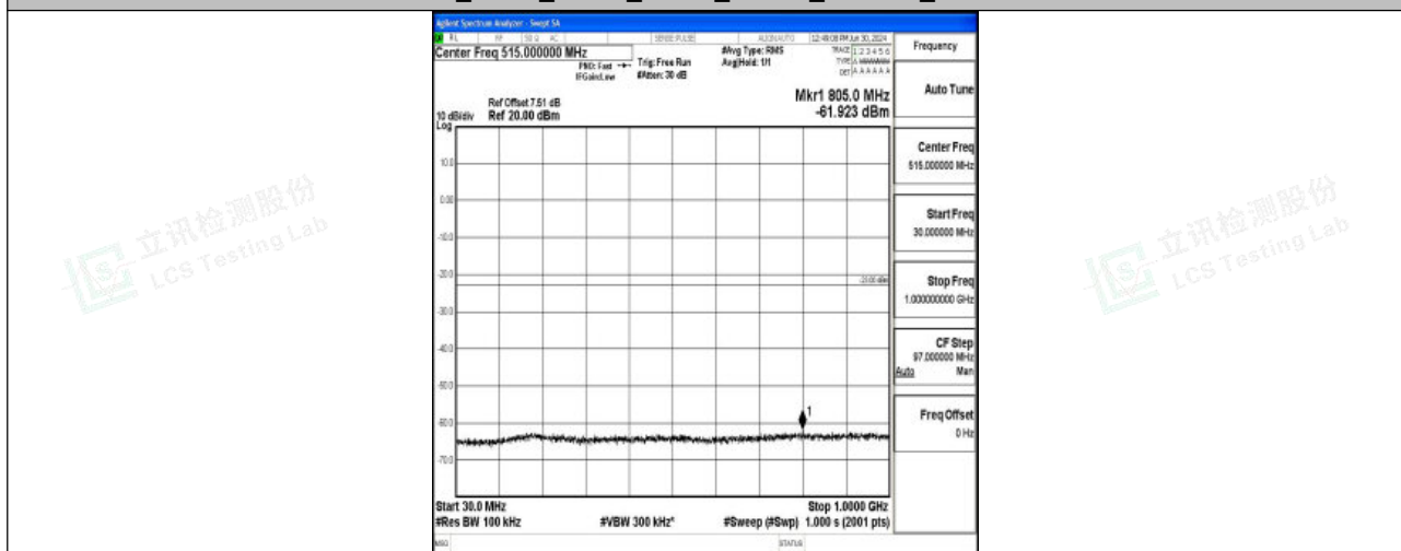
Band4_3MHz_QPSK_20175_1RB#0_30~1000_30~1000
