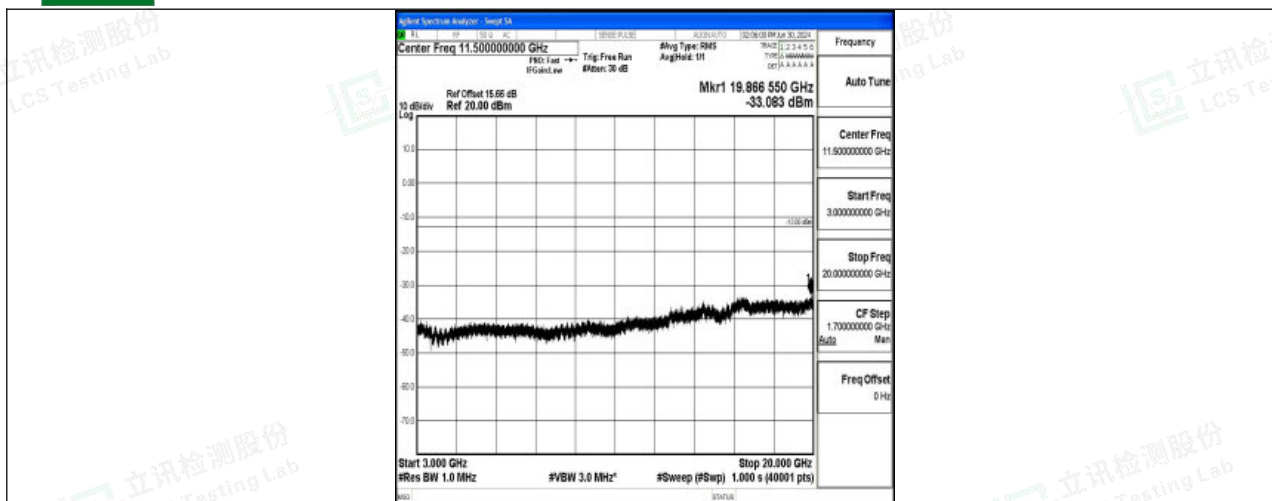
Band4_20MHz_16QAM_20175_1RB#0_3000~20000_3000~20000
