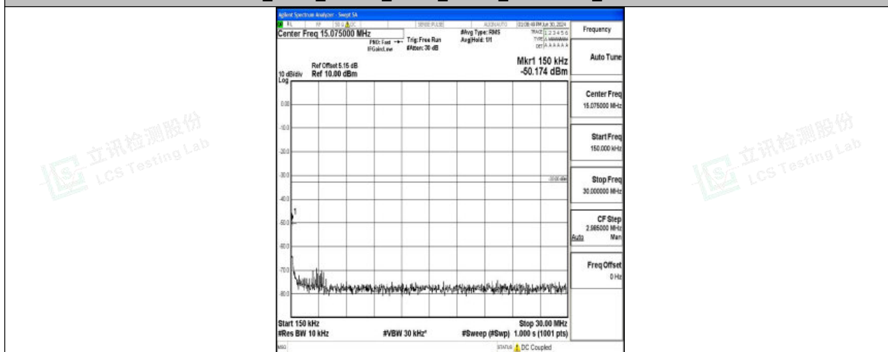
Band4_5MHz_16QAM_19975_1RB#0_0.15~30_0.15~30
