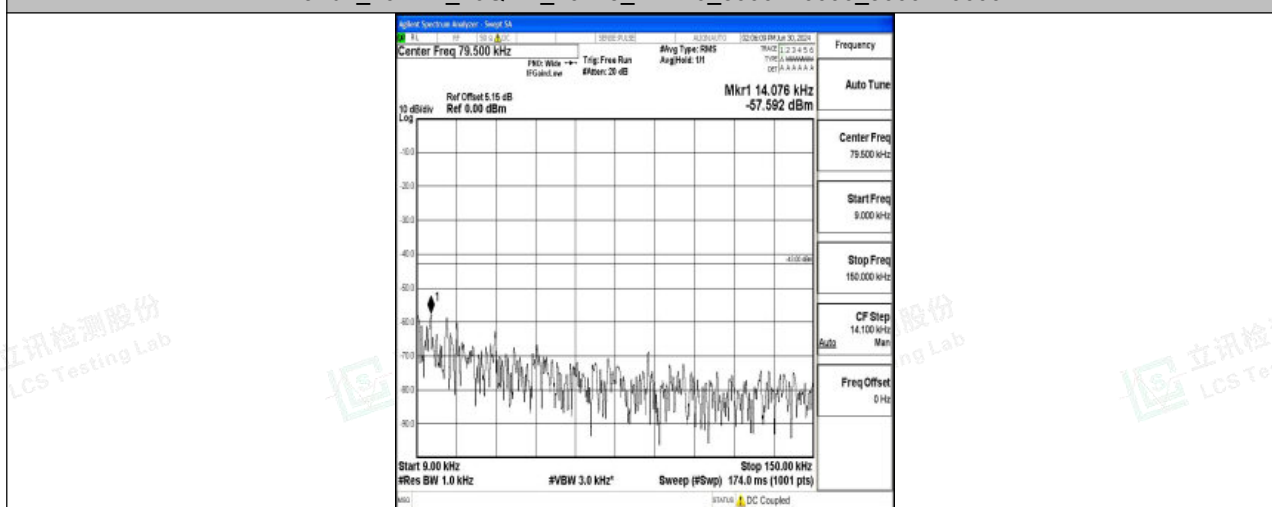
Band4_20MHz_QPSK_20300_1RB#0_0.009~0.15_0.009~0.15
