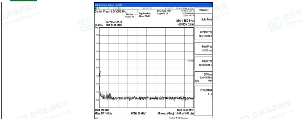
Band4_15MHz_QPSK_20025_1RB#0_0.15~30_0.15~30
