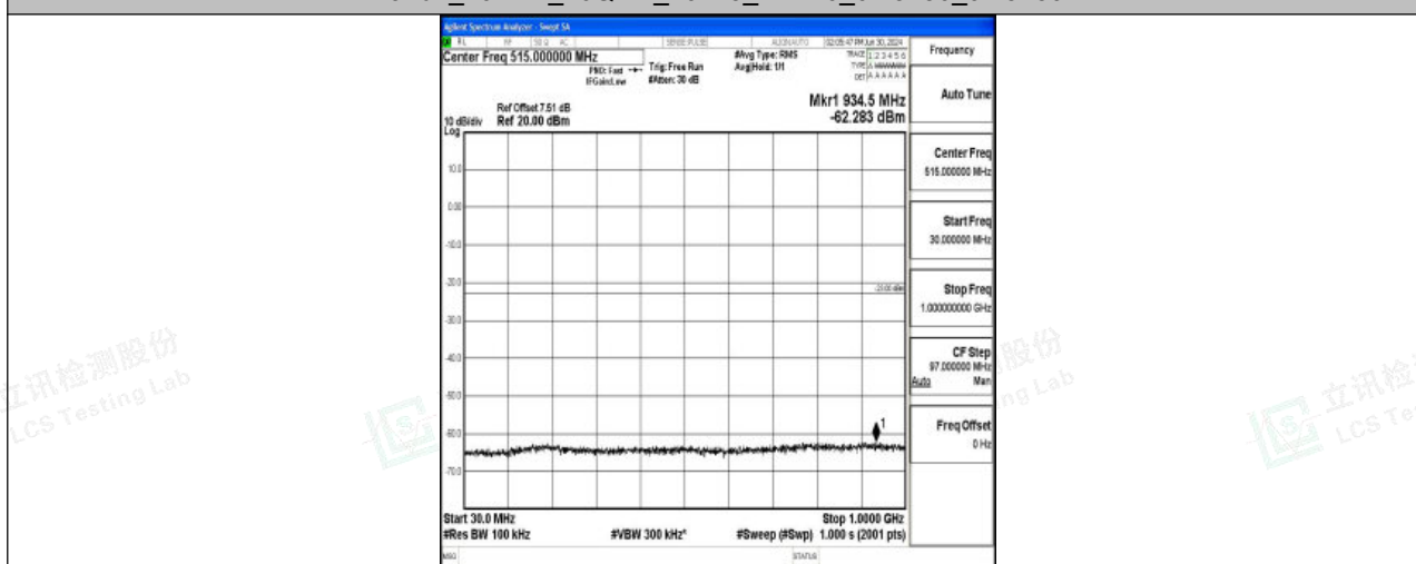
Band4_20MHz_16QAM_20175_1RB#0_30~1000_30~1000
