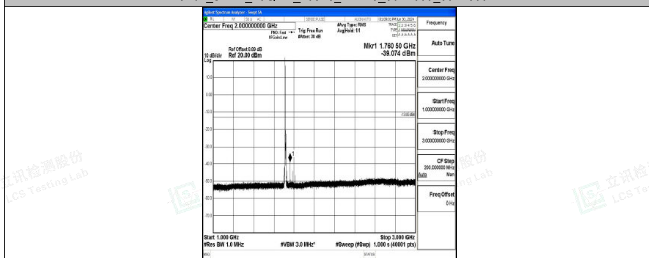
Band4_5MHz_16QAM_19975_1RB#0_1000~3000_1000~3000
