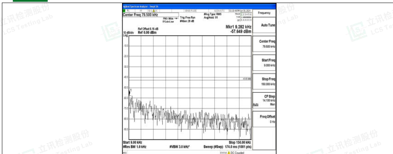
Band4_5MHz_16QAM_20375_1RB#0_0.009~0.15_0.009~0.15
