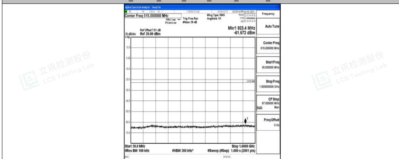
Band4_20MHz_QPSK_20175_1RB#0_30~1000_30~1000
