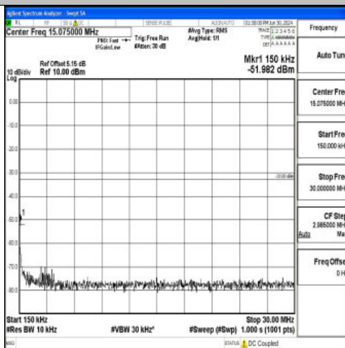
Band4_10MHz_QPSK_20350_1RB#0_0.15~30_0.15~30
