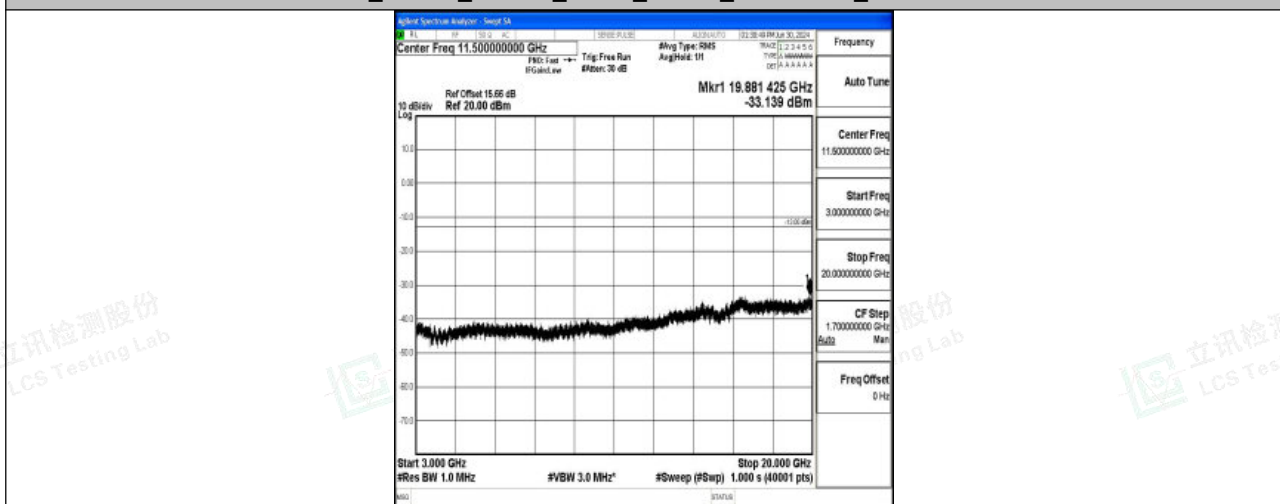
Band4_10MHz_16QAM_20350_1RB#0_3000~20000_3000~20000
