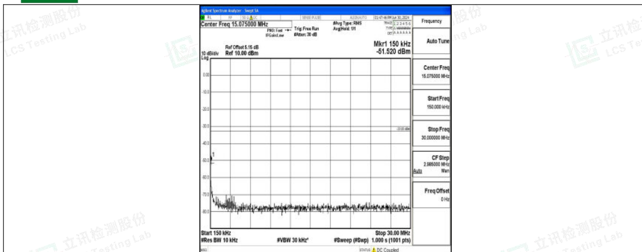
Band4_15MHz_16QAM_20175_1RB#0_0.15~30_0.15~30
