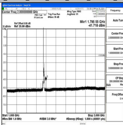
Band4_10MHz_QPSK_20350_1RB#0_1000~3000_1000~3000
