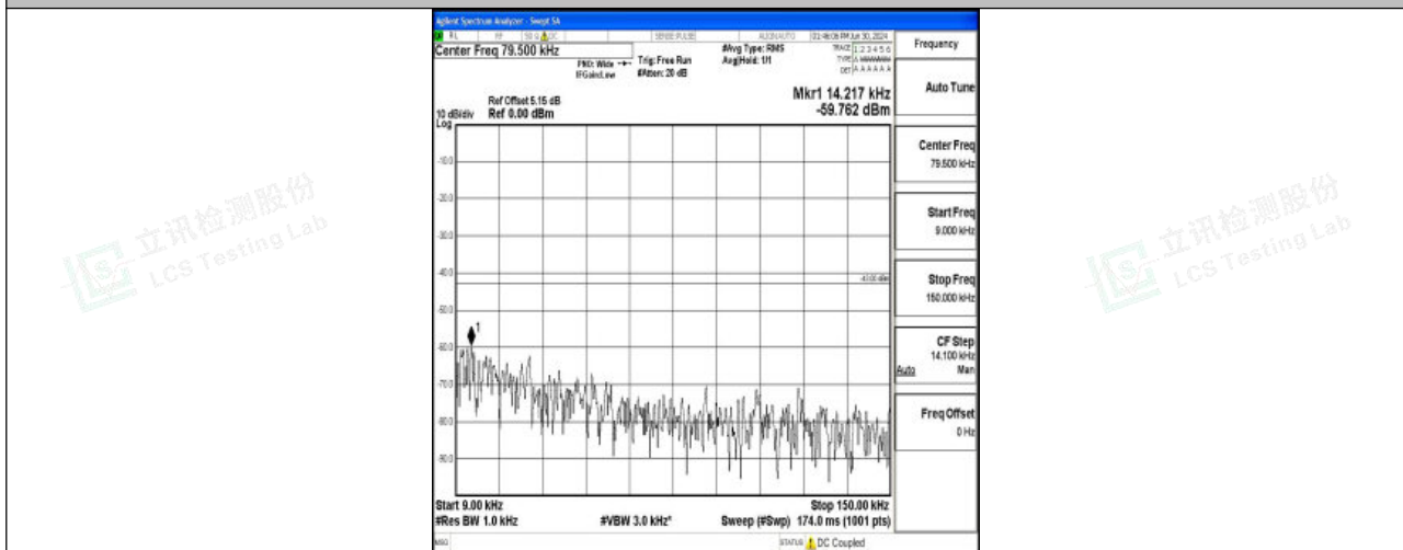
Band4_15MHz_QPSK_20025_1RB#0_0.009~0.15_0.009~0.15
