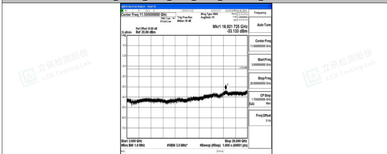
Band4_1.4MHz_QPSK_20393_1RB#0_3000~20000_3000~20000
