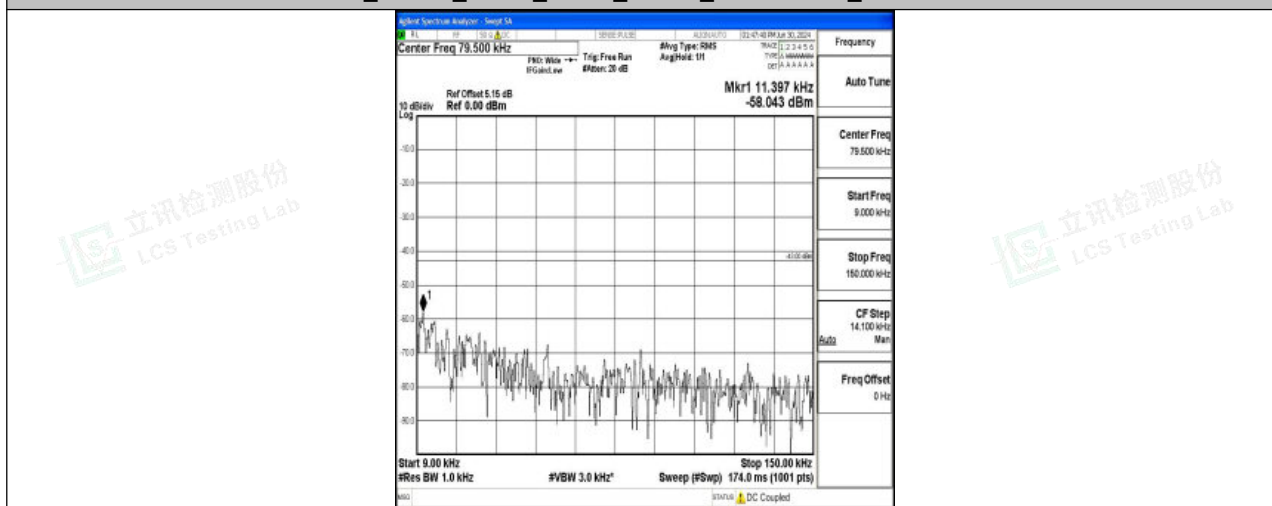
Band4_15MHz_16QAM_20175_1RB#0_0.009~0.15_0.009~0.15
