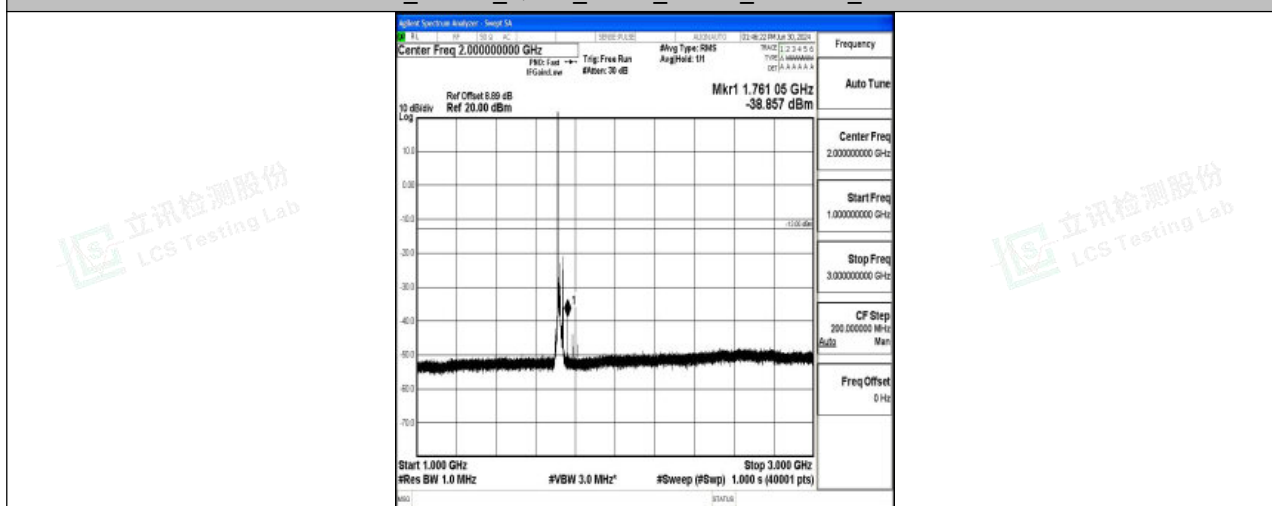
Band4_15MHz_QPSK_20025_1RB#0_1000~3000_1000~3000
