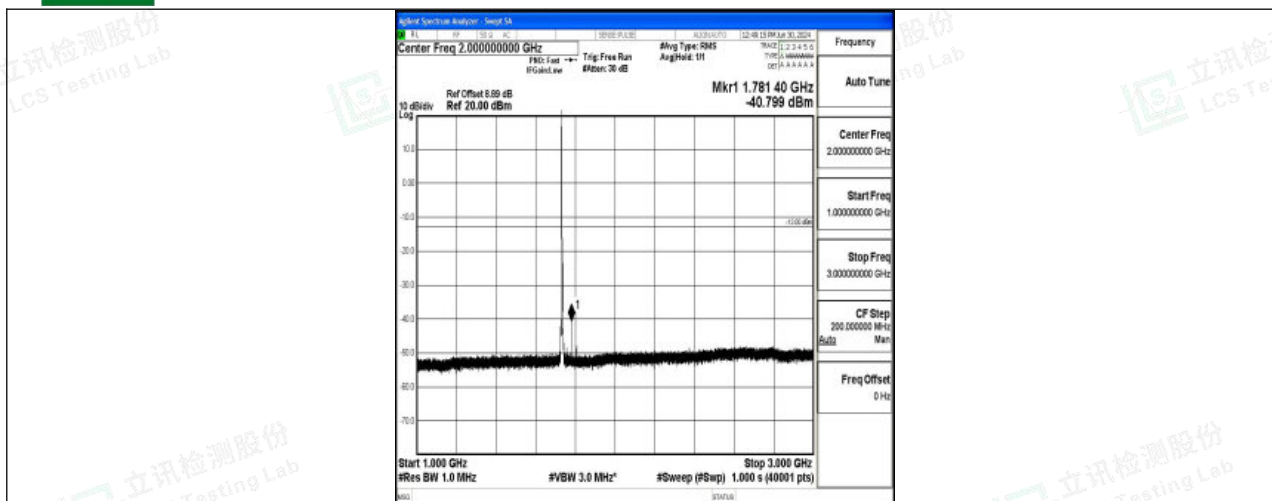
Band4_3MHz_QPSK_20175_1RB#0_1000~3000_1000~3000
