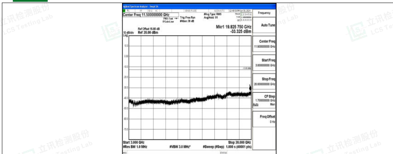
Band4_3MHz_16QAM_20175_1RB#0_3000~20000_3000~20000
