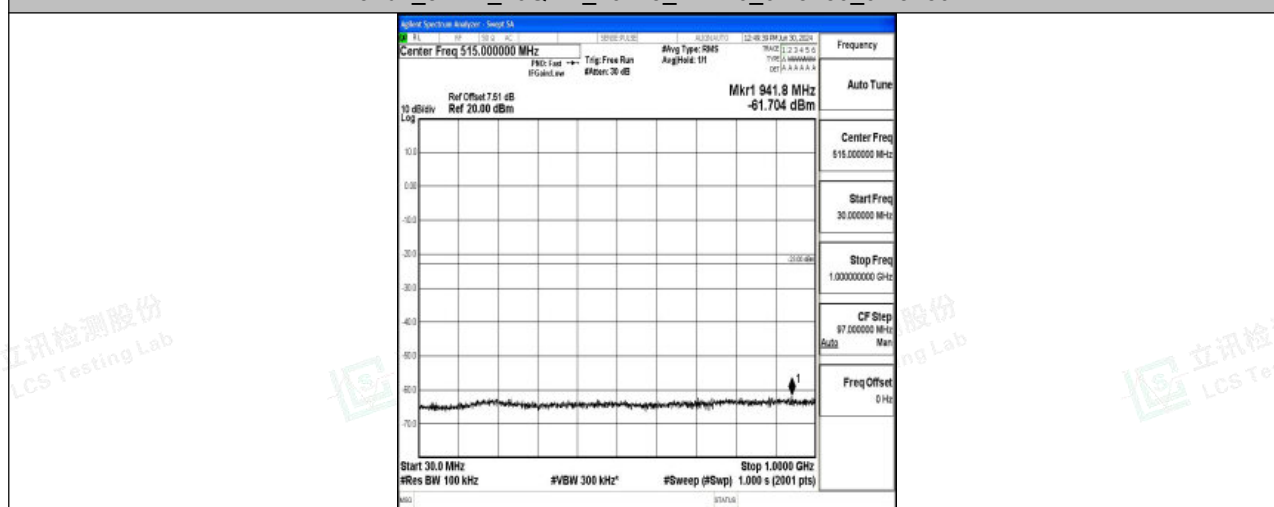
Band4_3MHz_16QAM_20175_1RB#0_30~1000_30~1000
