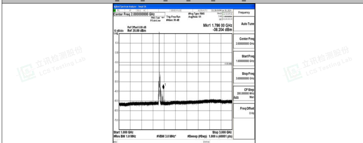
Band4_10MHz_QPSK_20000_1RB#0_1000~3000_1000~3000
