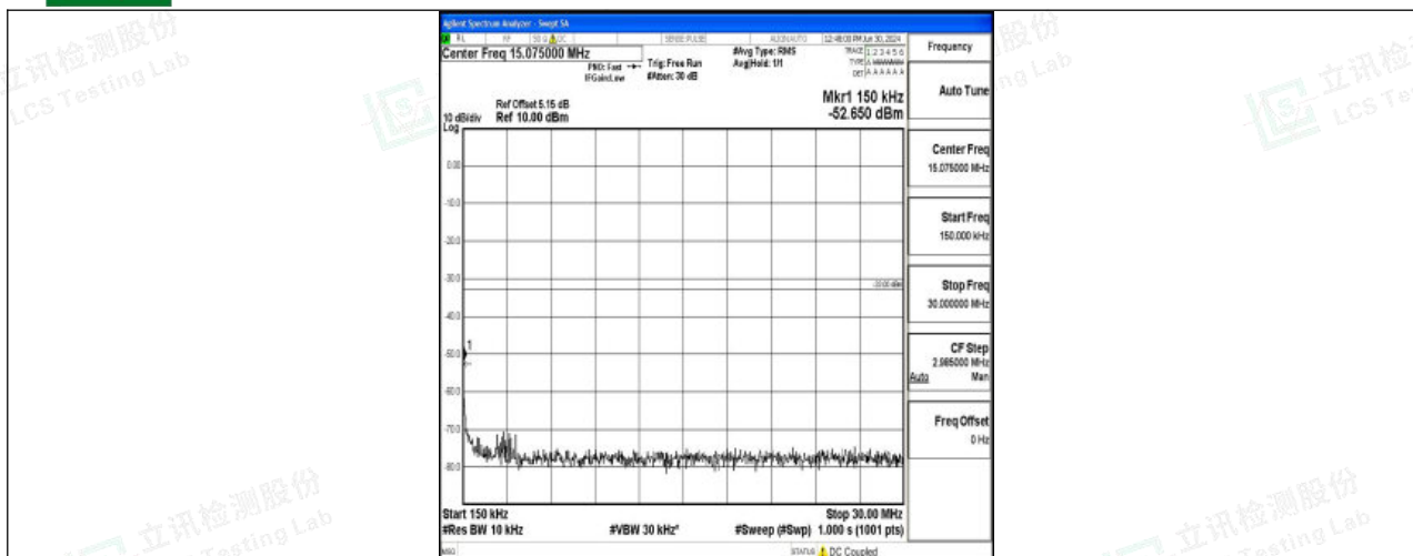
Band4_3MHz_QPSK_19965_1RB#0_0.15~30_0.15~30
