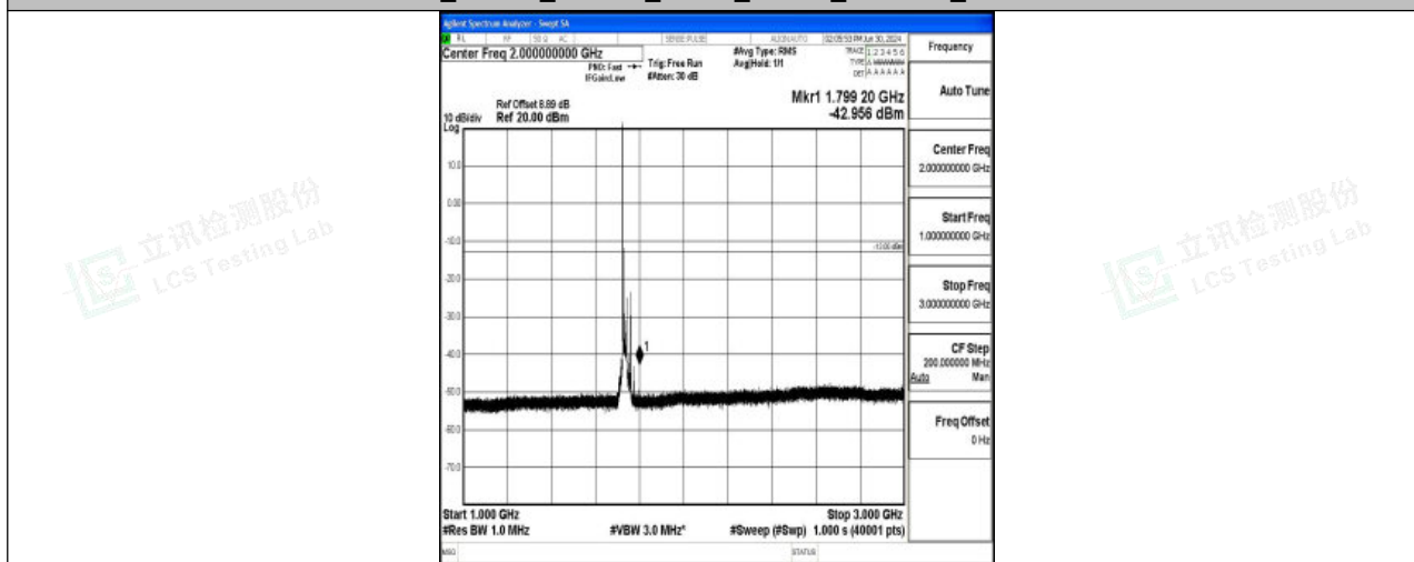
Band4_20MHz_16QAM_20175_1RB#0_1000~3000_1000~3000
