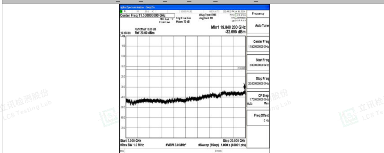
Band4_3MHz_QPSK_20175_1RB#0_3000~20000_3000~20000
