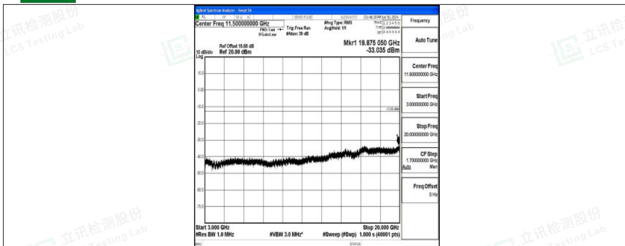
Band4_15MHz_QPSK_20025_1RB#0_3000~20000_3000~20000
