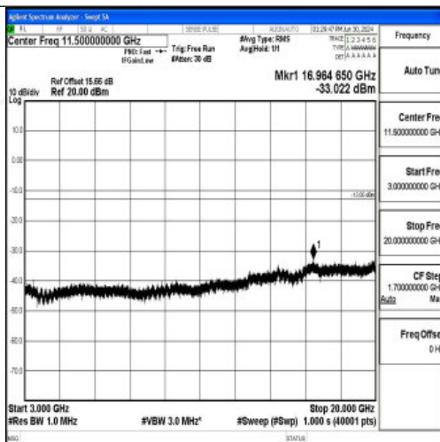
Band4_10MHz_16QAM_20175_1RB#0_3000~20000_3000~20000
