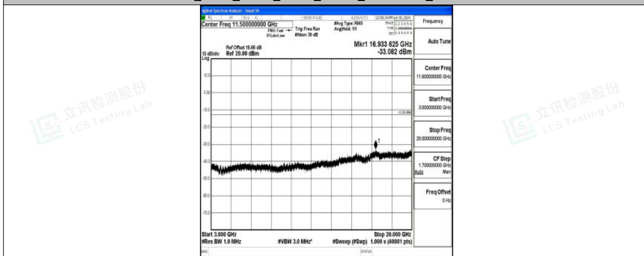
Band4_3MHz_QPSK_20385_1RB#0_3000~20000_3000~20000
