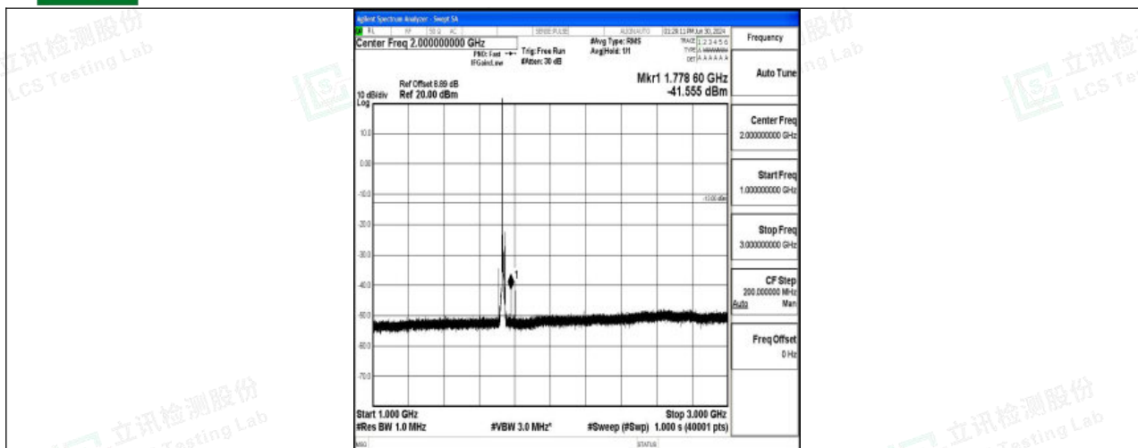
Band4_10MHz_QPSK_20175_1RB#0_1000~3000_1000~3000
