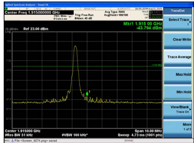
LTE Band 25 10MHz 16QAM 100%RB CH-High
