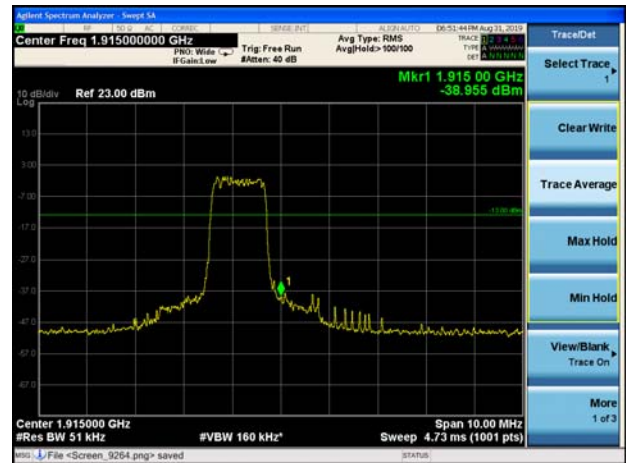
LTE Band 25 5MHz QPSK 1RB CH-High
