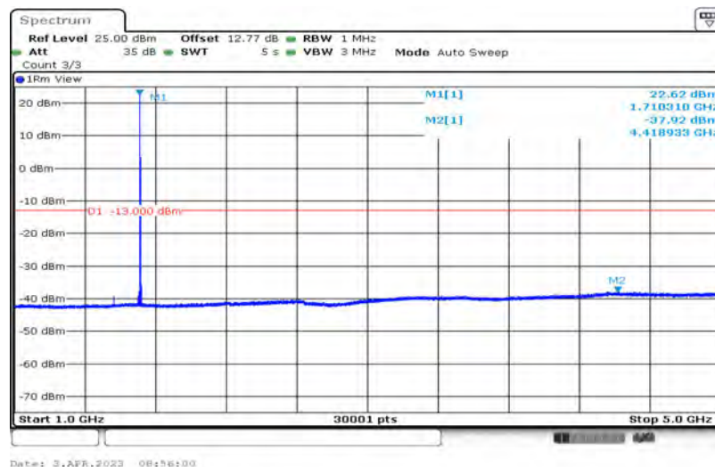
Band66-1.4MHz-16QAM-131979-1-0-Low-1000-5000--37.92-PASS
