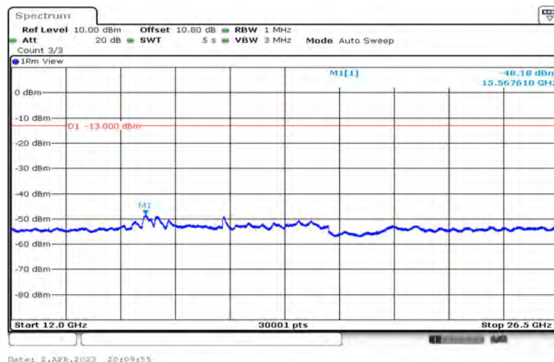
Band26-3MHz-16QAM-26705-1-0-Low-12000-26500--48.18-PASS
