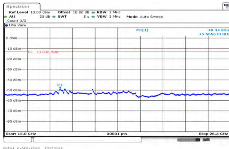
Band26-1.4MHz-16QAM-26740-1-0-Low-12000-26500--48.44-PASS
