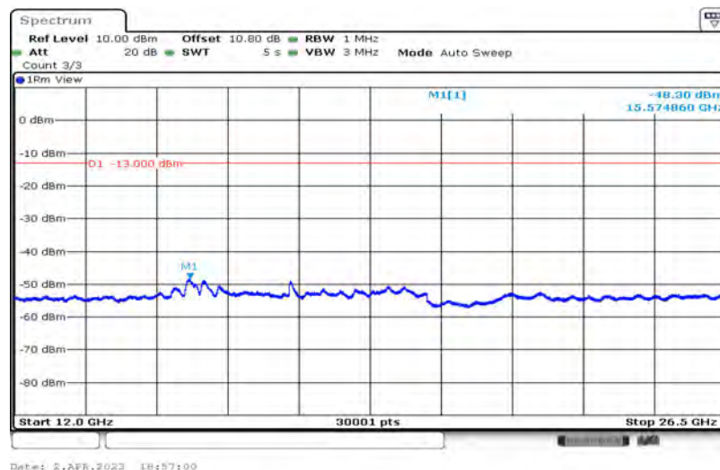
Band26-3MHz-QPSK-26805-1-0-Low-12000-26500--48.3-PASS
