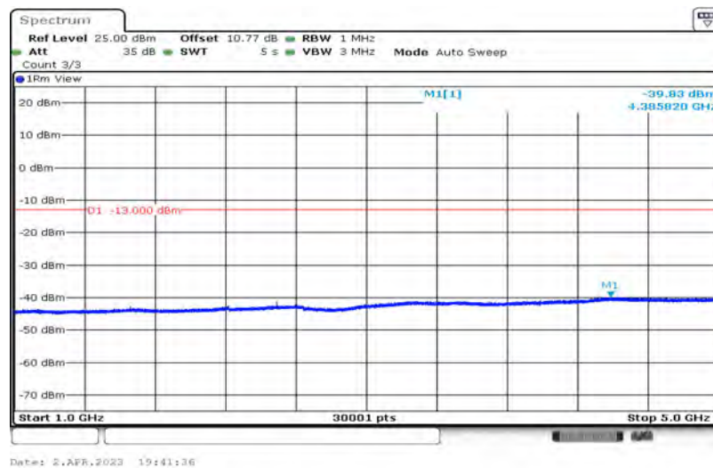
Band26-15MHz-QPSK-26915-1-0-Low-1000-5000--39.83-PASS
