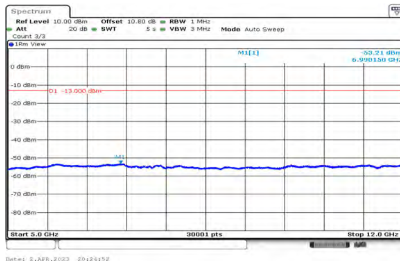
Band26-5MHz-16QAM-26740-1-0-Low-5000-12000--53.21-PASS
