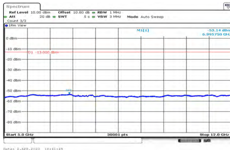
Band26-1.4MHz-16QAM-26797-1-0-Low-5000-12000--53.14-PASS
