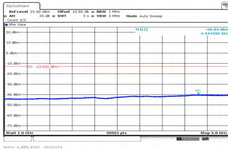
Band26-10MHz-QPSK-26740-1-0-Low-1000-5000--39.83-PASS
