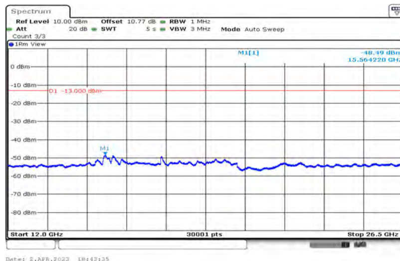
Band26-1.4MHz-QPSK-26915-1-0-Low-12000-26500--48.49-PASS
