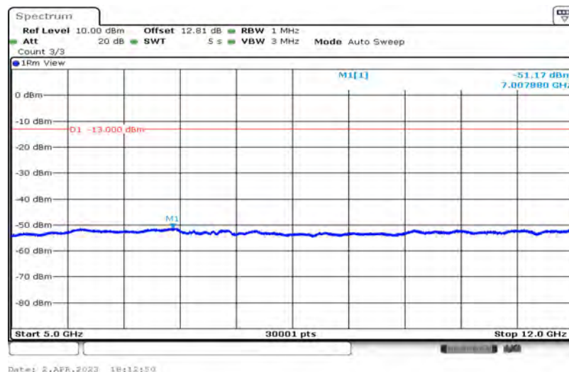
Band25-15MHz-QPSK-26615-1-0-High-5000-12000--51.17-PASS
