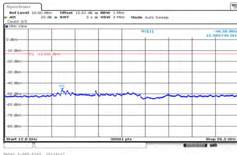
Band25-15MHz-16QAM-26615-1-0-High-12000-26500--46.5-PASS
