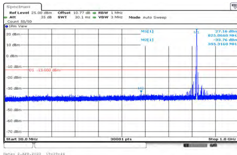
Band26-15MHz-16QAM-26865-1-0-Low-30-1000--33.76-PASS
