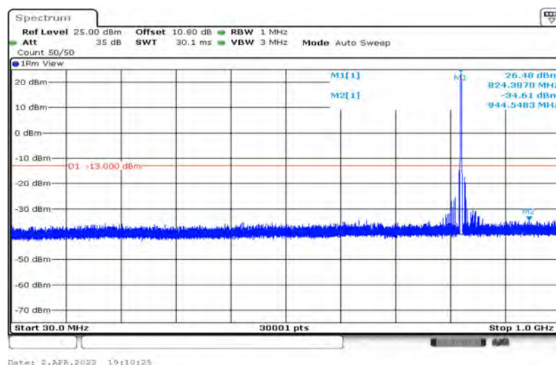
Band26-5MHz-QPSK-26815-1-0-Low-30-1000--34.61-PASS
