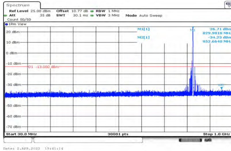
Band26-15MHz-QPSK-26915-1-0-Low-1000-5000--39.83-PASS
