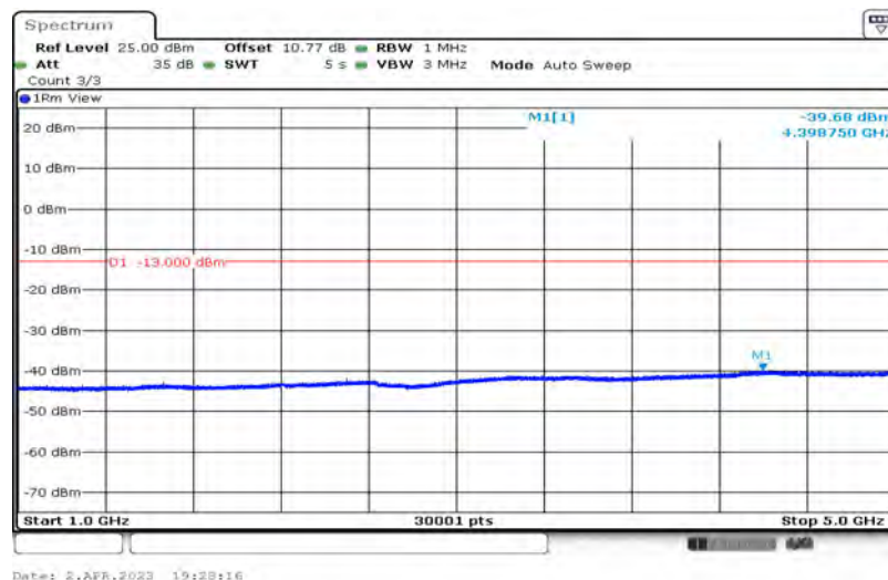
Band26-10MHz-16QAM-26915-1-0-Low-1000-5000--39.68-PASS
