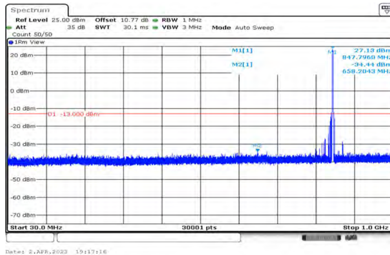
Band26-5MHz-16QAM-27015-1-0-High-30-1000--34.44-PASS
