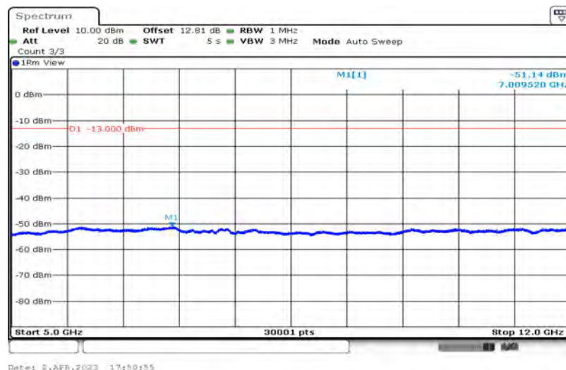
Band25-10MHz-16QAM-26640-1-0-High-5000-12000--51.14-PASS
