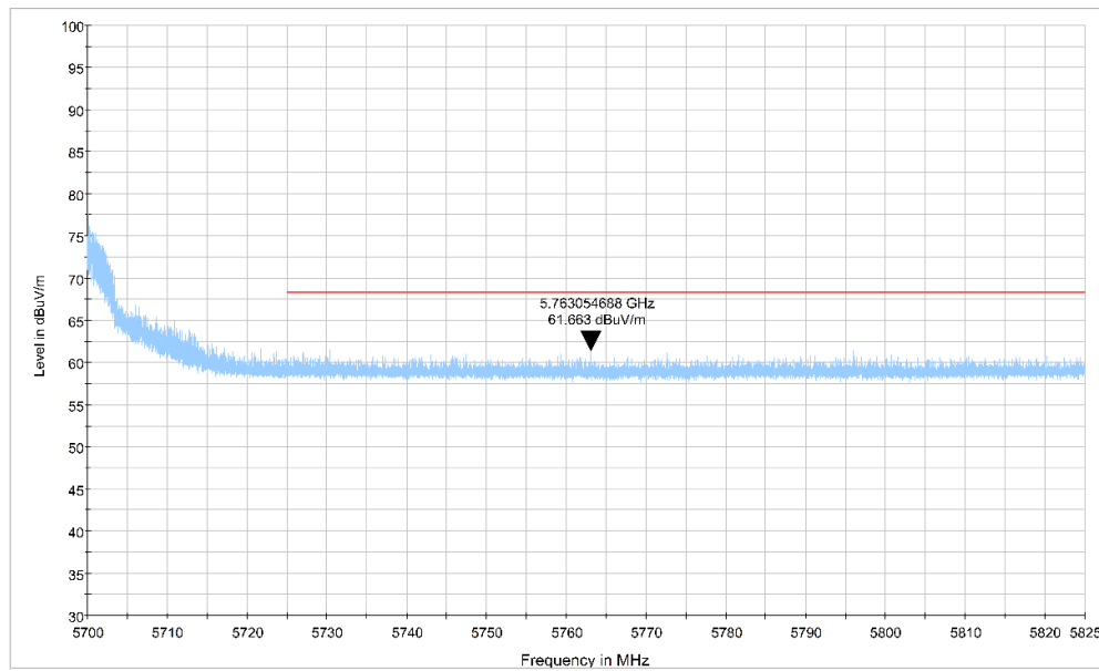
Fig.38 Band Edges (802.11a Ch136, 5680MHz)
