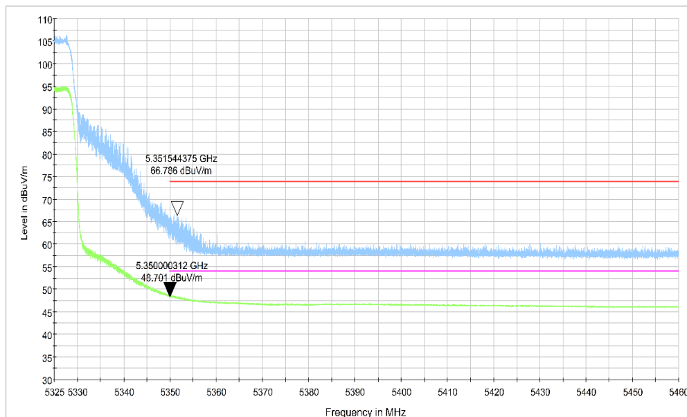
Fig.49 Band Edges (802.11ac-HT20 Ch64, 5320MHz)
