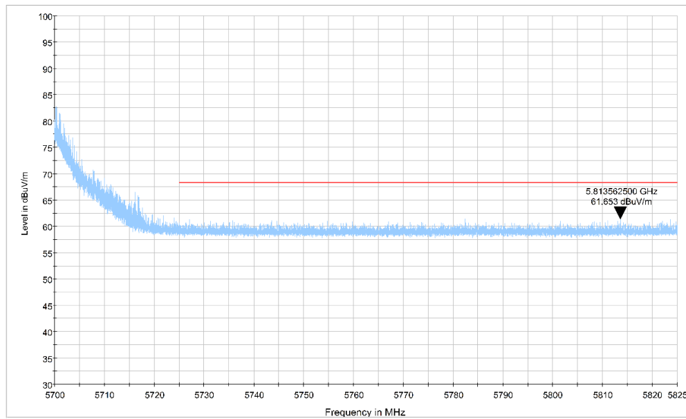
Fig.52 Band Edges (802.11ac-HT20 Ch136, 5680MHz)
