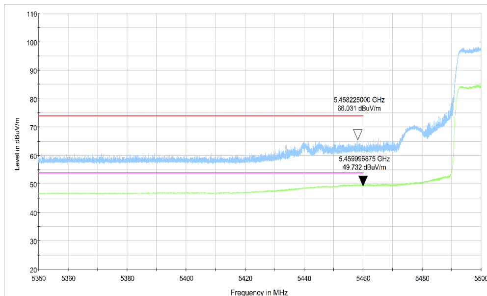
Fig.59 Band Edges (802.11ac-HT80 Ch106, 5530MHz)
