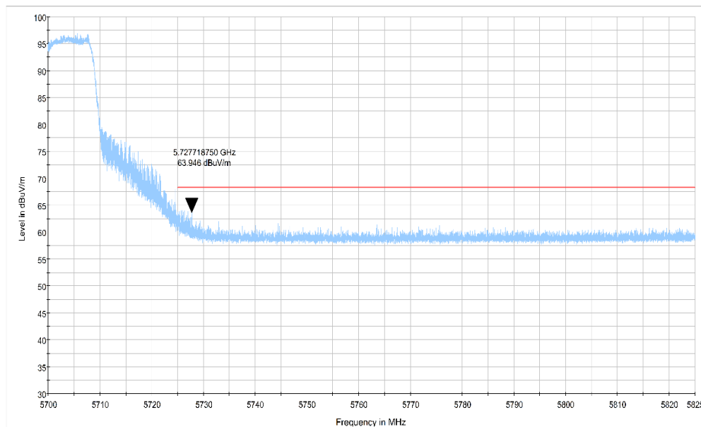
Fig.51 Band Edges (802.11ac-HT20 Ch140, 5700MHz)
