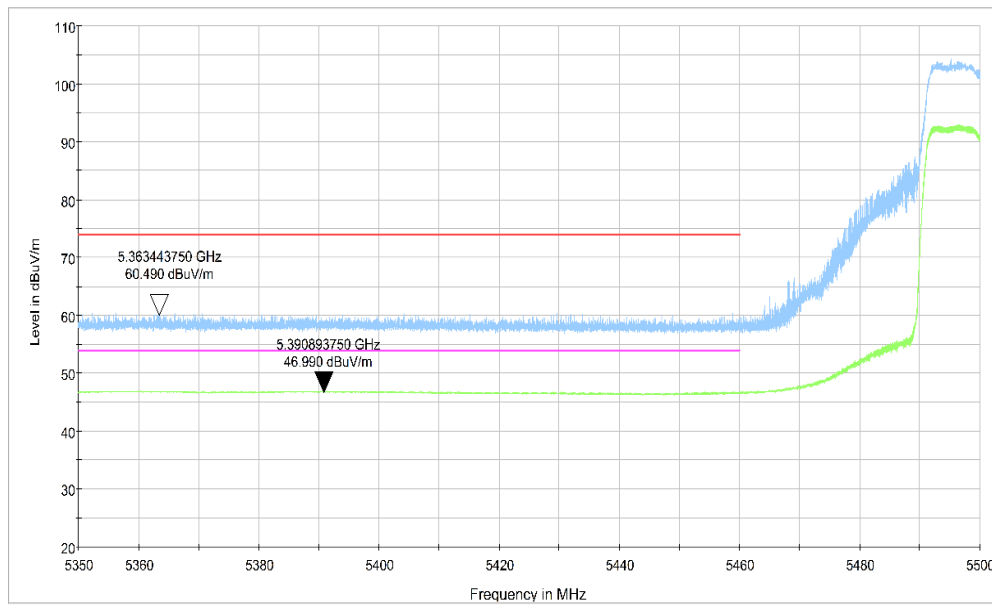
Fig.50 Band Edges (802.11ac-HT20 Ch100, 5500MHz)
