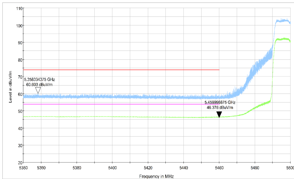
Fig.41 Band Edges (802.11n-HT20 Ch100, 5500MHz)
