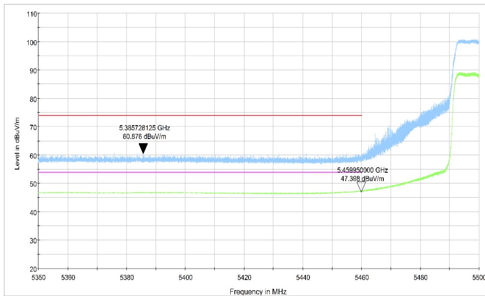
Fig.55 Band Edges (802.11ac-HT40 Ch102, 5510MHz)
