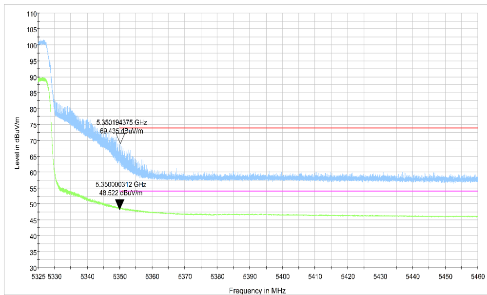
Fig.45 Band Edges (802.11n-HT40 Ch62, 5310MHz)
