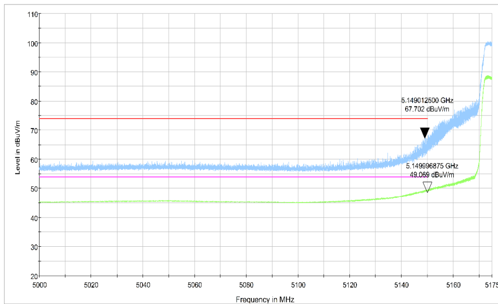
Fig.53 Band Edges (802.11ac-HT40 Ch38, 5190MHz)
