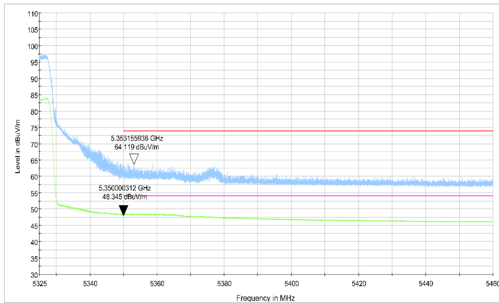
Fig.58 Band Edges (802.11ac-HT80 Ch58, 5290MHz)
