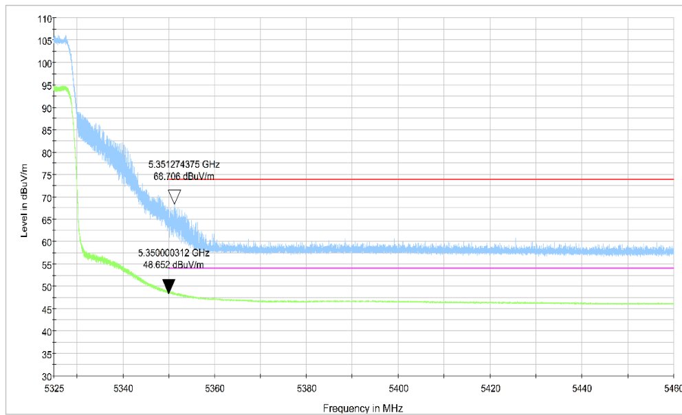
Fig.40 Band Edges (802.11n-HT20 Ch64, 5320MHz)
