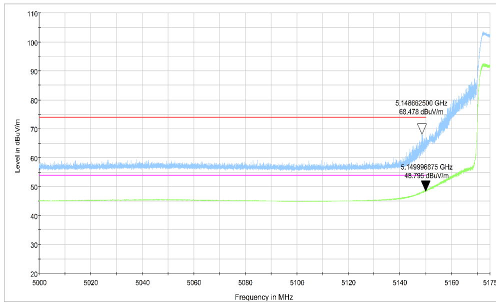
Fig.48 Band Edges (802.11ac-HT20 Ch36, 5180MHz)
