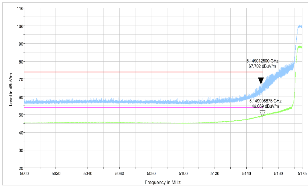
Fig.44 Band Edges (802.11n-HT40 Ch38, 5190MHz)
