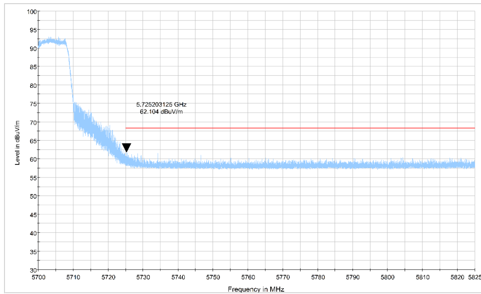
Fig.42 Band Edges (802.11n-HT20 Ch140, 5700MHz)
