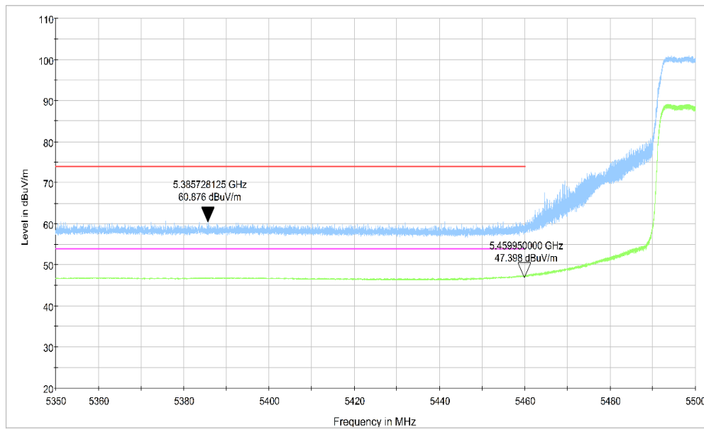
Fig.46 Band Edges (802.11n-HT40 Ch102, 5510MHz)
