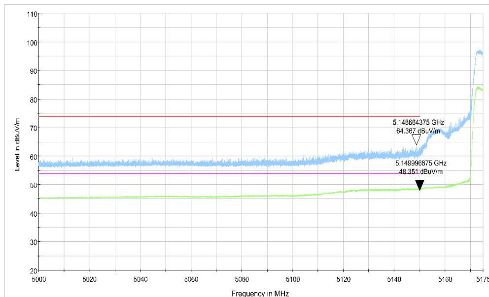
Fig.57 Band Edges (802.11ac-HT80 Ch42 , 5210MHz)
