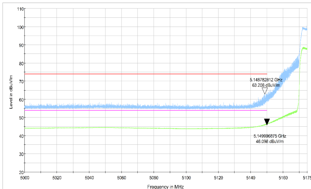
Fig.39 Band Edges (802.11n-HT20 Ch36, 5180MHz)
