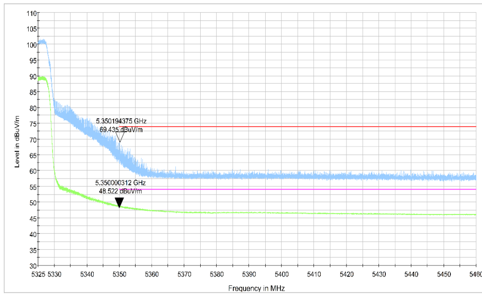
Fig.54 Band Edges (802.11ac-HT40 Ch62, 5310MHz)
