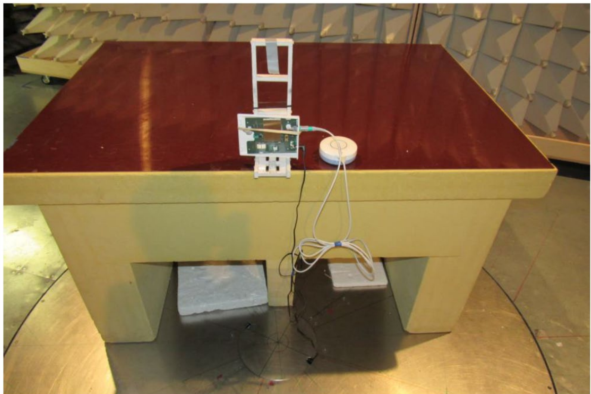
Test setup near view
