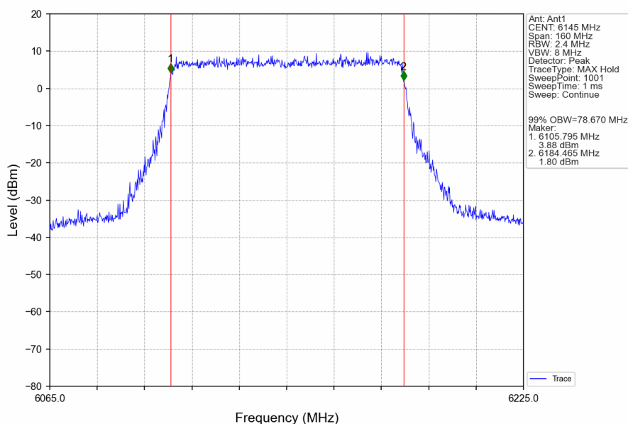
802.11ax(HEW80)_MCH_6145MHz_RU996_Left_Ant1_NTNV
