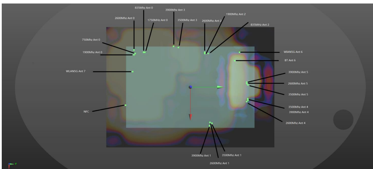
WWAN+WLAN5G Ant6+WLAN5G Ant7+NFC+BT_Bottom Face 0mm
