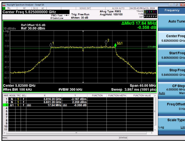
11N20MIMO-Ant0-5825-PASS
