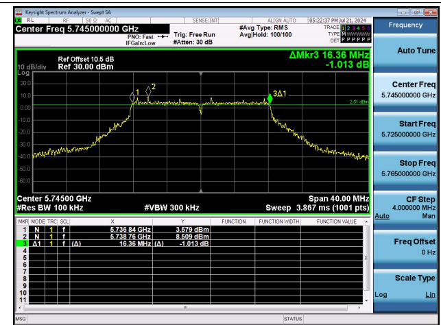
11A-Ant1-5745-PASS
