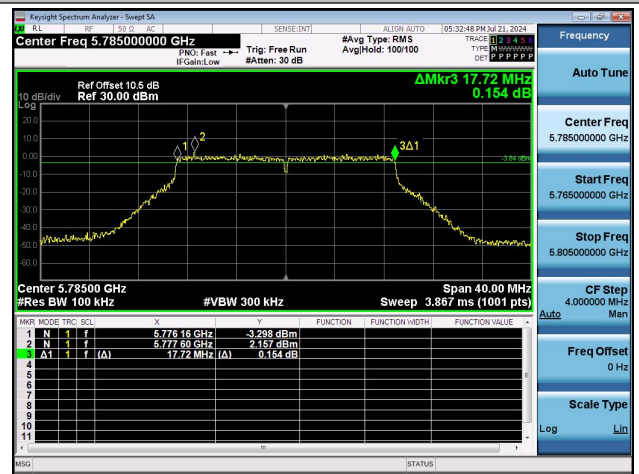
11N20MIMO-Ant1-5785-PASS
