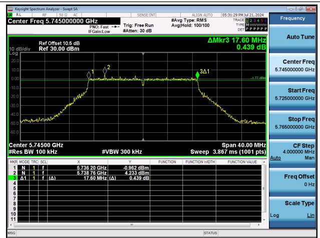
11N20MIMO-Ant1-5745-PASS
