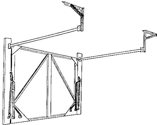
ONE PIECE DOOR WITH TRACK
