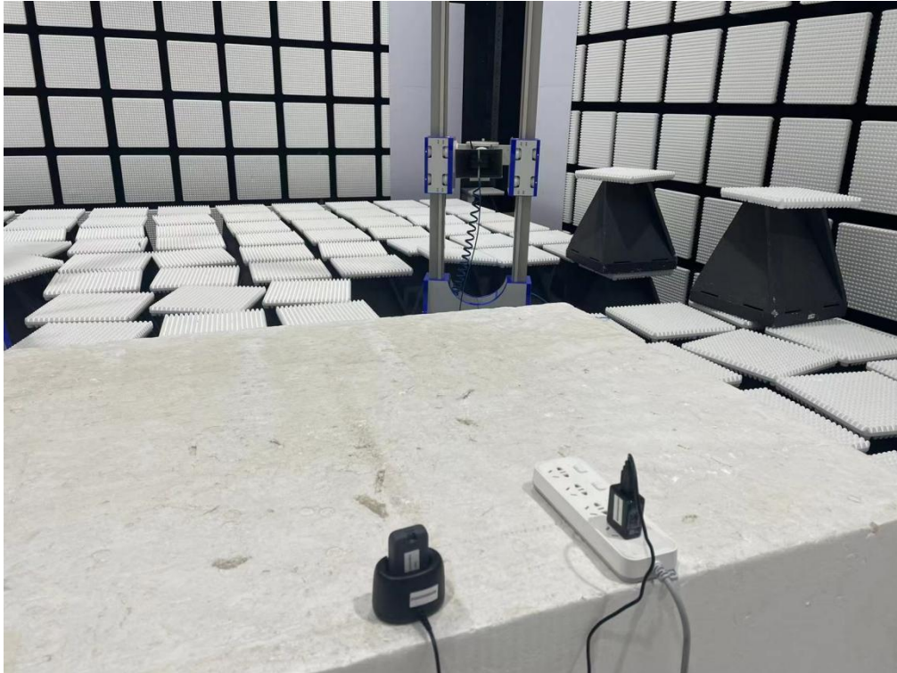
Pic2.Radiatedemissions(1GHz-18GHz)
