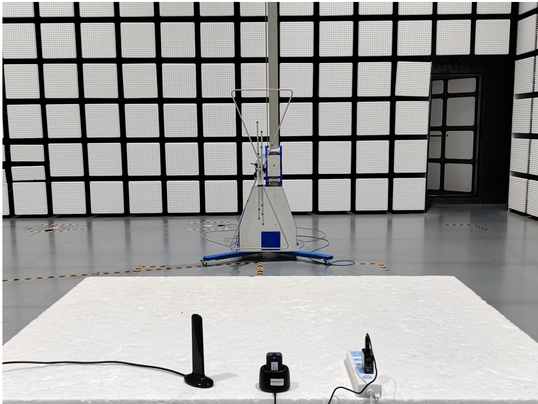
Pic4.RSE(30MHz-1GHz)
