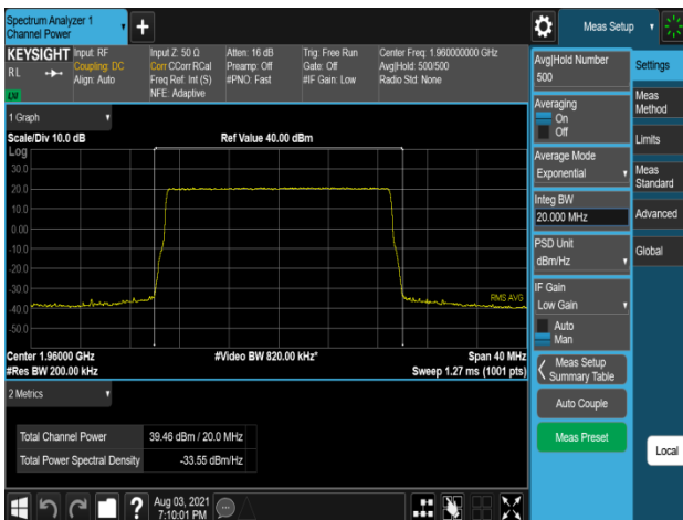
Plot 7-305. Conducted Average Output Power Plot (B2_20M_1C_256QAM - Mid Channel, Port 0)
