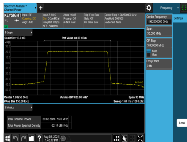
Plot 7-300. Conducted Average Output Power Plot (B2_15M_1C_64QAM - High Channel, Port 3)
