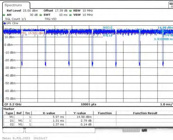
11AC20-CDD_Ant4_5200
