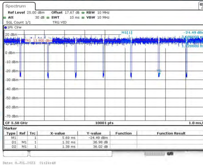
11AC20-CDD_Ant4_5580
