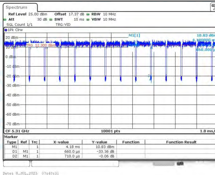
11AC40-CDD_Ant2_5310
