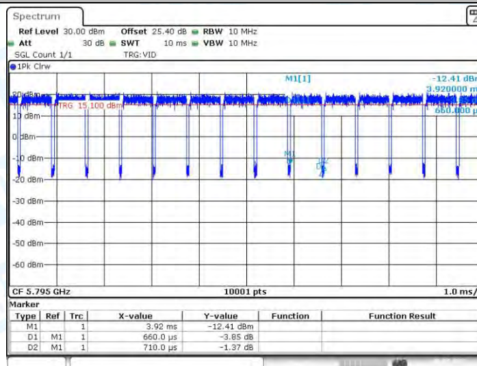
11AC40-CDD_Ant4_5795
