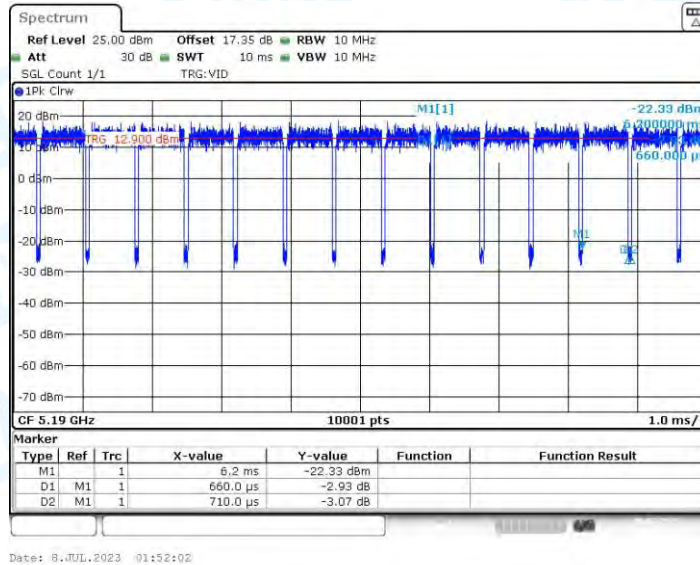
11AC40-CDD_Ant3_5190
