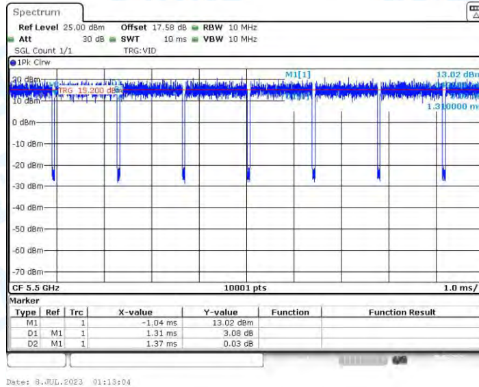
11AC20-CDD_Ant4_5500
