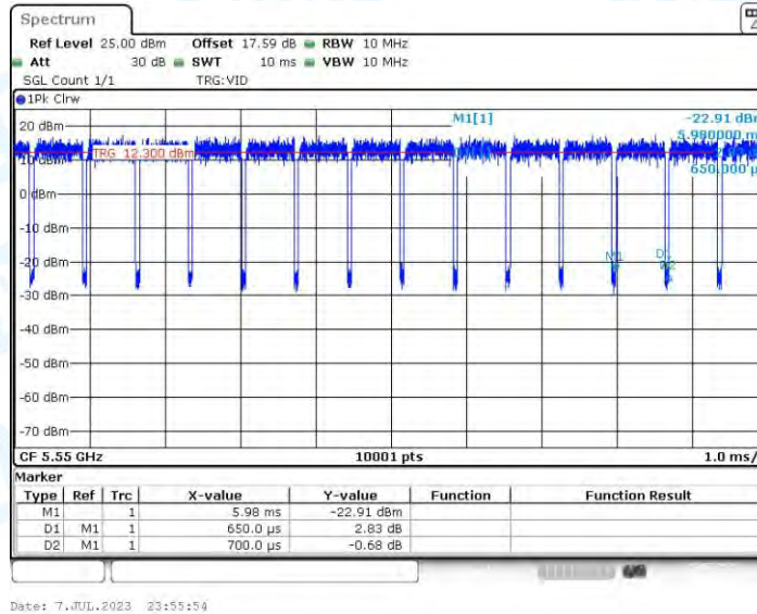
11N40-CDD_Ant4_5550
