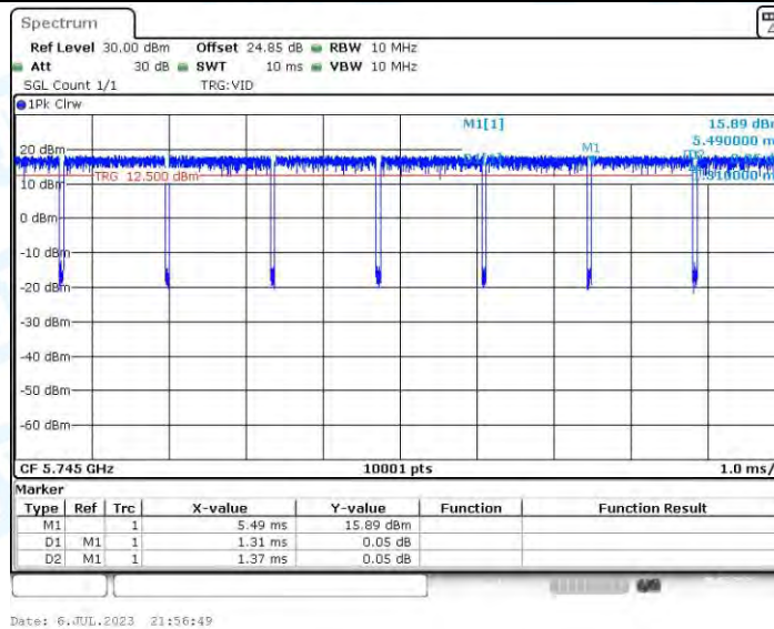
11AC20-CDD_Ant2_5745
