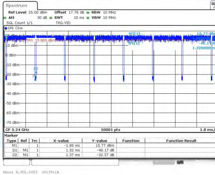
11AC20-CDD_Ant3_5240
