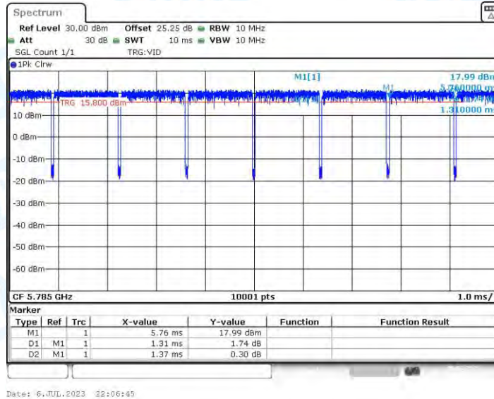
11AC20-CDD_Ant3_5785
