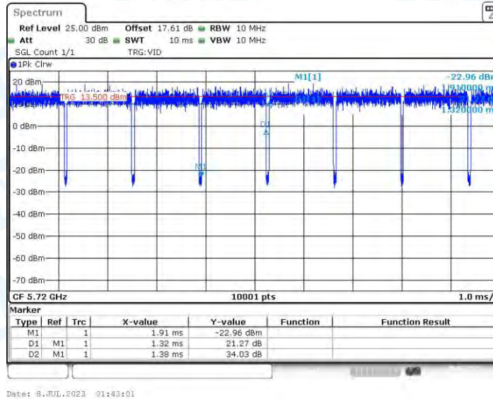
11AC20-CDD_Ant4_5720
