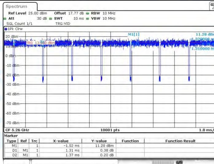
11AC20-CDD_Ant4_5260
