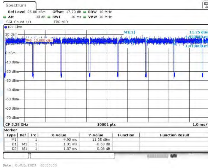
11AC20-CDD_Ant3_5280
