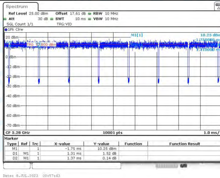
11AC20-CDD_Ant4_5280
