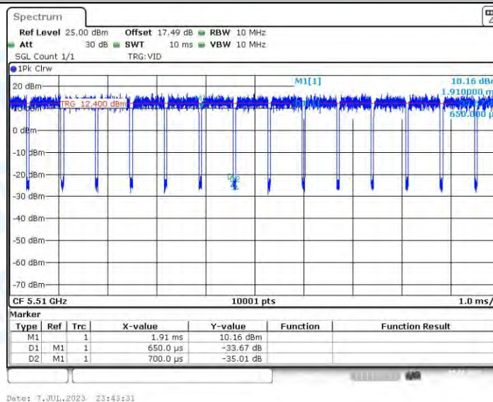
11N40-CDD_Ant4_5510
