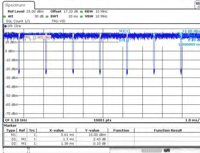
11N20-CDD_Ant4_5180
