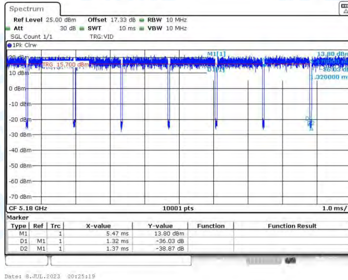
11AC20-CDD_Ant4_5180
