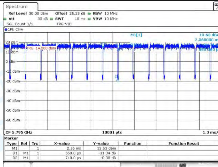
11AC40-CDD_Ant3_5795
