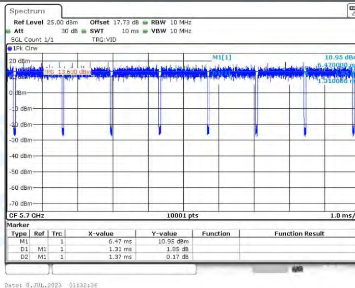
11AC20-CDD_Ant4_5700
