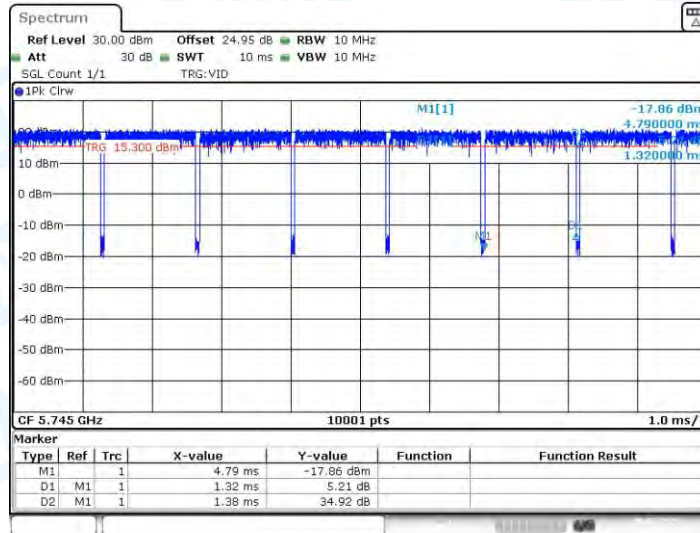
11AC20-CDD_Ant4_5745
