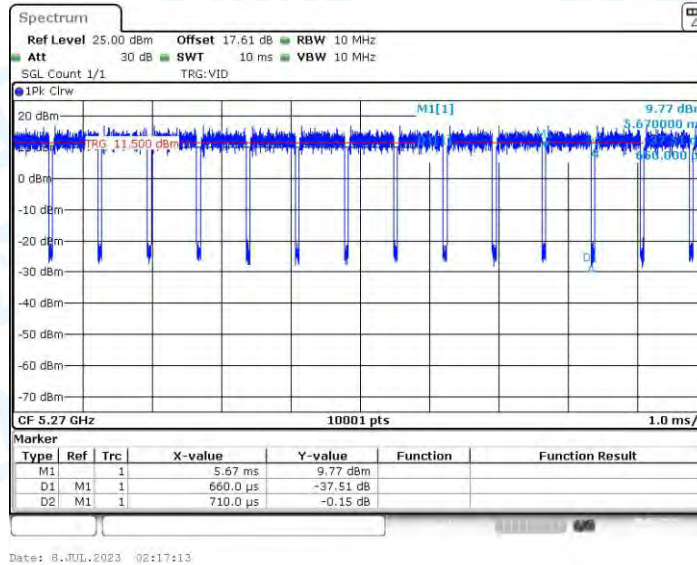
11AC40-CDD_Ant4_5270
