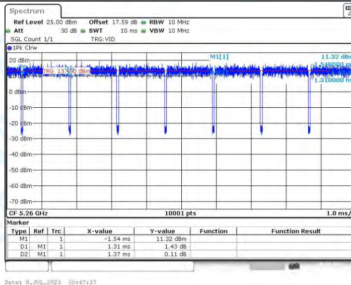
11AC20-CDD_Ant3_5260
