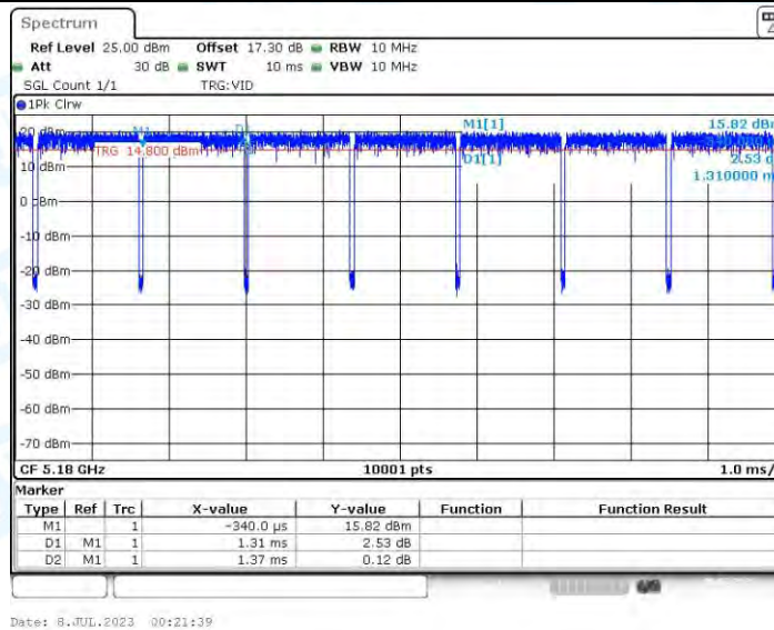
11AC20-CDD_Ant2_5180
