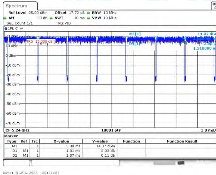
11AC20-CDD_Ant4_5240
