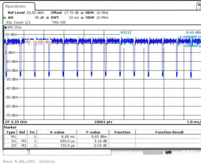
11AC40-CDD_Ant4_5230
