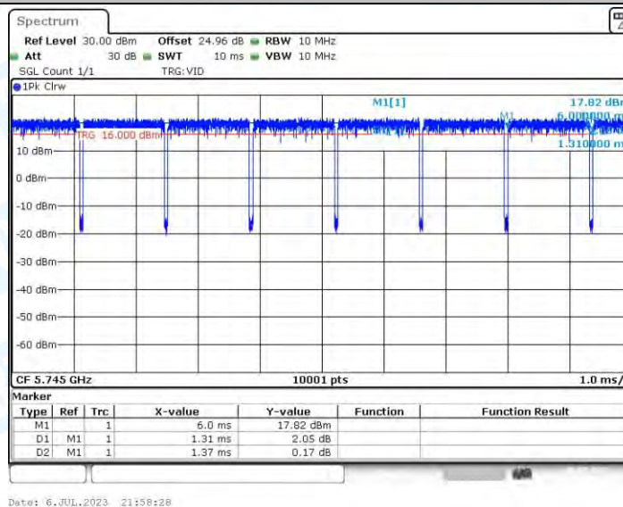
11AC20-CDD_Ant3_5745
