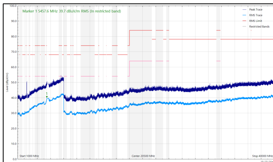
Figure 67 - U-NII-2C - 5640 MHz (CH128), HT20, CDD, Core 0 + Core 1 and 2440 MHz (CH18), Core 0, ePA, 1 GHz to 40 GHz, Horizontal
