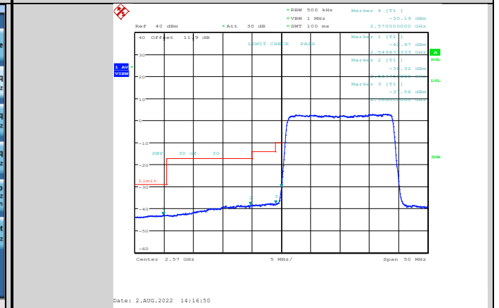
Band38-20MHz-64QAM-37850-100RB#0
