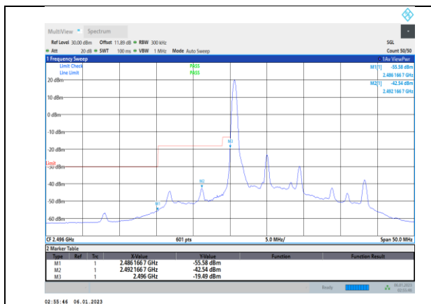
Band41-10MHz-16QAM-39700-50RB#0
