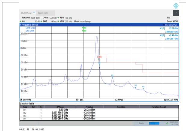
Band41-5MHz-64QAM-41565-25RB#0
