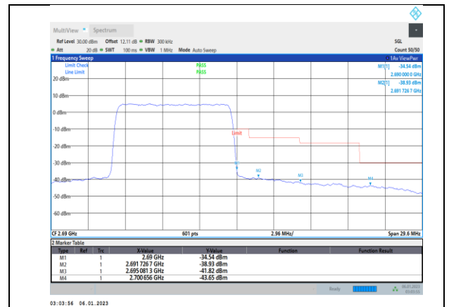
Band41-10MHz-64QAM-39700-1RB#0
