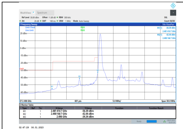
Band41-15MHz-16QAM-39725-75RB#0
