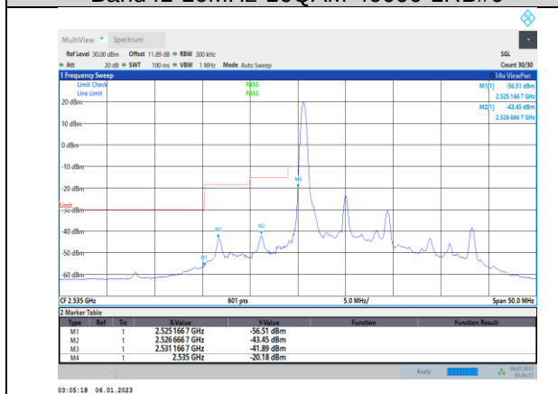
Band41-10MHz-16QAM-40090-50RB#0
