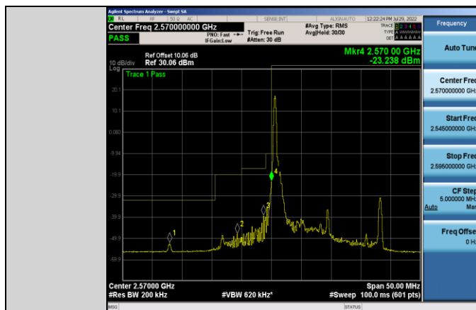
Band38-10MHz-16QAM-37800-1RB#0
