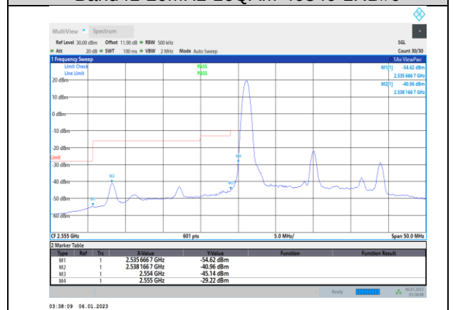
Band41-20MHz-16QAM-40340-100RB#0
