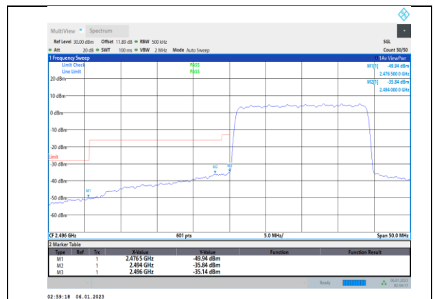
Band41-20MHz-QPSK-40140-1RB#0
