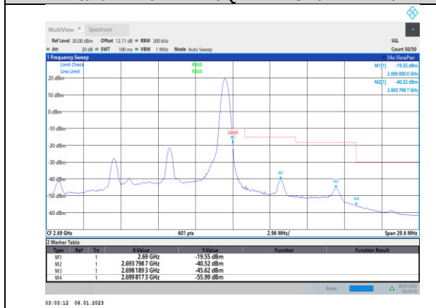
Band41-10MHz-16QAM-41540-50RB#0
