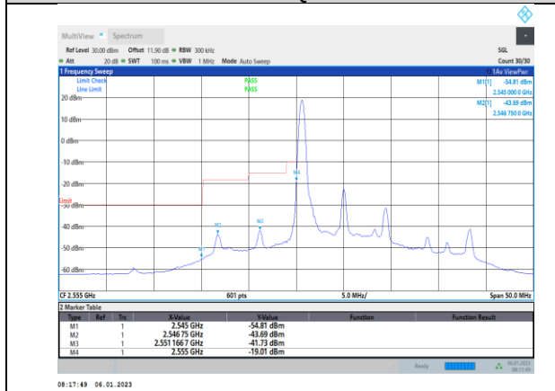
Band41-10MHz-64QAM-40290-50RB#0
