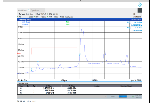
Band41-20MHz-64QAM-39750-100RB#0
