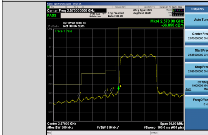
Band38-15MHz-16QAM-37825-75RB#0
