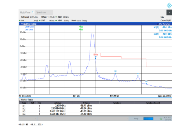
Band41-10MHz-16QAM-41190-50RB#0
