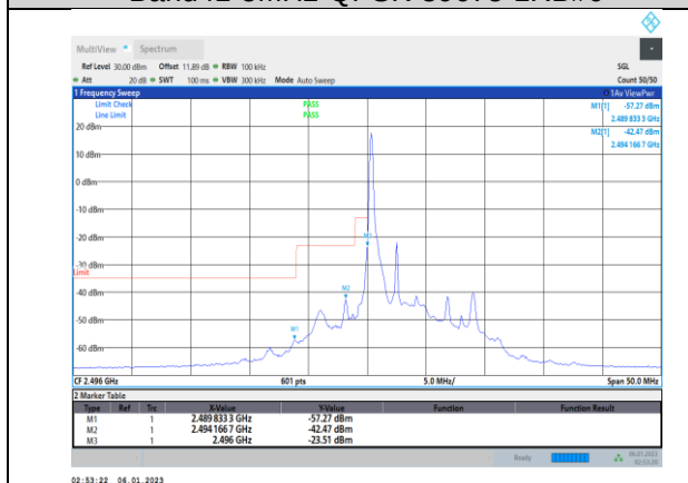
Band41-5MHz-QPSK-39675-25RB#0
