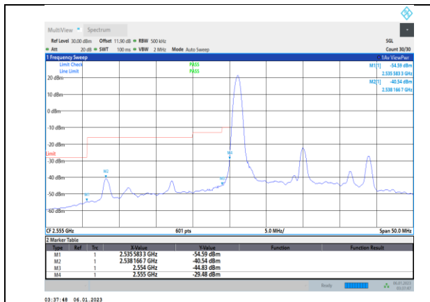
Band41-20MHz-QPSK-40340-100RB#0
