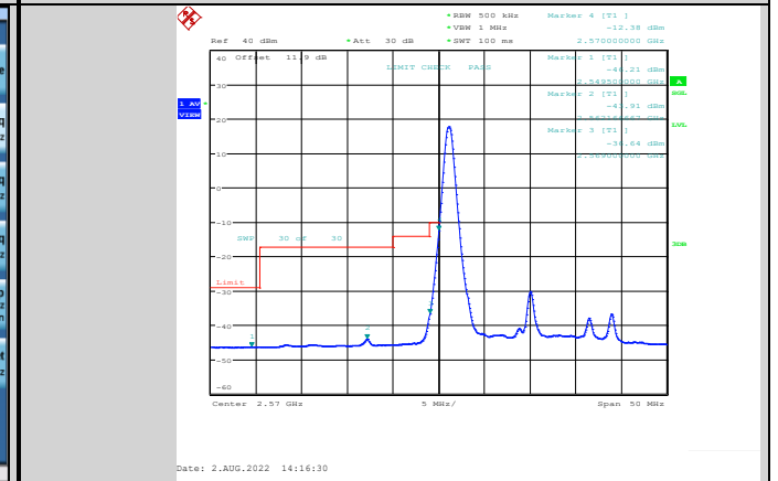
Band38-20MHz-64QAM-37850-1RB#0
