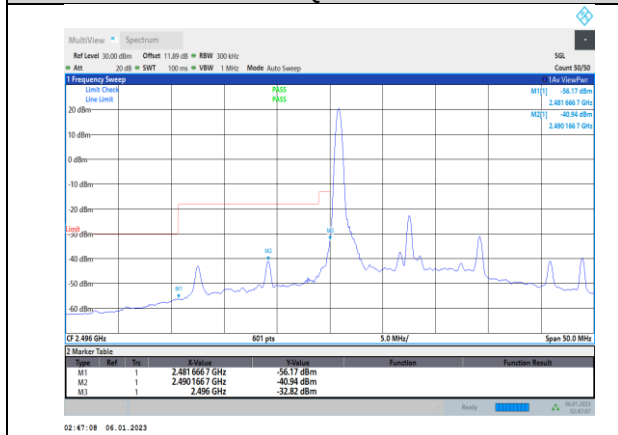
Band41-15MHz-QPSK-39725-75RB#0
