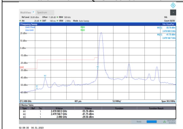
Band41-20MHz-QPSK-39750-100RB#0
