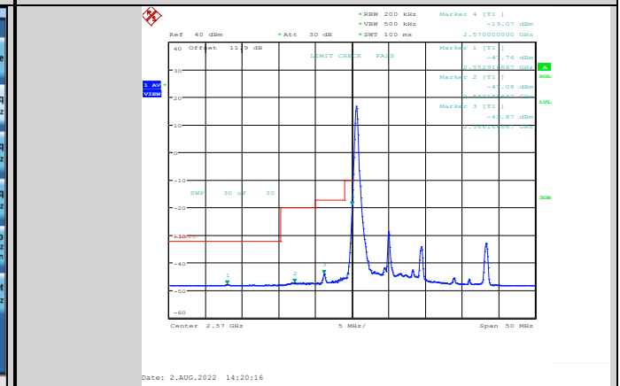
Band38-10MHz-64QAM-37800-1RB#0
