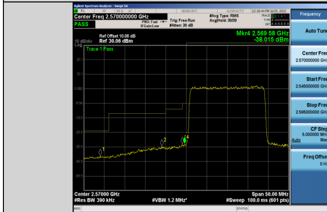
Band38-20MHz-16QAM-37850-100RB#0
