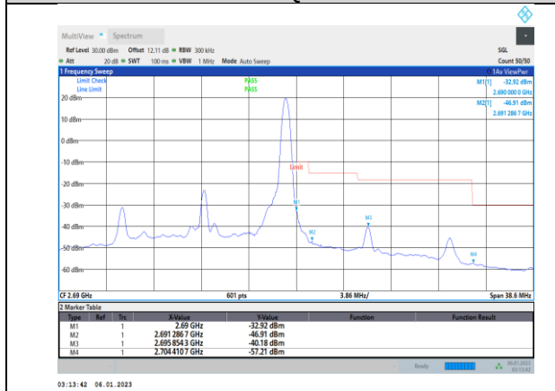
Band41-15MHz-16QAM-41515-75RB#0
