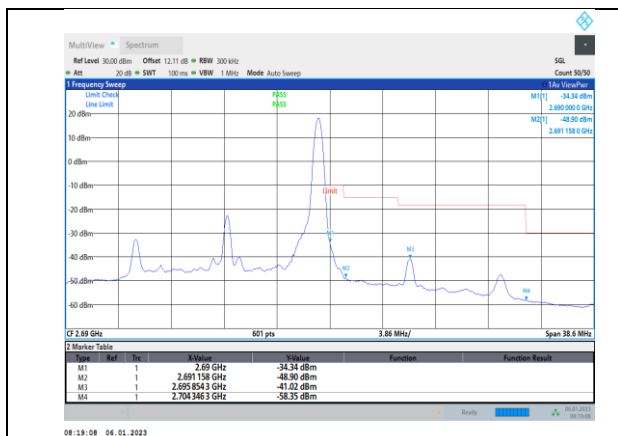
Band41-15MHz-64QAM-41515-75RB#0
