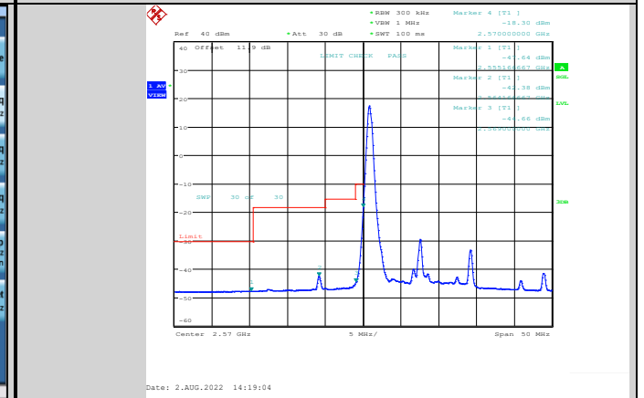
Band38-15MHz-64QAM-37825-1RB#0
