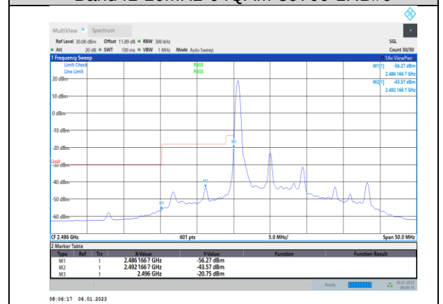
Band41-10MHz-64QAM-39700-50RB#0
