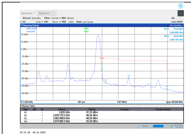
Band41-20MHz-16QAM-41140-100RB#0
