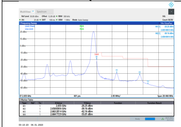
Band41-10MHz-QPSK-41190-50RB#0
