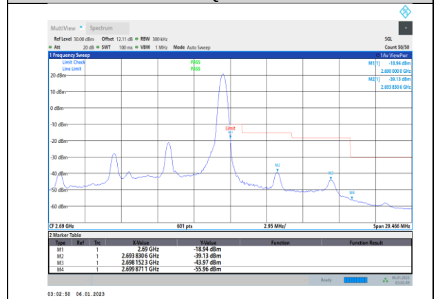
Band41-10MHz-QPSK-41540-50RB#0
