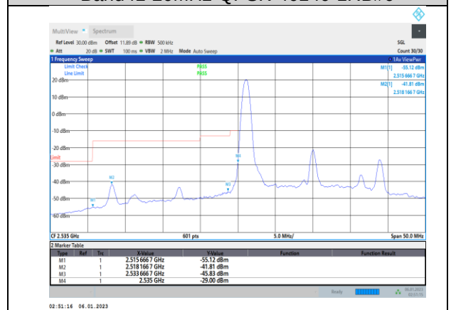
Band41-20MHz-QPSK-40140-100RB#0
