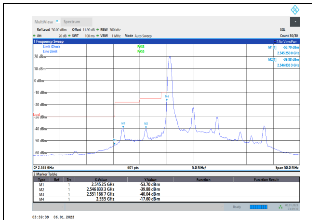
Band41-10MHz-QPSK-40290-50RB#0
