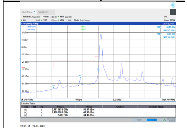
Band41-15MHz-64QAM-39725-75RB#0
