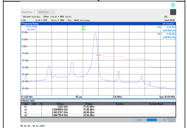
Band41-10MHz-64QAM-41190-50RB#0
