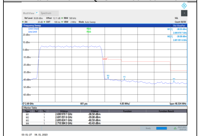
Band41-20MHz-16QAM-39750-1RB#0
