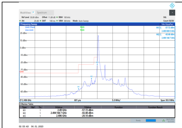
Band41-5MHz-16QAM-39675-25RB#0
