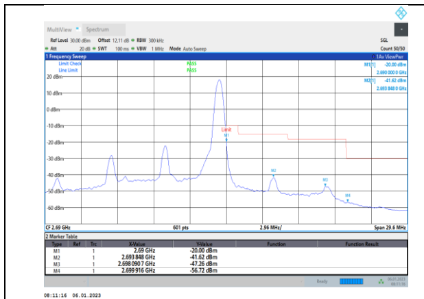
Band41-10MHz-64QAM-41540-50RB#0
