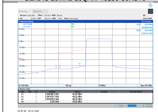
Band41-10MHz-16QAM-41190-1RB#49
