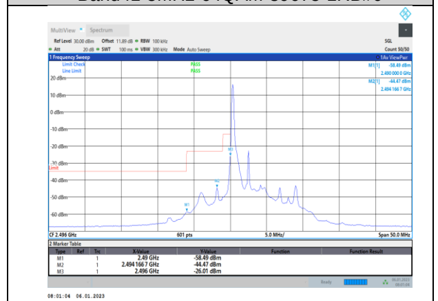
Band41-5MHz-64QAM-39675-25RB#0
