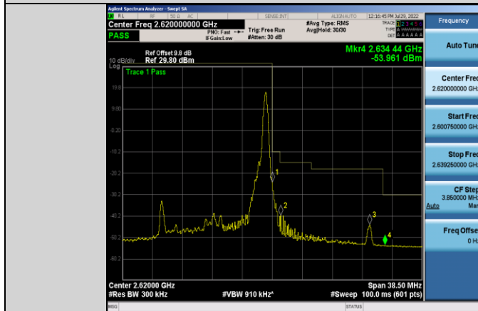
Band38-15MHz-16QAM-38175-1RB#74
