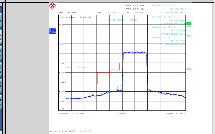
Band38-10MHz-64QAM-37800-50RB#0
