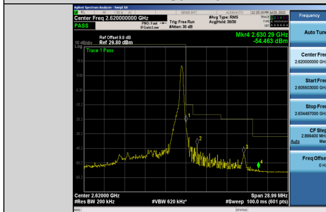
Band38-10MHz-16QAM-38200-1RB#49
