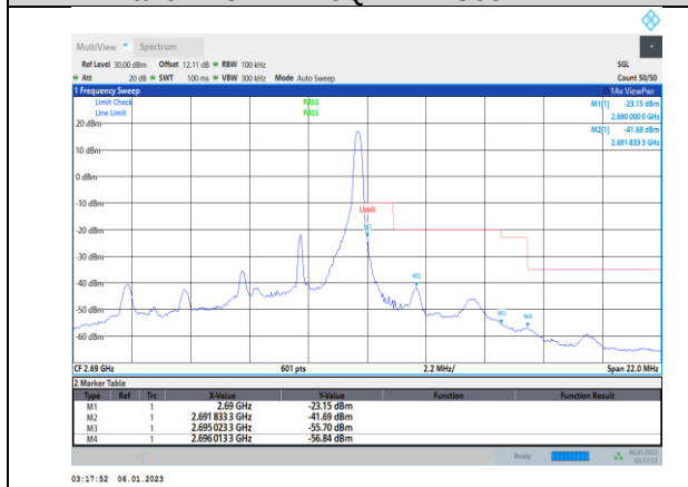
Band41-5MHz-16QAM-41565-25RB#0
