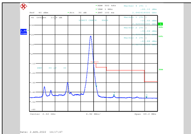
Band38-20MHz-64QAM-38150-1RB#99
