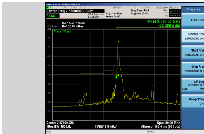
Band38-15MHz-16QAM-37825-1RB#0
