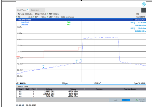
Band41-15MHz-16QAM-41515-1RB#74
