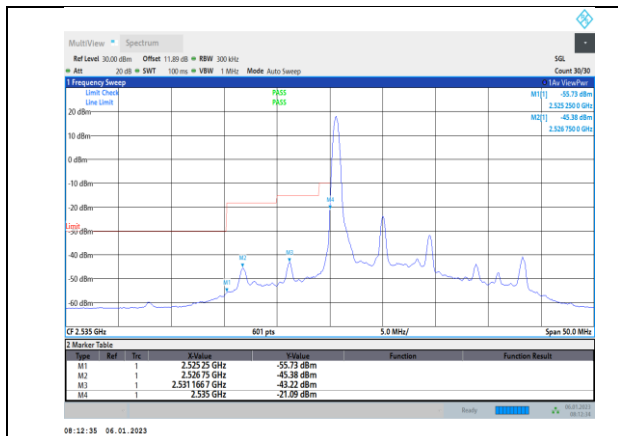
Band41-10MHz-64QAM-40090-50RB#0
