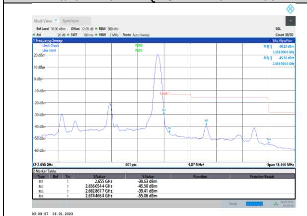
Band41-20MHz-QPSK-41140-100RB#0
