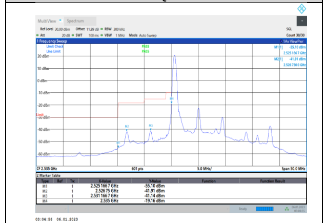
Band41-10MHz-QPSK-40090-50RB#0
