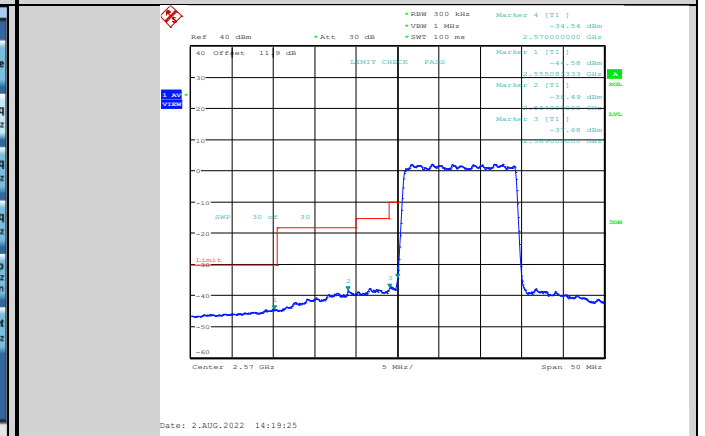
Band38-15MHz-64QAM-37825-75RB#0
