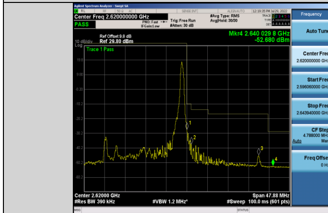
Band38-20MHz-16QAM-38150-1RB#99
