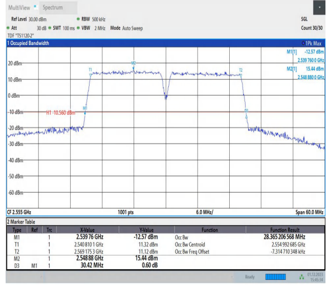
7-7-15MHz-15MHz-QPSK-QPSK-21225-21375-75RB#0-75RB #0-PASS
