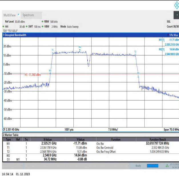
7-7-15MHz-20MHz-16QAM-16QAM-21179-21350-75RB#0-100 RB#0-PASS
