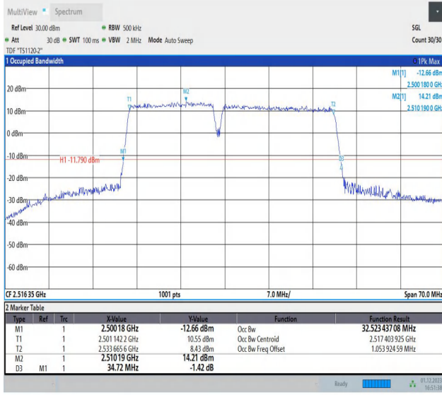
7-7-15MHz-20MHz-16QAM-16QAM-20828-20999-75RB#0-10 ORB#0-PASS
