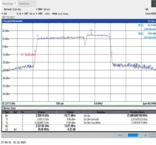
7-7-20MHz-10MHz-16QAM-16QAM-20850-20994-100RB#0-5 ORB#0-PASS
