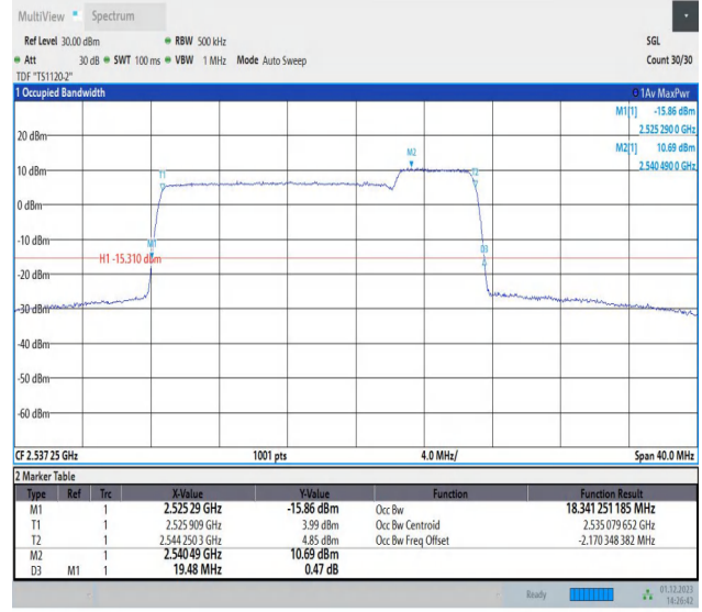
7-7-15MHz-5MHz-64QAM-64QAM-21076-21169-75RB#0-25R B#0-PASS
