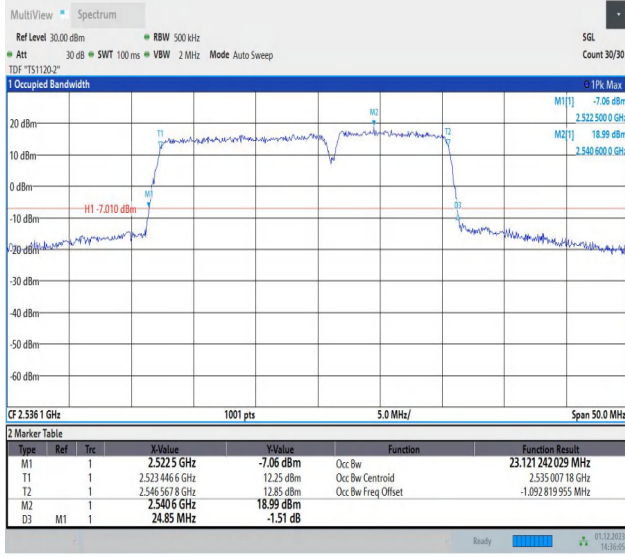
7-7-15MHz-10MHz-16QAM-16QAM-21051-21171-75RB#0-50 RB#0-PASS
