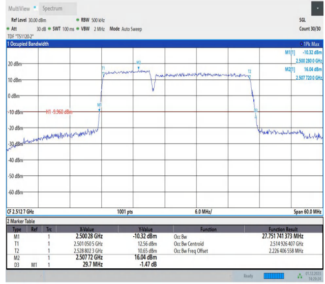
7-7-10MHz-20MHz-QPSK-QPSK-20805-20949-50RB#0-100R B#0-PASS
