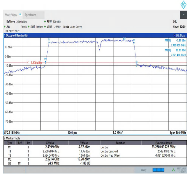
7-7-15MHz-10MHz-QPSK-QPSK-21277-21397-75RB#0-50RB #0-PASS
