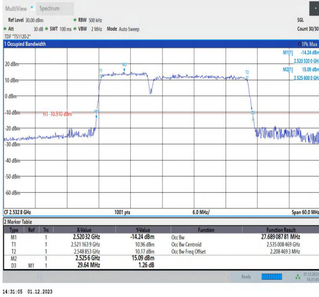
7-7-10MHz-20MHz-16QAM-16QAM-21006-21150-50RB#0-100 RB#0-PASS
