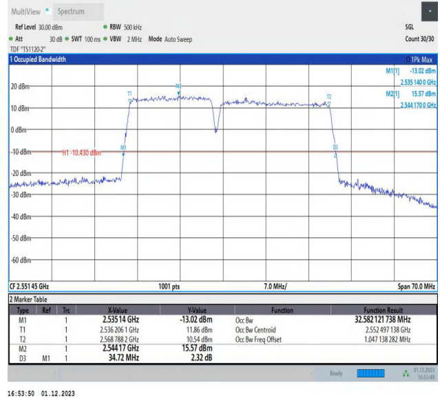
7-7-15MHz-20MHz-QPSK-QPSK-21179-21350-75RB#0-100R B#0-PASS
