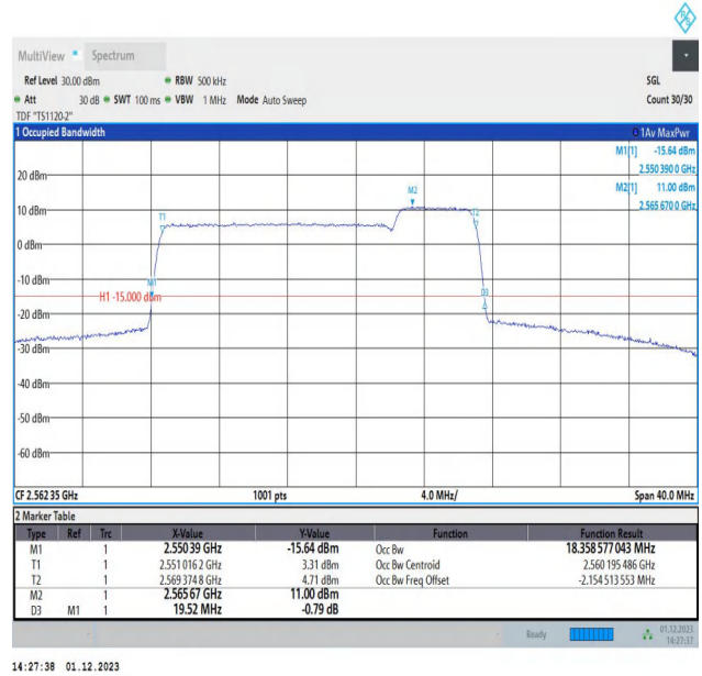
7-7-15MHz-5MHz-16QAM-16QAM-21327-21420-75RB#0-25R B#0-PASS
