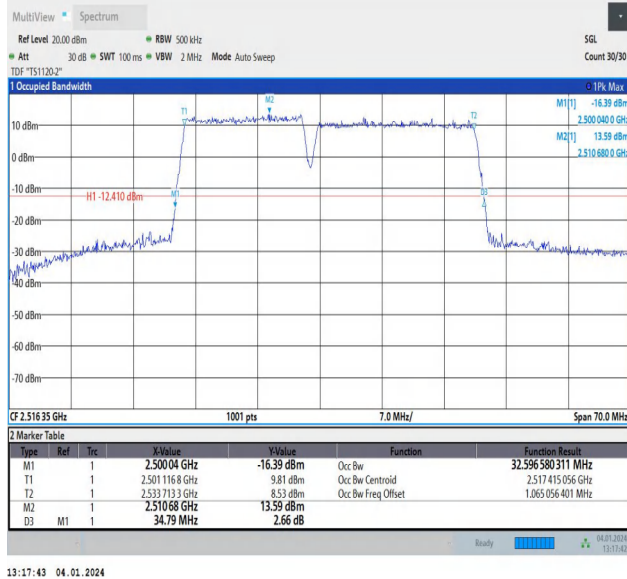
7-7-15MHz-20MHz-64QAM-64QAM-20828-20999-75RB#0-10 ORB#0-PASS
