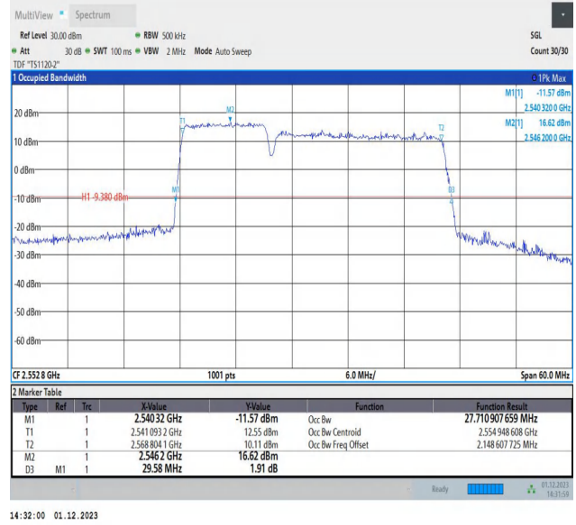
7-7-10MHz-20MHz-QPSK-QPSK-21206-21350-50RB#0-100R B#0-PASS
