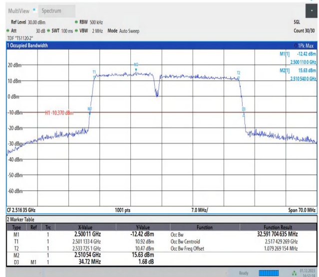
7-7-15MHz-20MHz-QPSK-QPSK-20828-20999-75RB#0-100R B#0-PASS
