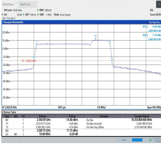
7-7-15MHz-5MHz-64QAM-64QAM-21327-21420-75RB#0-25R B#0-PASS
