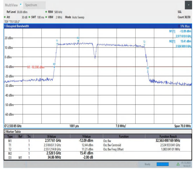
7-7-15MHz-20MHz-QPSK-QPSK-21003-21174-75RB#0-100R B#0-PASS
