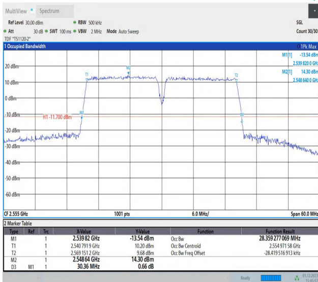
7-7-15MHz-15MHz-16QAM-16QAM-21225-21375-75RB#0-75 RB#0-PASS
