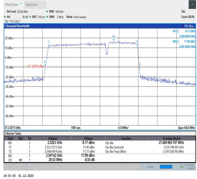
7-7-20MHz-10MHz-QPSK-QPSK-21051-21195-100RB#0-50R B#0-PASS
