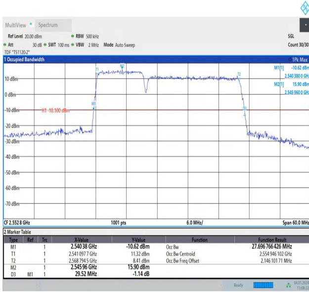
7-7-15MHz-10MHz-16QAM-16QAM-21051-21171-75RB#0-50 RB#0-PASS
