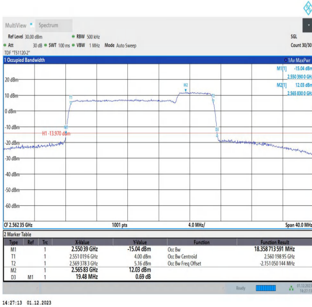
7-7-15MHz-5MHz-QPSK-QPSK-21327-21420-75RB#0-25RB#0-PASS
