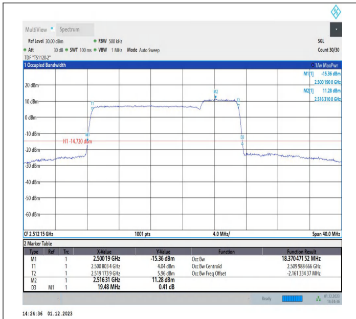
7-7-15MHz-5MHz-QPSK-QPSK-20825-20918-75RB#0-25RB#0-PASS
