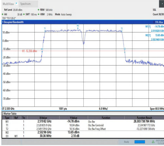
7-7-15MHz-15MHz-64QAM-64QAM-21025-21175-75RB#0-75 RB#0-PASS
