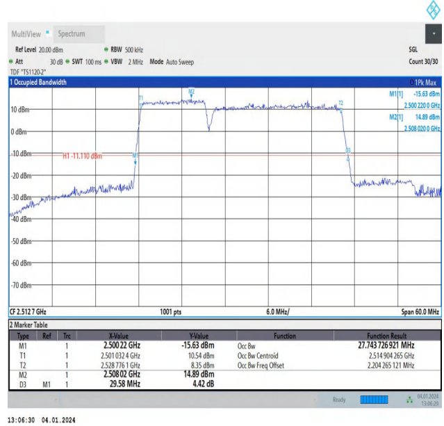
7-7-10MHz-20MHz-64QAM-64QAM-20805-20949-50RB#0-10 0RB#0-PASS
