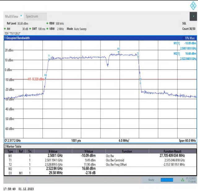
7-7-20MHz-10MHz-QPSK-QPSK-20850-20994-100RB#0-50R B#0-PASS
