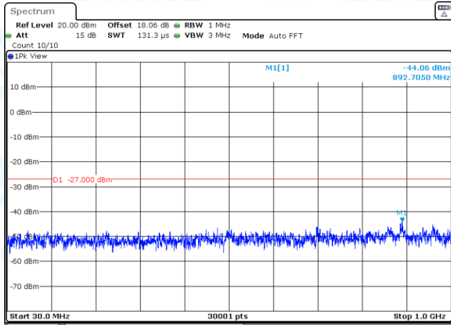
11A-Ant3-5500-30~1000-PASS
