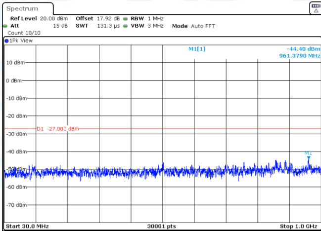
11AC40SISO-Ant3-5230-30~1000-PASS
