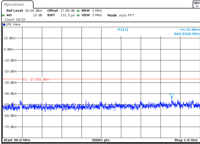
11AC40SISO-Ant3-5190-30~1000-PASS
