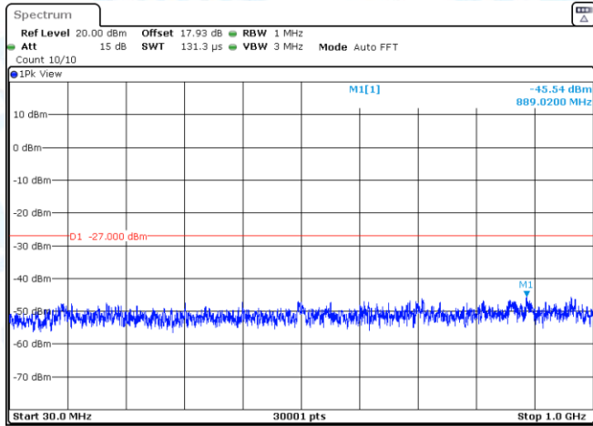
11N40SISO-Ant3-5310-30~1000-PASS
