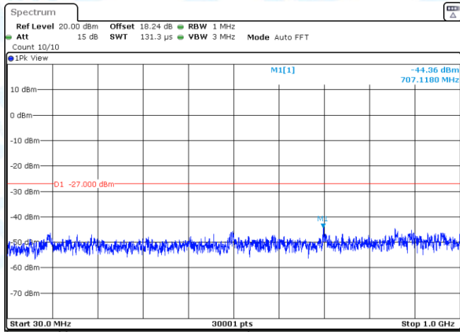
11N20SISO-Ant3-5785-30~1000-PASS
