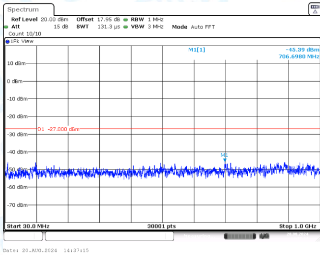
11A-Ant3-5180-30~1000-PASS
