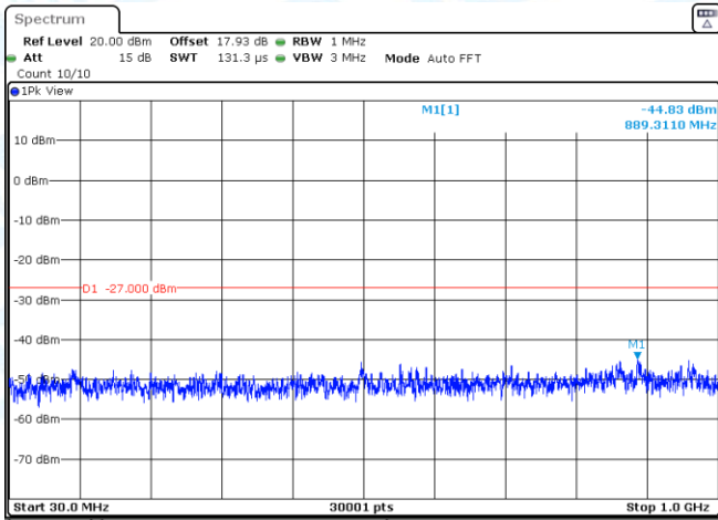
11AC20SISO-Ant3-5280-30~1000-PASS
