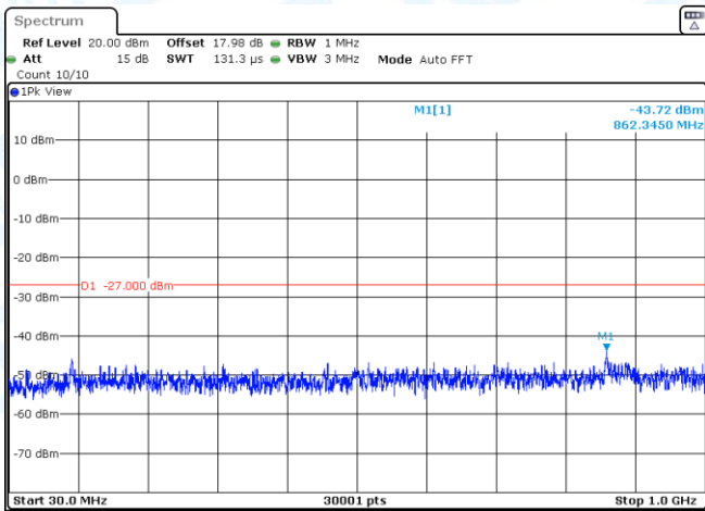
11AC20SISO-Ant3-5200-30~1000-PASS
