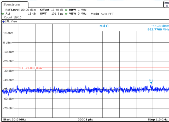
11N20SISO-Ant3-5580-30~1000-PASS
