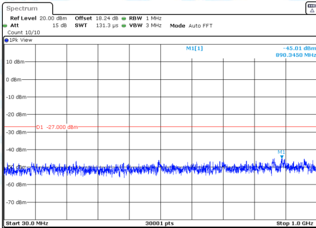
11AC20SISO-Ant3-5785-30~1000-PASS
