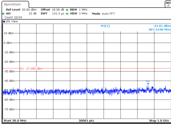
11AC20SISO-Ant3-5500-30~1000-PASS
