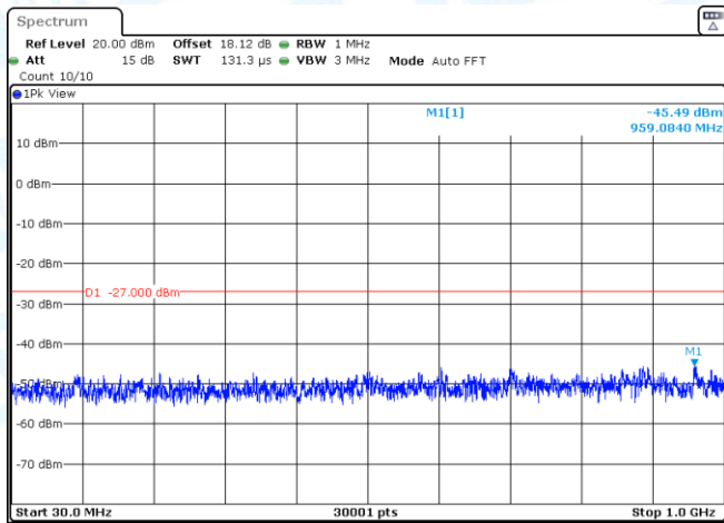
11N40SISO-Ant3-5510-30~1000-PASS
