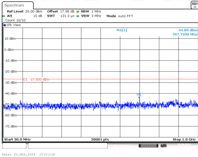
11A-Ant3-5240-30~1000-PASS
