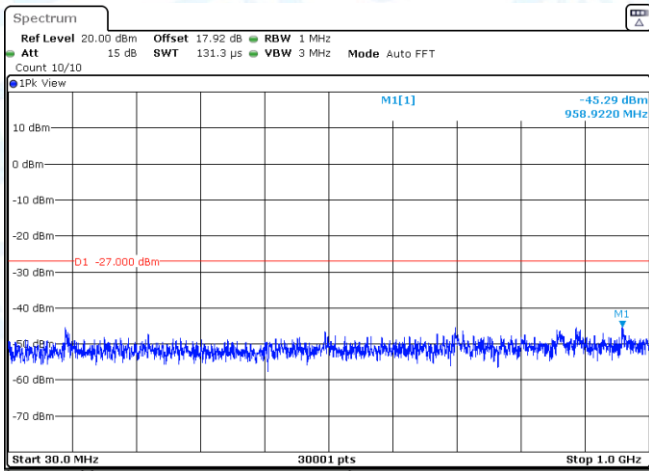
11AC20SISO-Ant3-5260-30~1000-PASS
