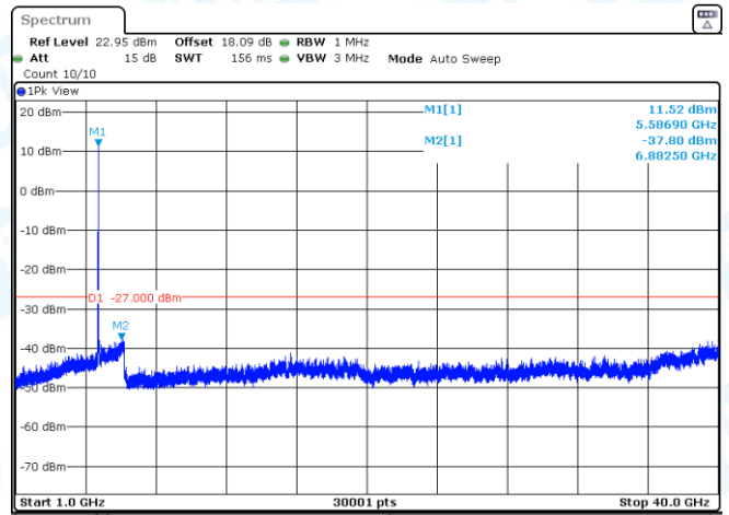
11A-Ant3-5500-1000~40000-PASS
