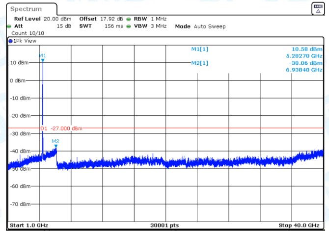
11N20SISO-Ant3-5260-1000~40000-PASS
