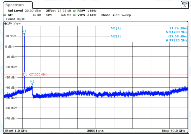
11AC20SISO-Ant3-5280-1000~40000-PASS
