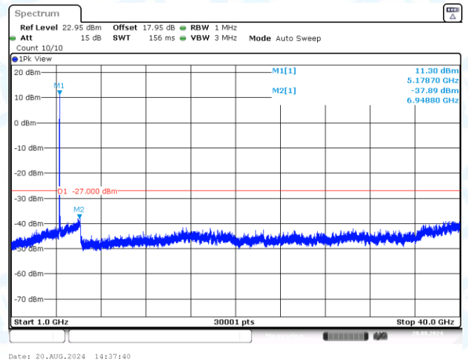
11A-Ant3-5180-1000~40000-PASS
