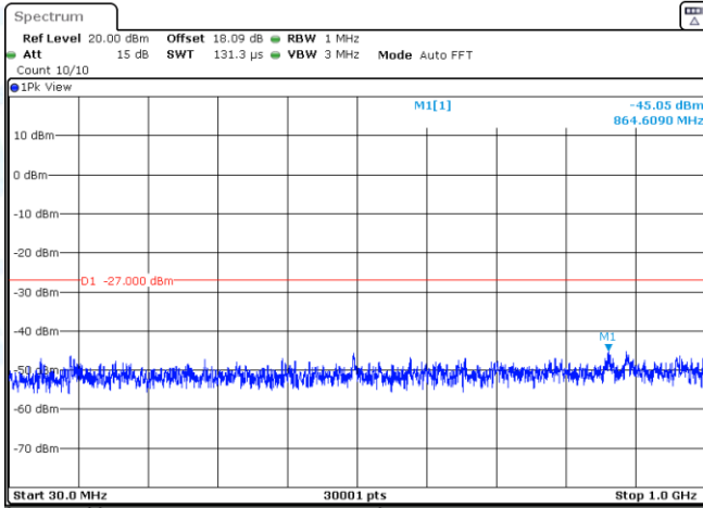
11N20SISO-Ant3-5500-30~1000-PASS
