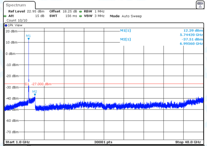
11A-Ant3-5745-1000~40000-PASS
