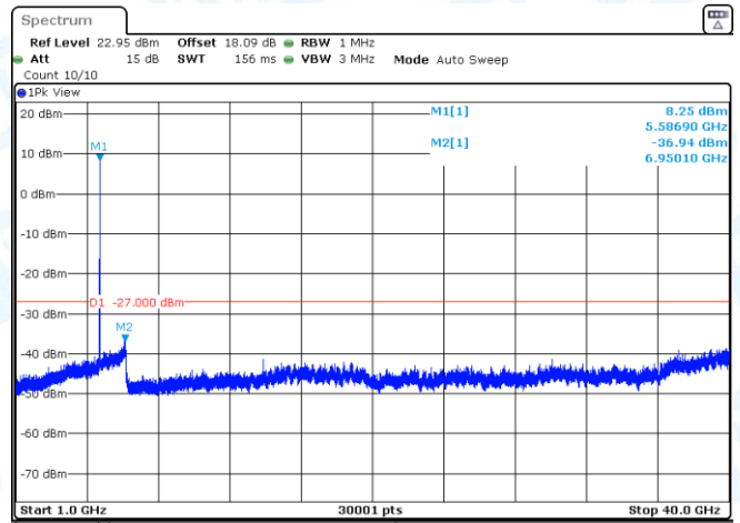
11AC20SISO-Ant3-5500-1000~40000-PASS
