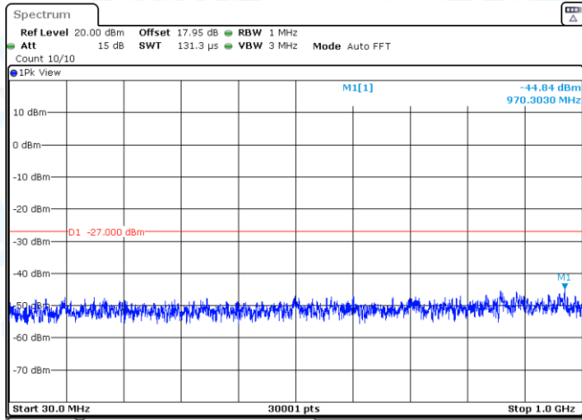
11N20SISO-Ant3-5180-30~1000-PASS
