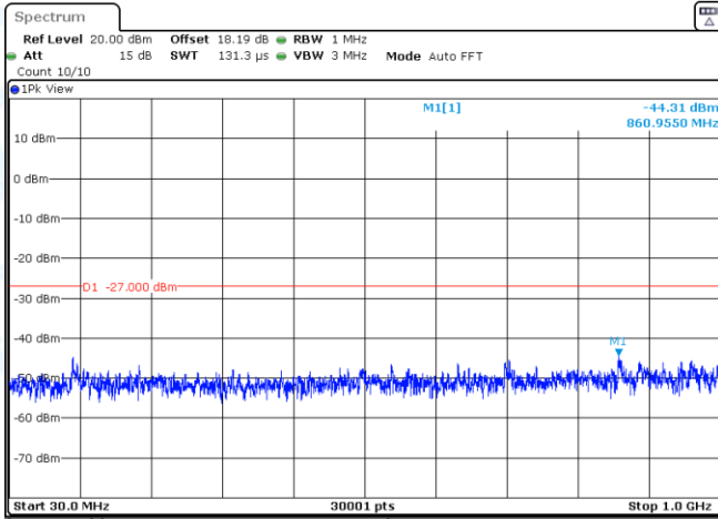
11AC20SISO-Ant3-5745-30~1000-PASS
