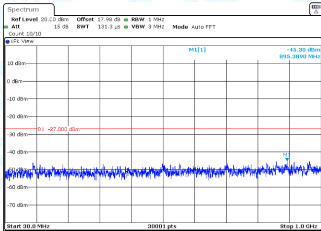
11N20SISO-Ant3-5200-30~1000-PASS
