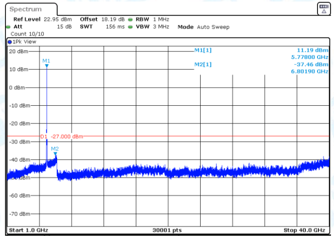
11N20SISO-Ant3-5745-1000~40000-PASS
