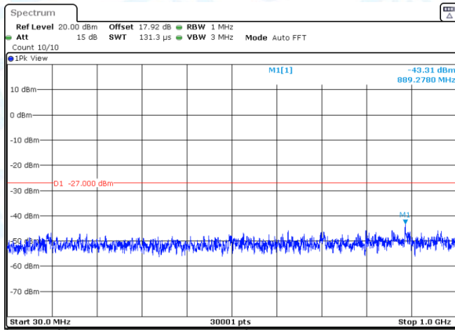
11N20SISO-Ant3-5260-30~1000-PASS
