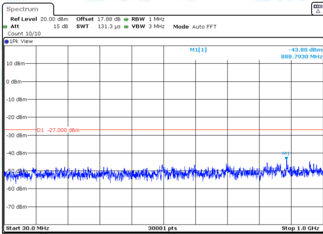
11AC20SISO-Ant3-5180-30~1000-PASS
