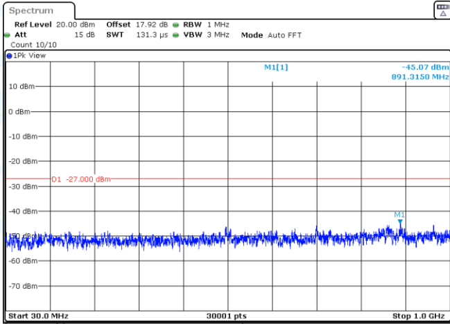
11A-Ant3-5260-30~1000-PASS
