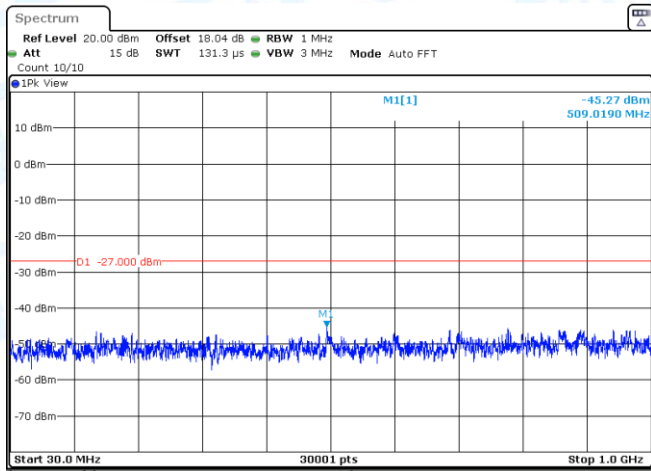
11N40SISO-Ant3-5310-30~1000-PASS
