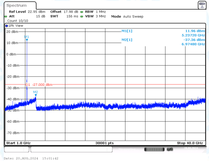
11A-Ant3-5240-1000~40000-PASS
