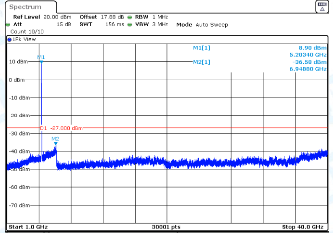
11AC40SISO-Ant3-5190-1000~40000-PASS
