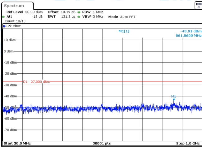
11A-Ant3-5745-30~1000-PASS
