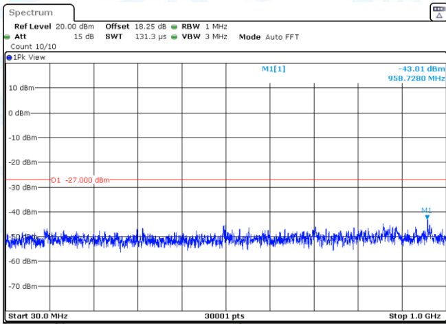
11N40SISO-Ant3-5670-30~1000-PASS
