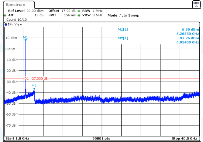
11N40SISO-Ant3-5230-1000~40000-PASS
