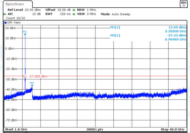
11N20SISO-Ant3-5500-1000~40000-PASS
