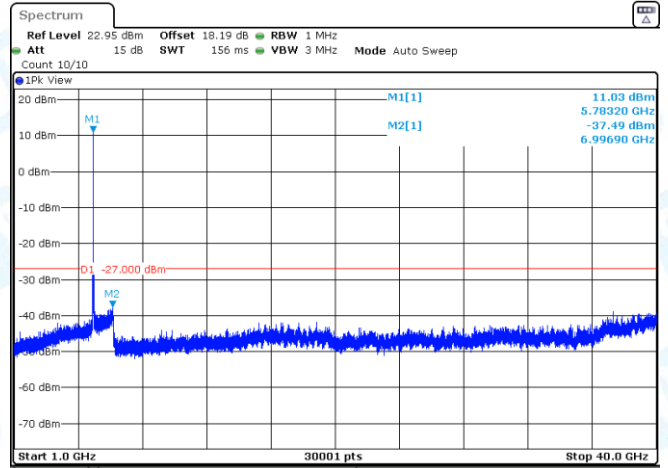
11AC20SISO-Ant3-5745-1000~40000-PASS
