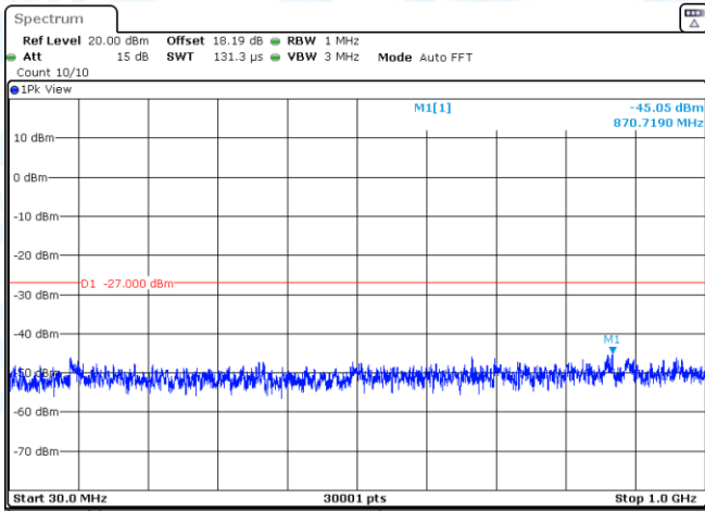
11N40SISO-Ant3-5755-30~1000-PASS
