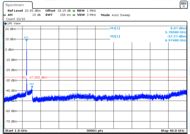
11N40SISO-Ant3-5755-1000~40000-PASS
