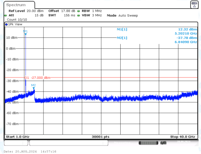
11A-Ant3-5200-1000~40000-PASS
