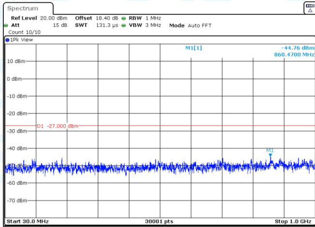
11AC20SISO-Ant3-5580-30~1000-PASS
