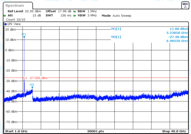
11N20SISO-Ant3-5200-1000~40000-PASS
