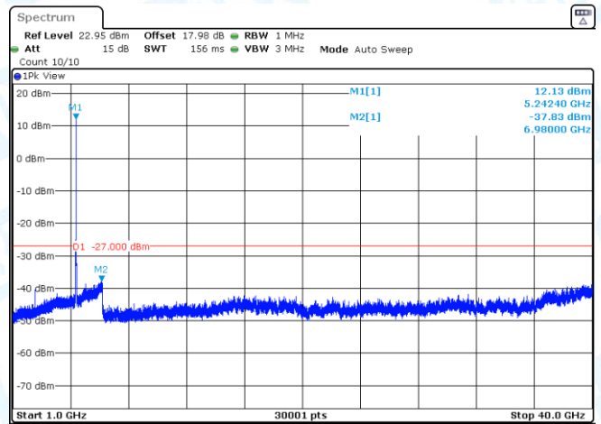
11AC20SISO-Ant3-5200-1000~40000-PASS
