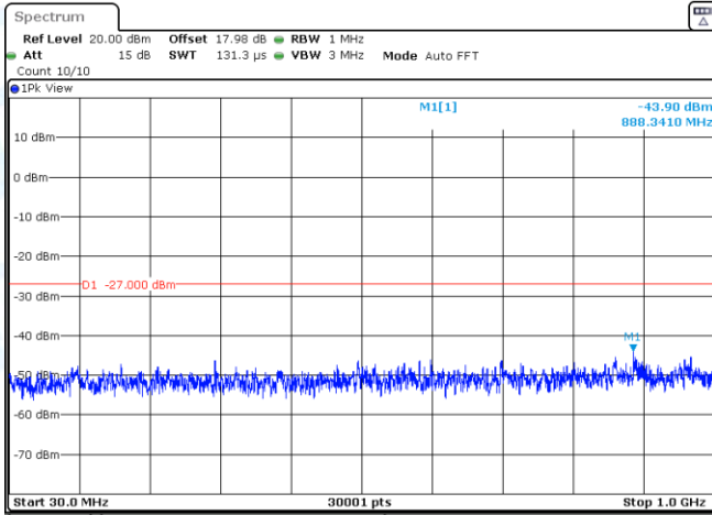
11N40SISO-Ant3-5190-30~1000-PASS
