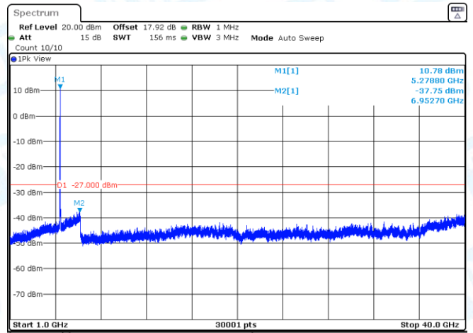
11AC20SISO-Ant3-5260-1000~40000-PASS
