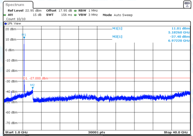
11AC20SISO-Ant3-5180-1000~40000-PASS
