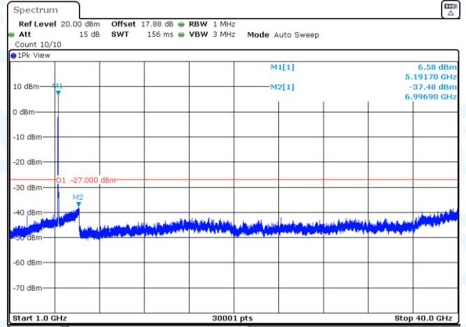
11N40SISO-Ant3-5190-1000~40000-PASS
