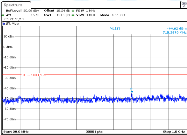
11A-Ant3-5785-30~1000-PASS
