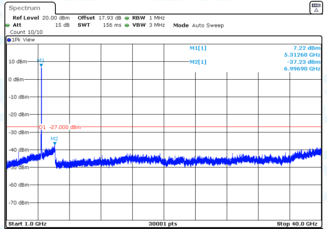
11N40SISO-Ant3-5310-1000~40000-PASS
