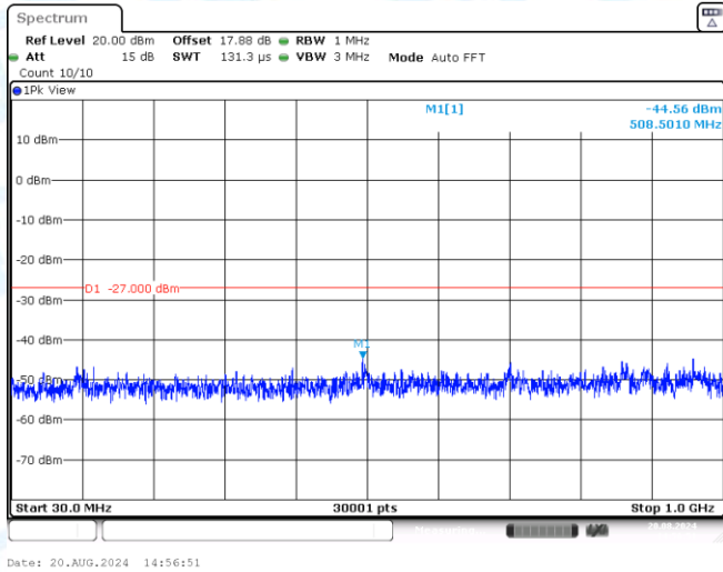
11A-Ant3-5200-30~1000-PASS
