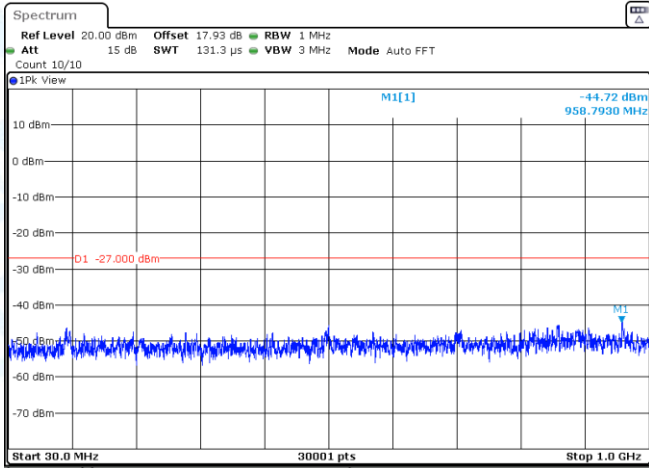
11A-Ant3-5280-30~1000-PASS
