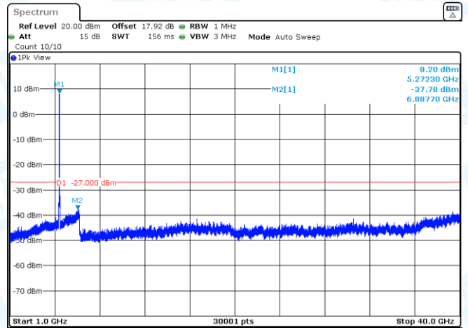
11AC40SISO-Ant3-5230-1000~40000-PASS
