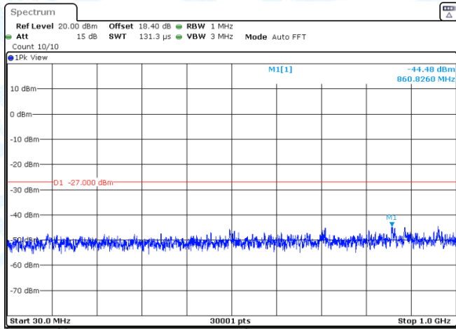
11A-Ant3-5580-30~1000-PASS
