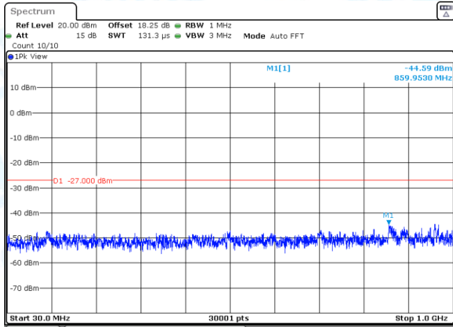
11N20SISO-Ant3-5745-30~1000-PASS
