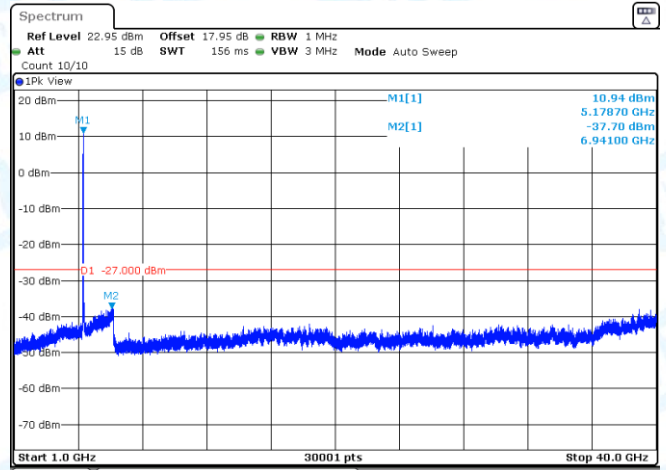
11N20SISO-Ant3-5180-1000~40000-PASS
