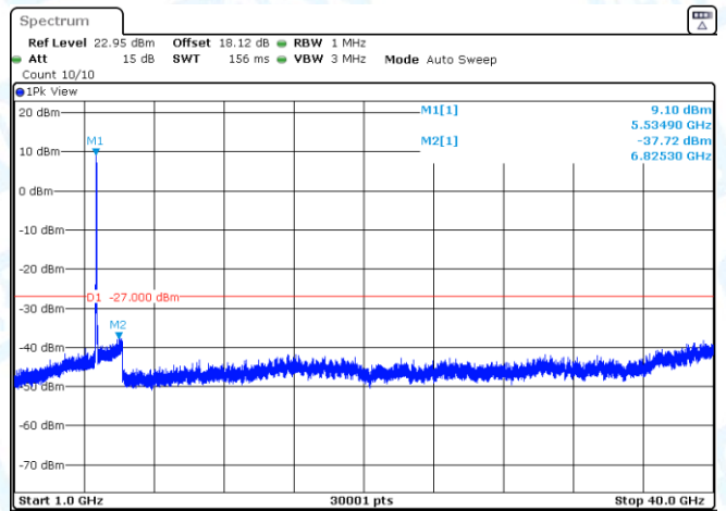
11N40SISO-Ant3-5510-1000~40000-PASS
