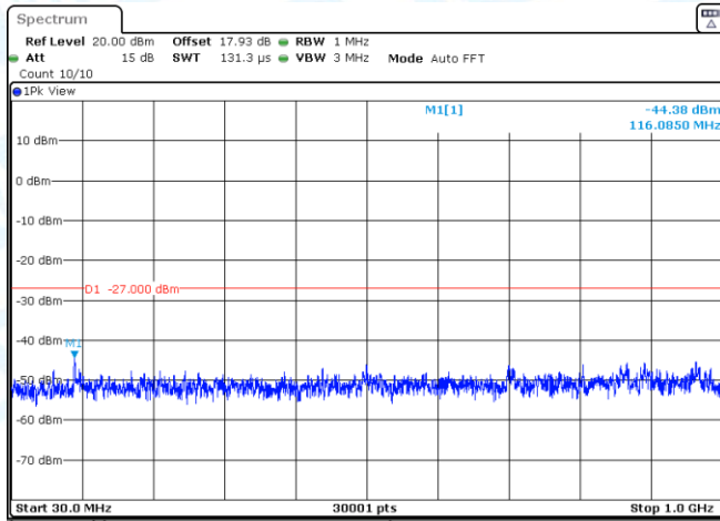
11N20SISO-Ant3-5280-30~1000-PASS
