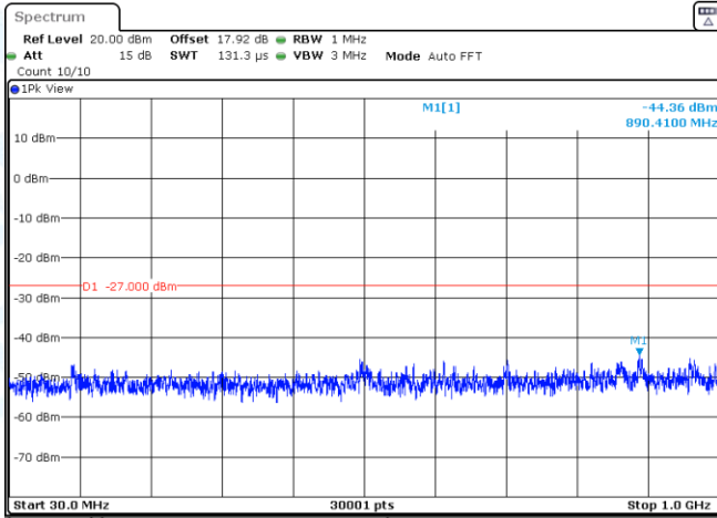
11N40SISO-Ant3-5230-30~1000-PASS
