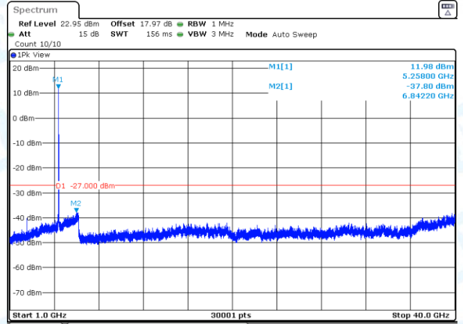
11A-Ant3-5260-1000~40000-PASS
