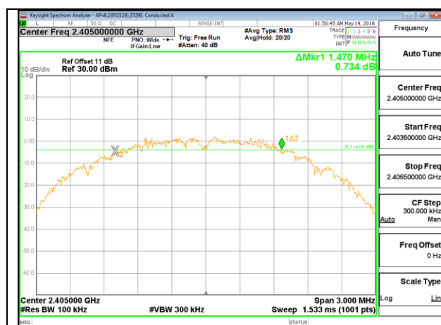
LOW CHANNEL 11
