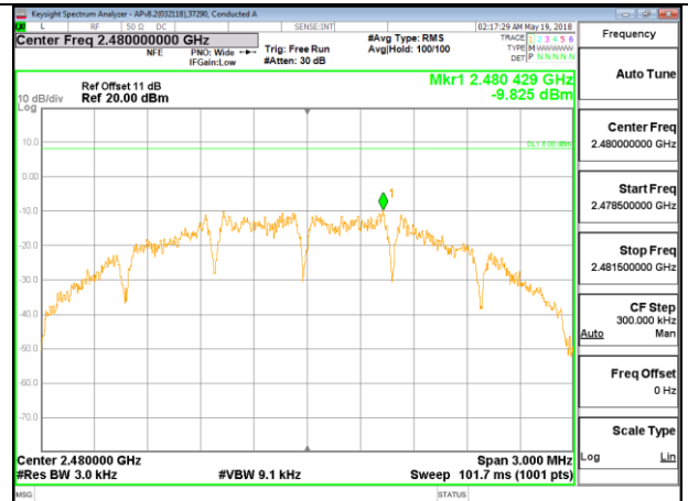
HIGH CHANNEL 26
