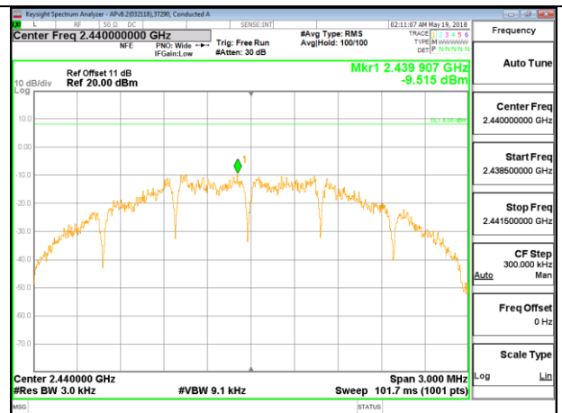
MID CHANNEL 18
