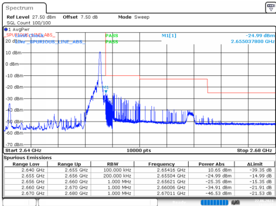
2_15MHz_High_QPSK_1@74
