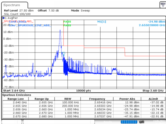
2_15MHz_High_16QAM_1@74
