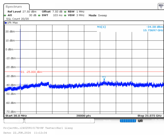
15MHz_High_QPSK_1@0
