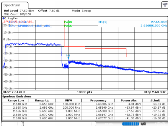
2_15MHz_High_16QAM_75@0
