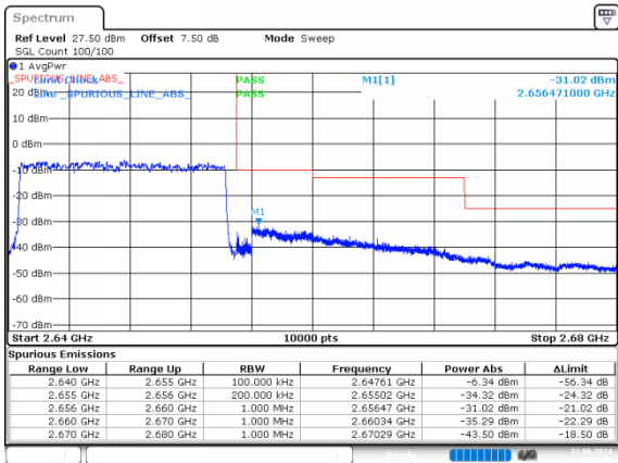
2_15MHz_High_QPSK_75@0
