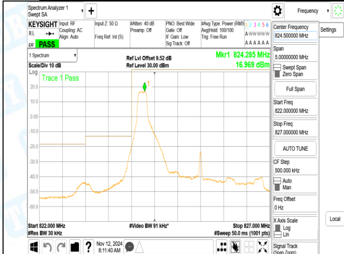
Band5_3MHz_16QAM_20415_15RB#0
