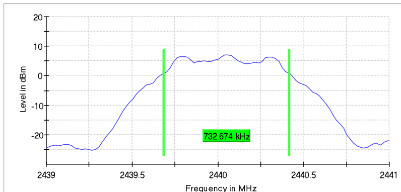
6 dB Bandwidth
