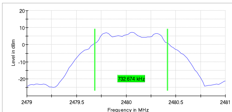
6 dB Bandwidth
