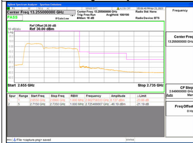
41C / 10+20MHz / High CH / QPSK / 50#0-100#0
