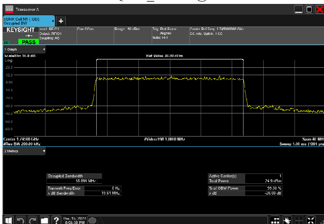
n66_20MHz_15kHz_1745MHz_CP-OFDM 64 QAM_RB106@0
