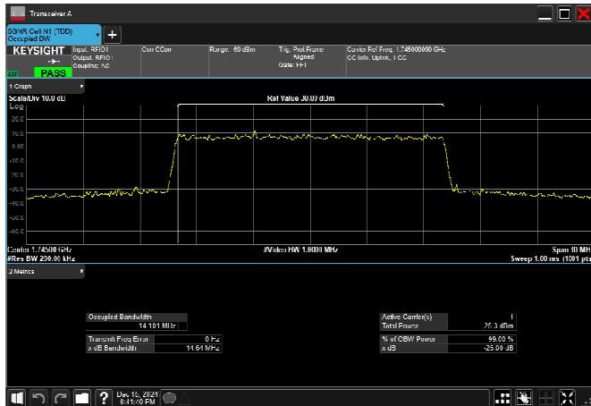
n66_15MHz_15kHz_1745MHz_CP-OFDM 256 QAM_RB79@0
