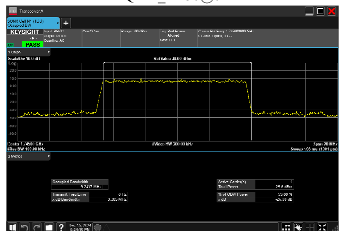
n66_10MHz_15kHz_1745MHz_DFT-s-OFDM 16 QAM_RB50@0
