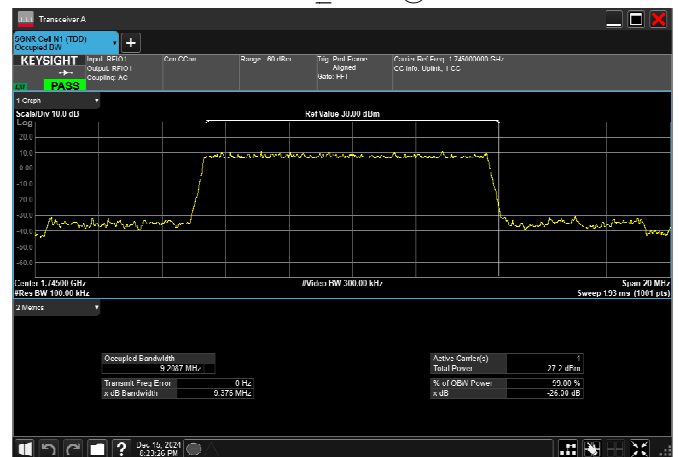
n66_10MHz_15kHz_1745MHz_DFT-s-OFDM 16 QAM_RB50@0
