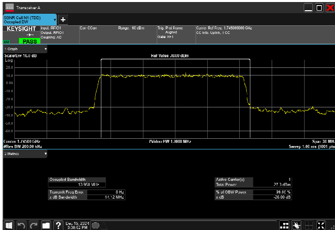
n66_15MHz_15kHz_1745MHz_DFT-s-OFDM 16 QAM_RB75@0
