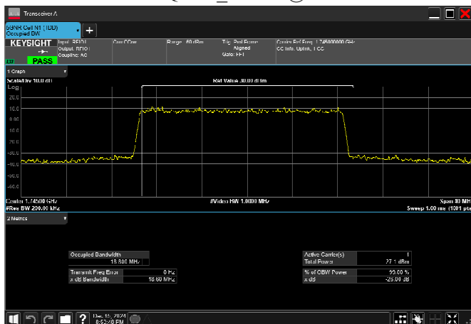
n66_20MHz_15kHz_1745MHz_DFT-s-OFDM QPSK_RB100@0
