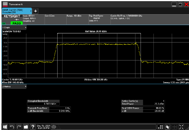
n66_10MHz_15kHz_1745MHz_CP-OFDM QPSK_RB52@0
