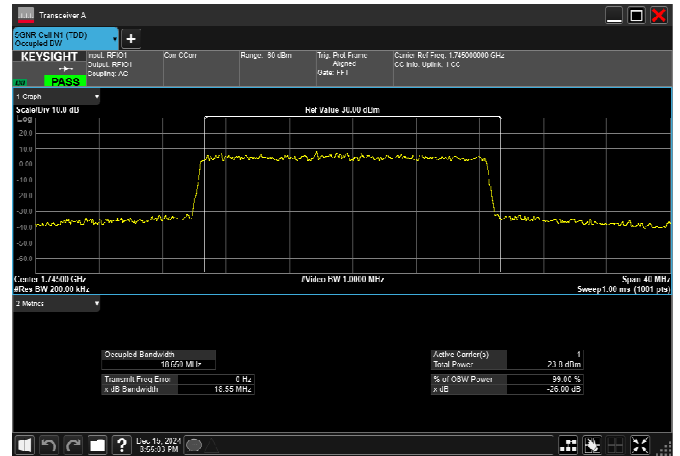
n66_20MHz_15kHz_1745MHz_CP-OFDM 16 QAM_RB106@0
