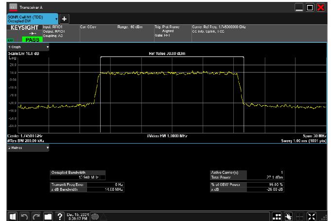
n66_15MHz_15kHz_1745MHz_DFT-s-OFDM 64 QAM_RB75@0
