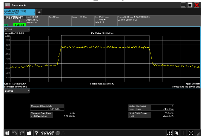
n66_10MHz_15kHz_1745MHz_CP-OFDM 256 QAM_RB52@0
