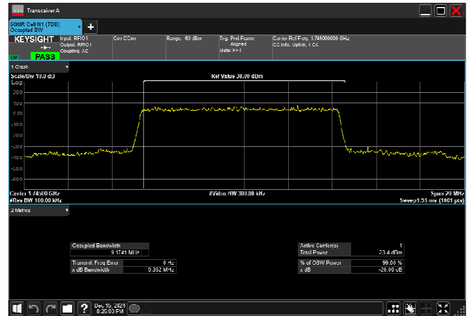
n66_10MHz_15kHz_1745MHz_CP-OFDM 16 QAM_RB52@0
