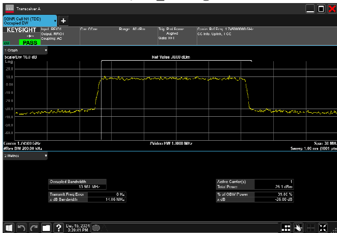
n66_15MHz_15kHz_1745MHz_DFT-s-OFDM 256 QAM_RB75@0
