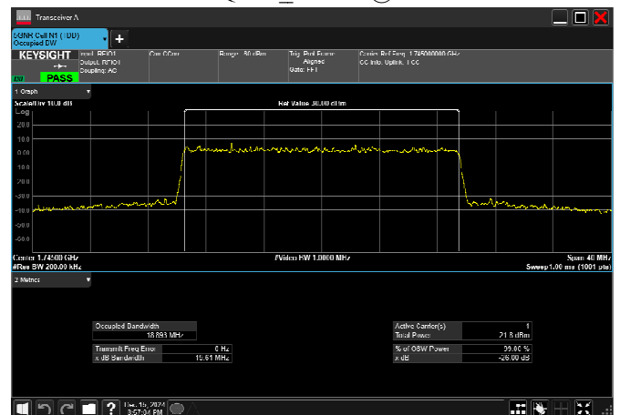
n66_20MHz_15kHz_1745MHz_CP-OFDM 256 QAM_RB106@0
