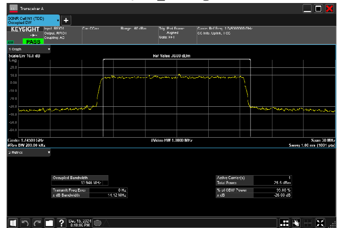
n66_15MHz_15kHz_1745MHz_CP-OFDM QPSK_RB79@0
