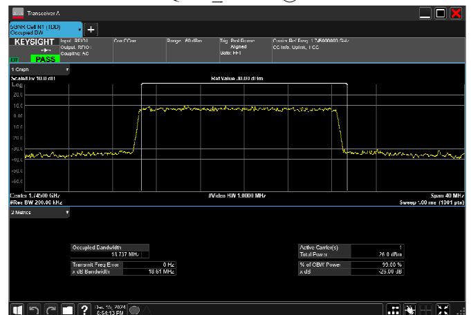
n66_20MHz_15kHz_1745MHz_DFT-s-OFDM 16 QAM_RB100@0
