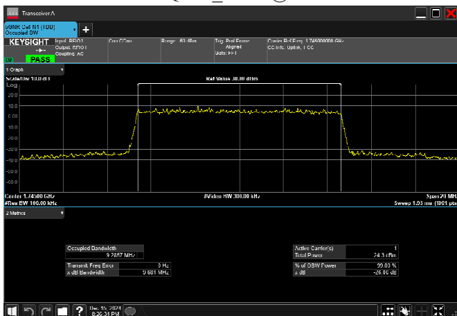
n66_10MHz_15kHz_1745MHz_CP-OFDM 64 QAM_RB52@0
