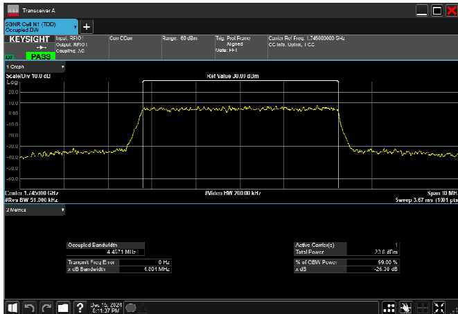
n66_5MHz_15kHz_1745MHz_CP-OFDM 256 QAM_RB25@0
