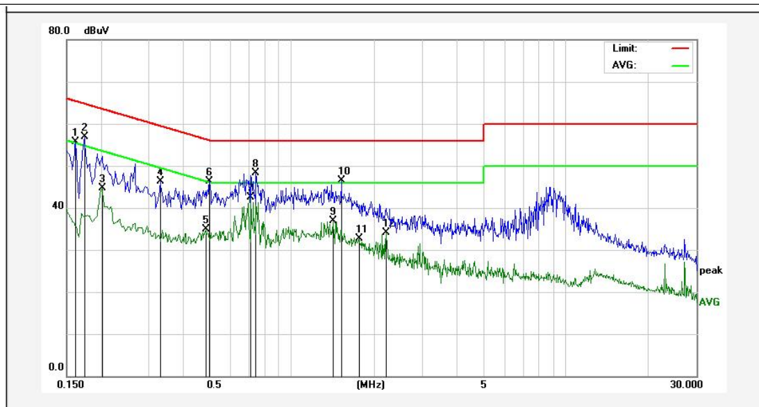
TM3 / Line: Neutral / Band: 2400-2483.5 MHz / BW: 20 / CH: L
